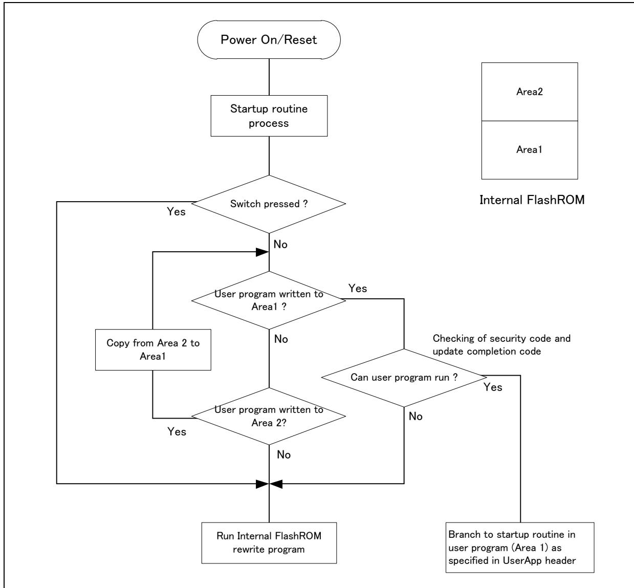
Figure 8-9 Power On / Reset Operation Flow (Using the backup function)
