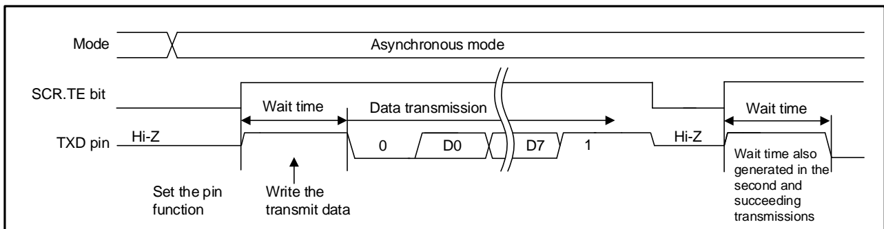
Figure 1.1 Internal Wait Time in Data Transmission
