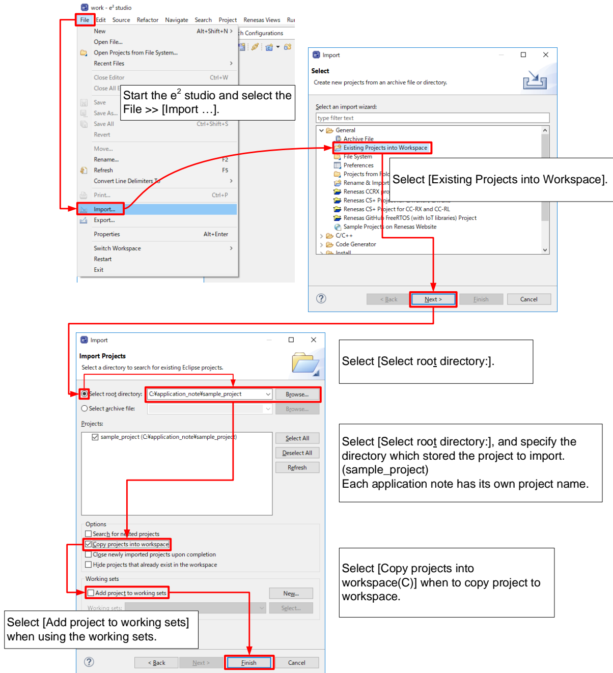
Figure 5.1 Importing a Project into e 2 studio
