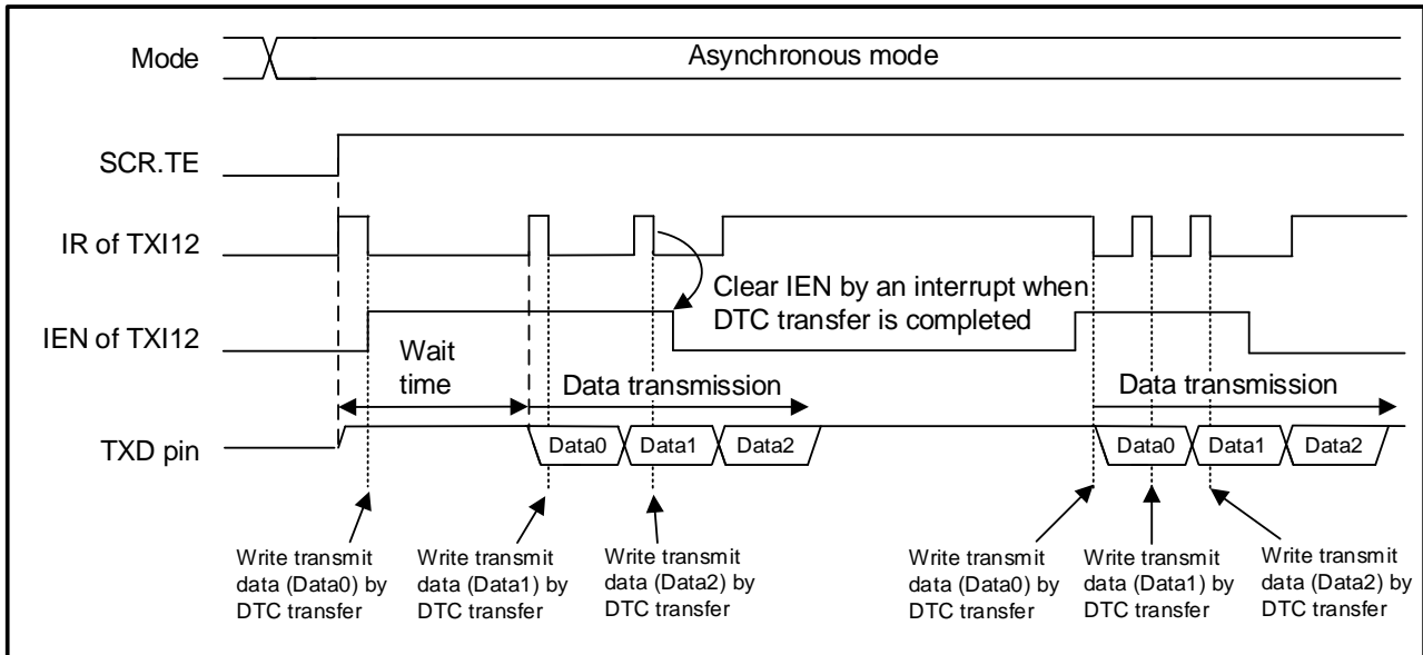
Figure 3.12 Timing Chart After Modification (Writing Transmit Data by DTC Transfer)
