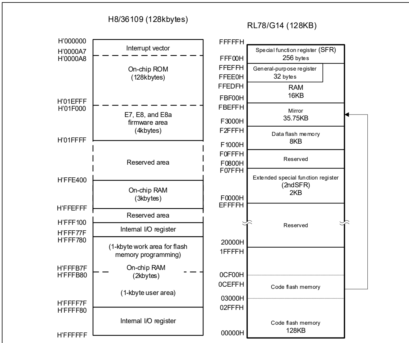
Figure 1.1 Memory maps of 128Kbyte flash memory for the H8/36109 and the RL78/G14
