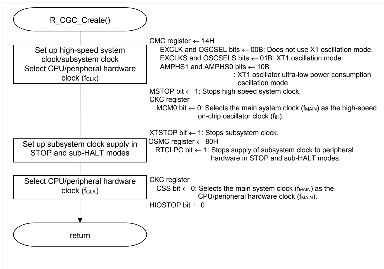
Figure 5.5 CPU Clock Setup
