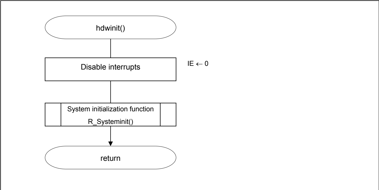
Figure 5.2 Initialization Function
