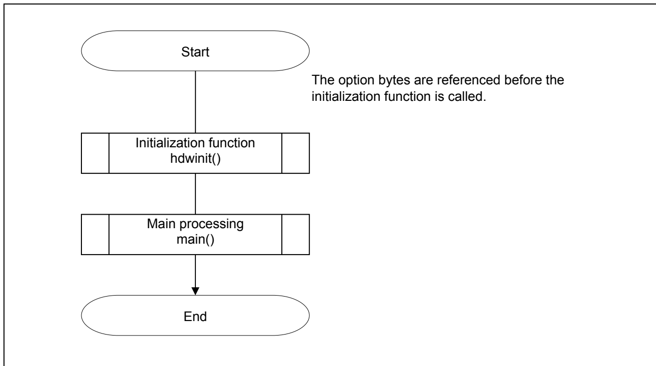
Figure 5.1 Overall Flow
