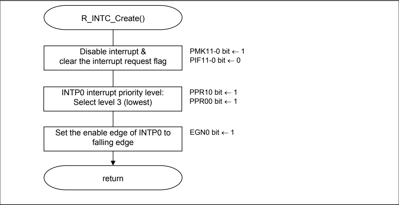
Figure 5.6 INTP0 Initialization
