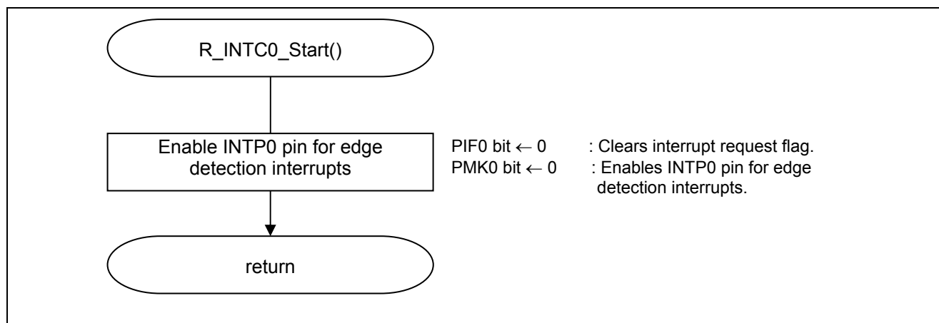
Figure 5.11 INTP0 Interrupt Enable Processing
