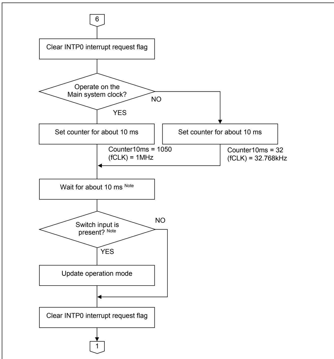
Figure 5.7 Main Processing (3/3)
