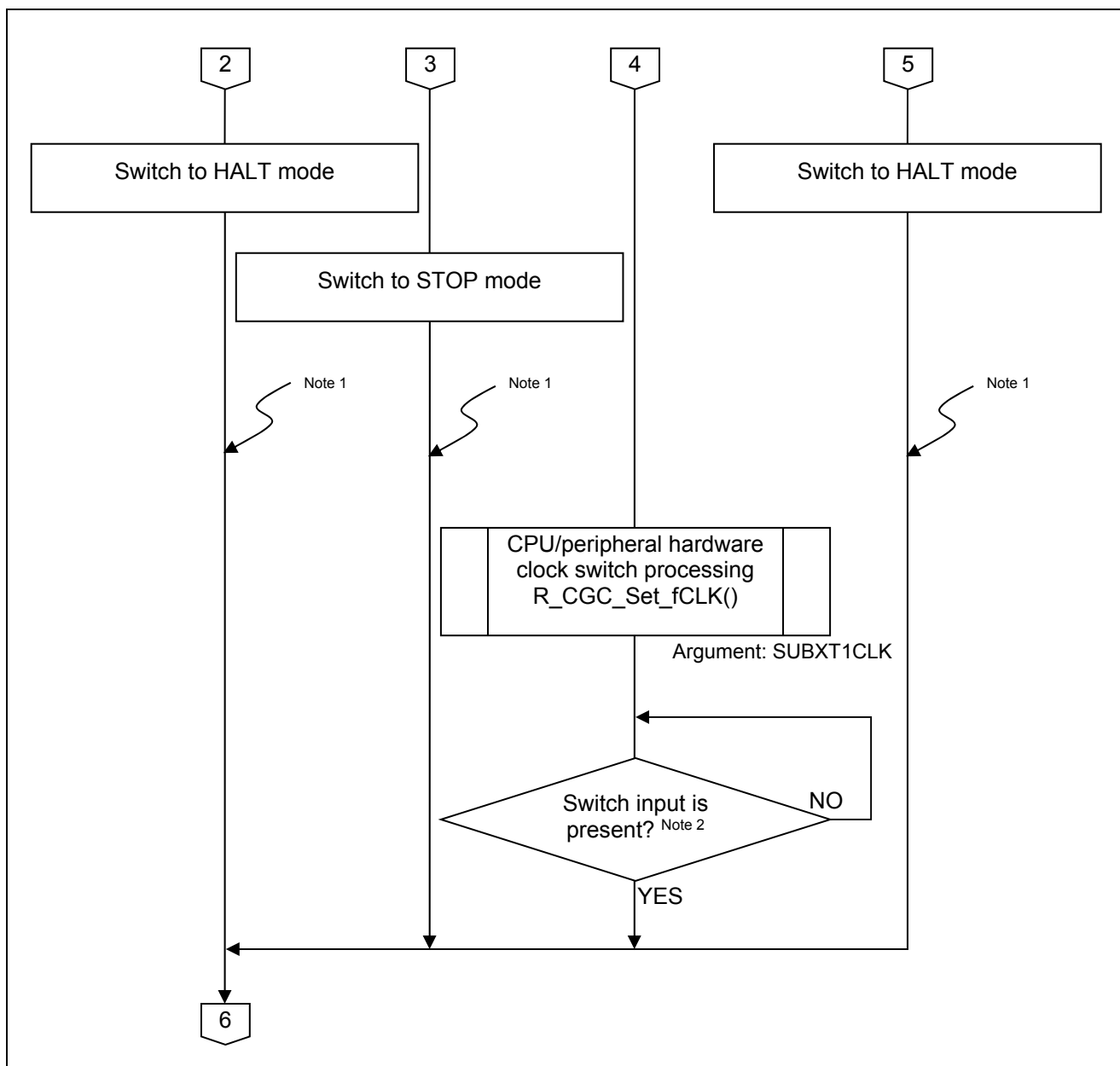
Figure 5.7 Main Processing (2/3)
