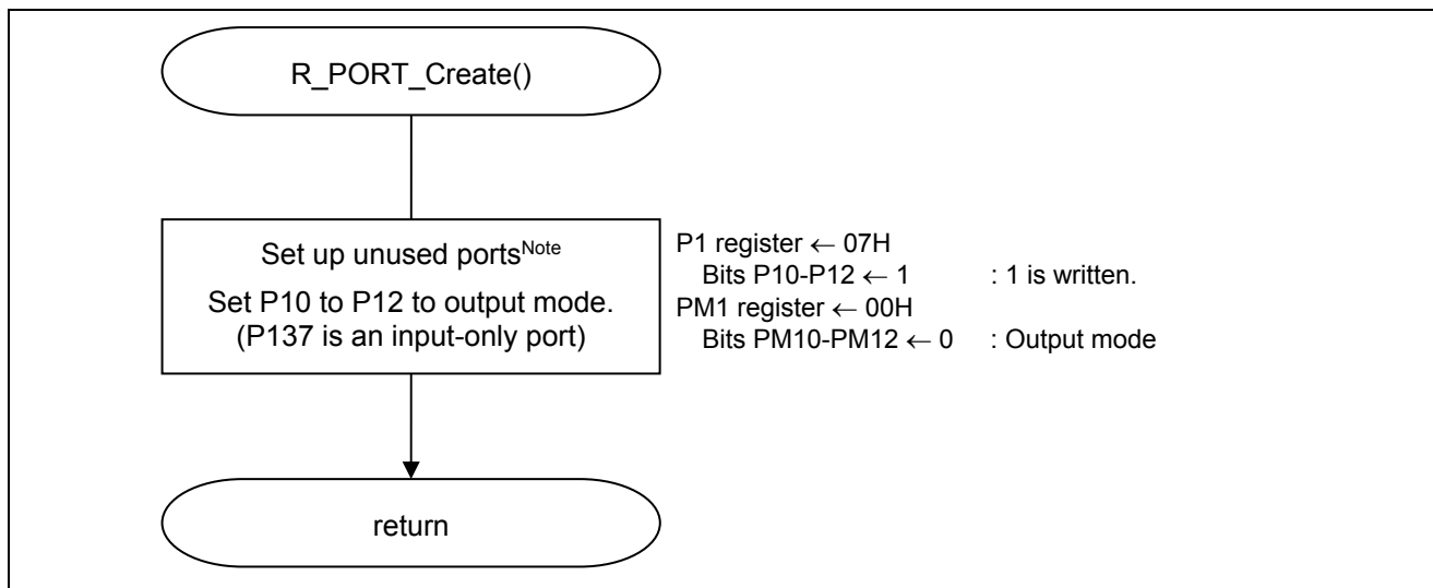
Figure 5.4 I/O Port Setup
