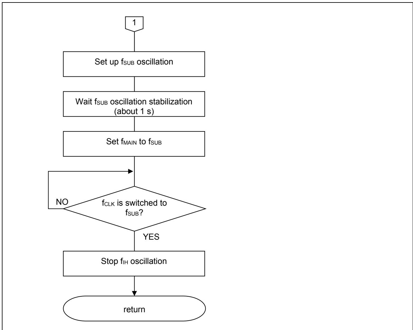
Figure 5.13 CPU/Peripheral Hardware Clock Switch Processing (2/2)
