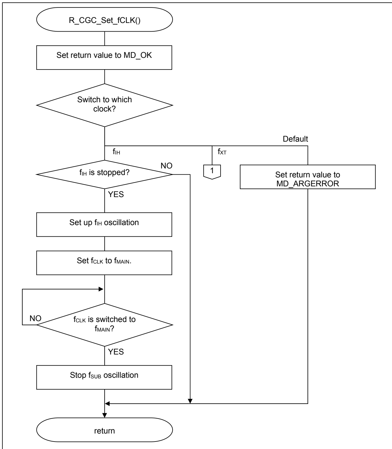
Figure 5.12 CPU/Peripheral Hardware Clock Switch Processing (1/2)
