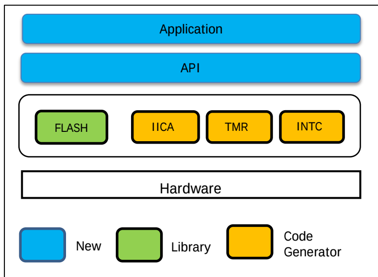
Figure 5.1 Software Structure
