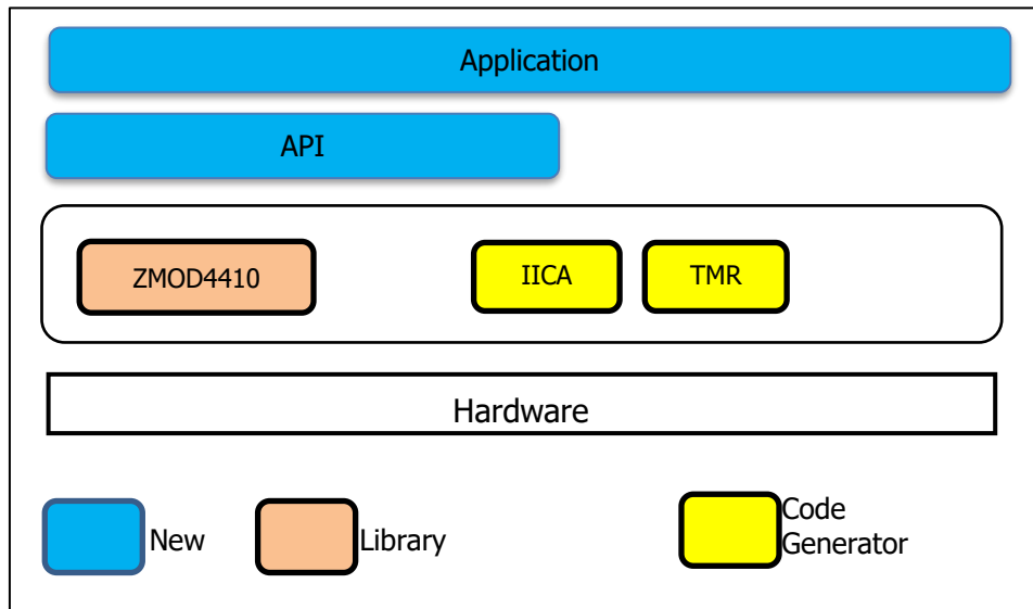
Figure 5.1 Software Structure
