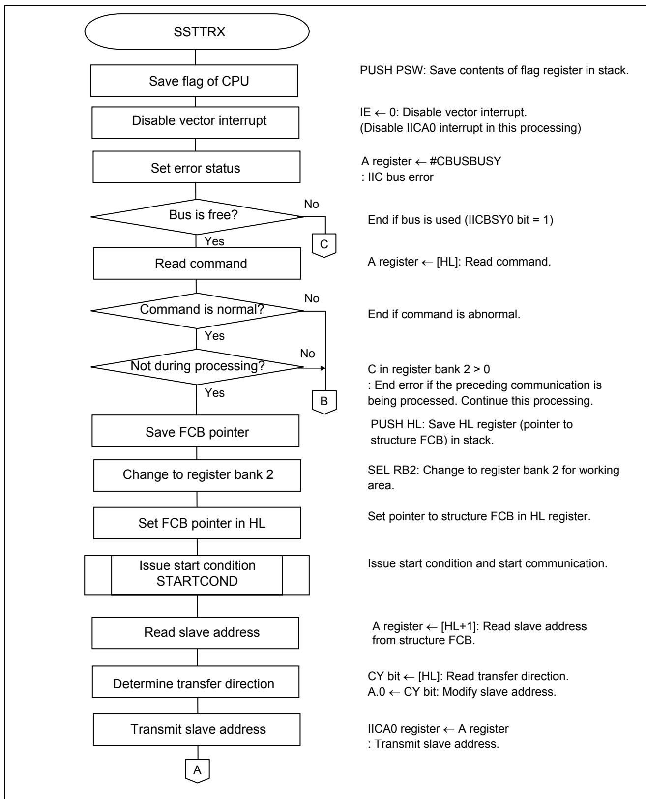
Figure 5.9 Master Transmission Start Processing (1/2)
