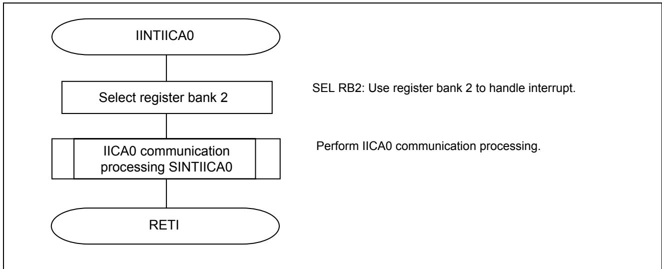
Figure 5.13 IICA0 Interrupt Processing
