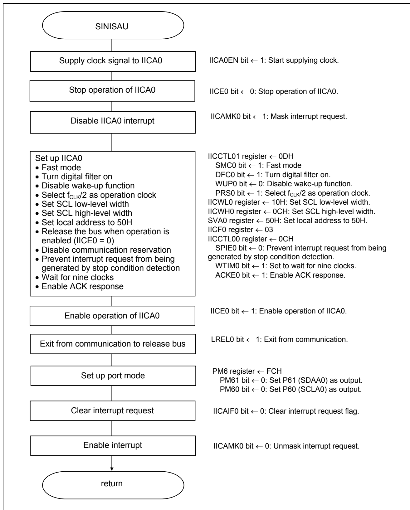
Figure 5.6 Serial Interface IICA Setup
