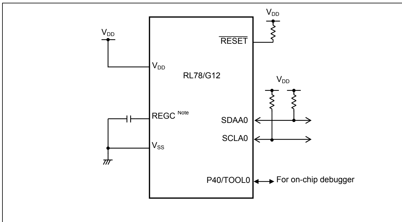
Figure 4.1 Hardware Configuration
