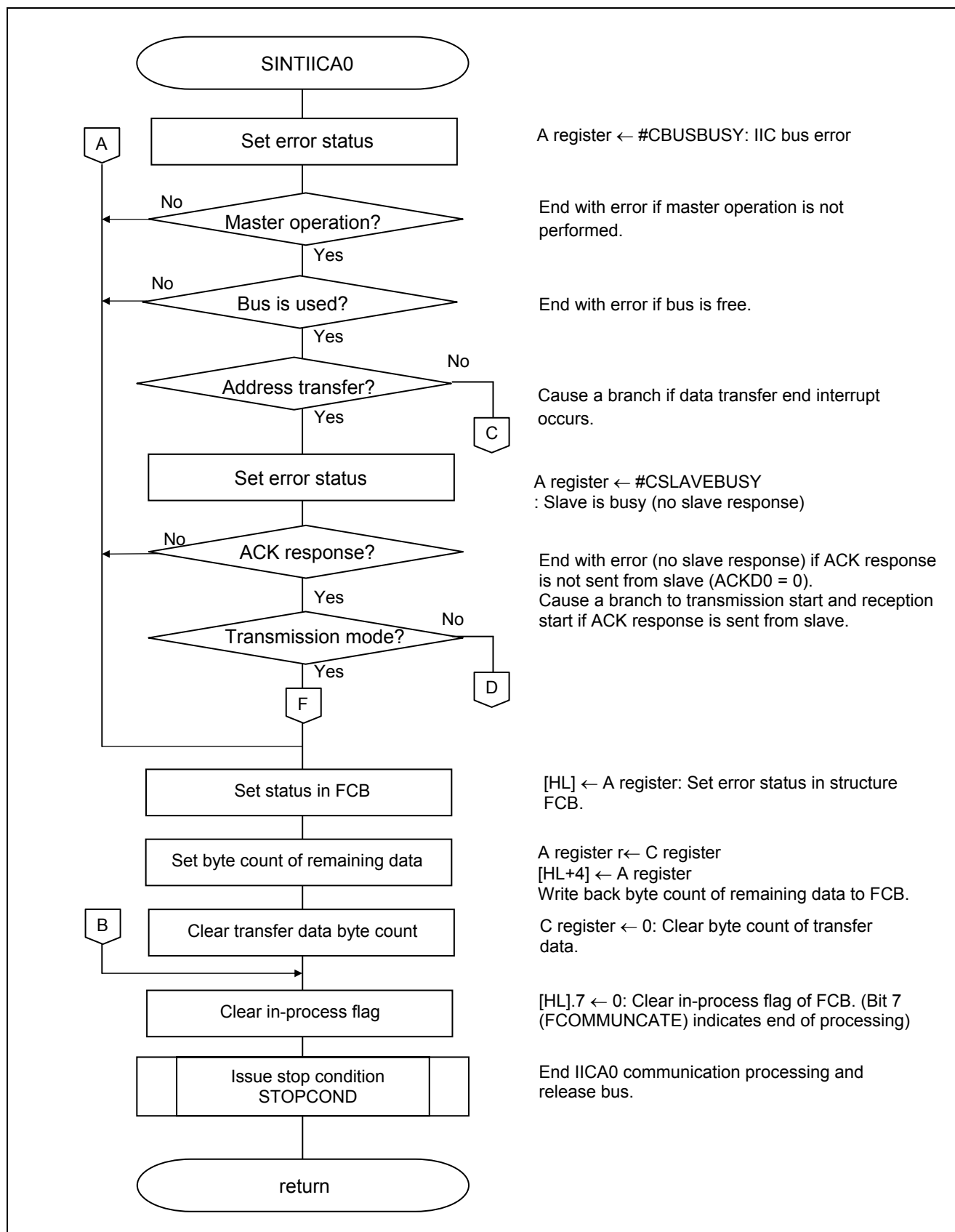
Figure 5.14 IICA0 Master Communication Processing (1/3)
