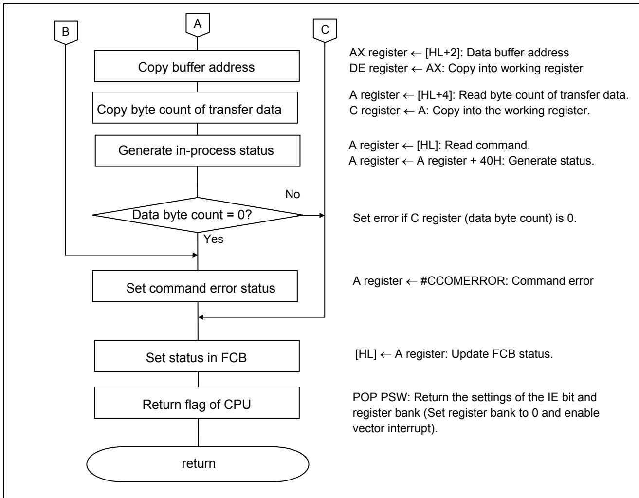
Figure 5.10 Master Transmission Start Processing (2/2)
