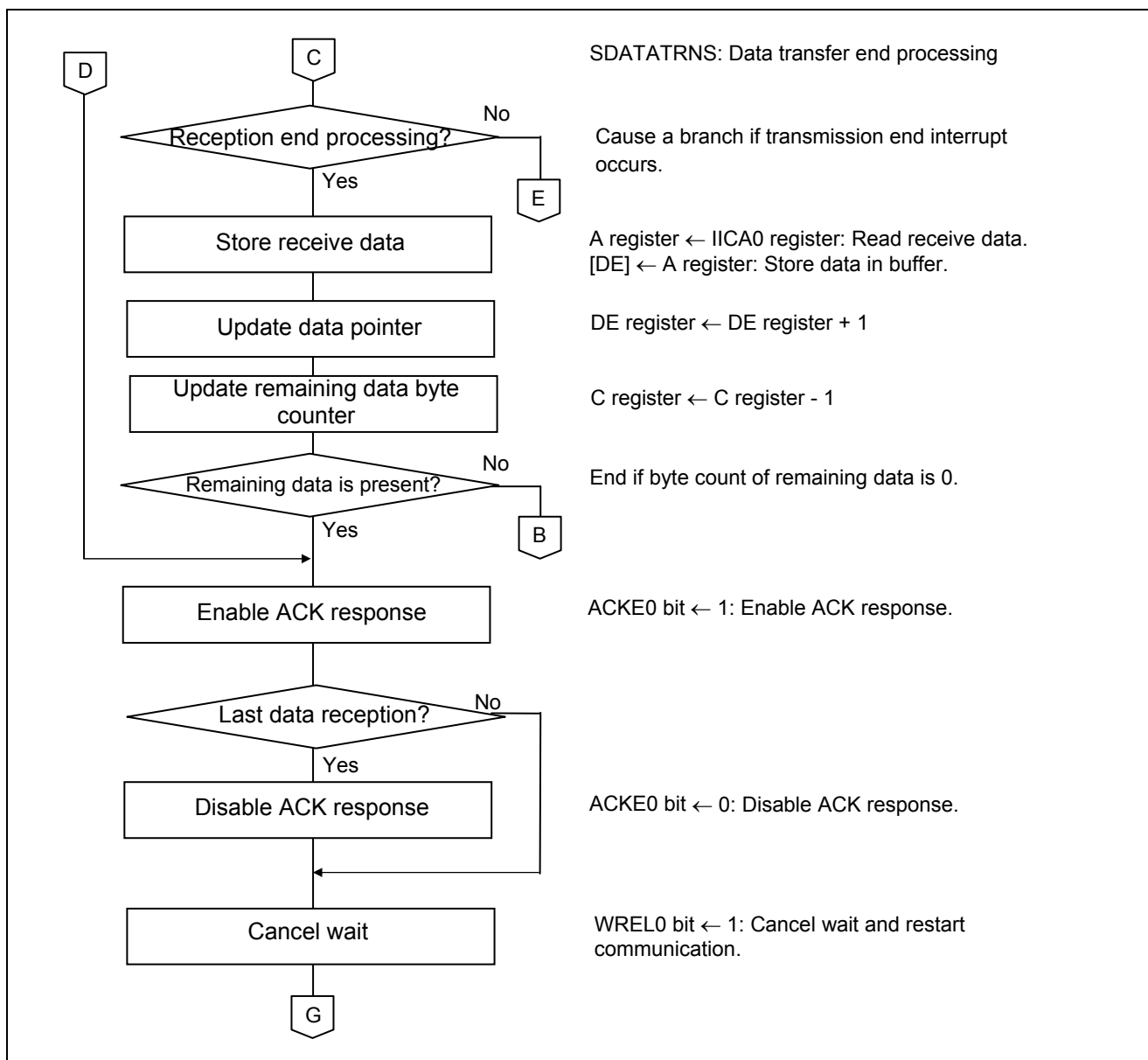
Figure 5.15 IICA0 Master Communication Processing (2/3)
