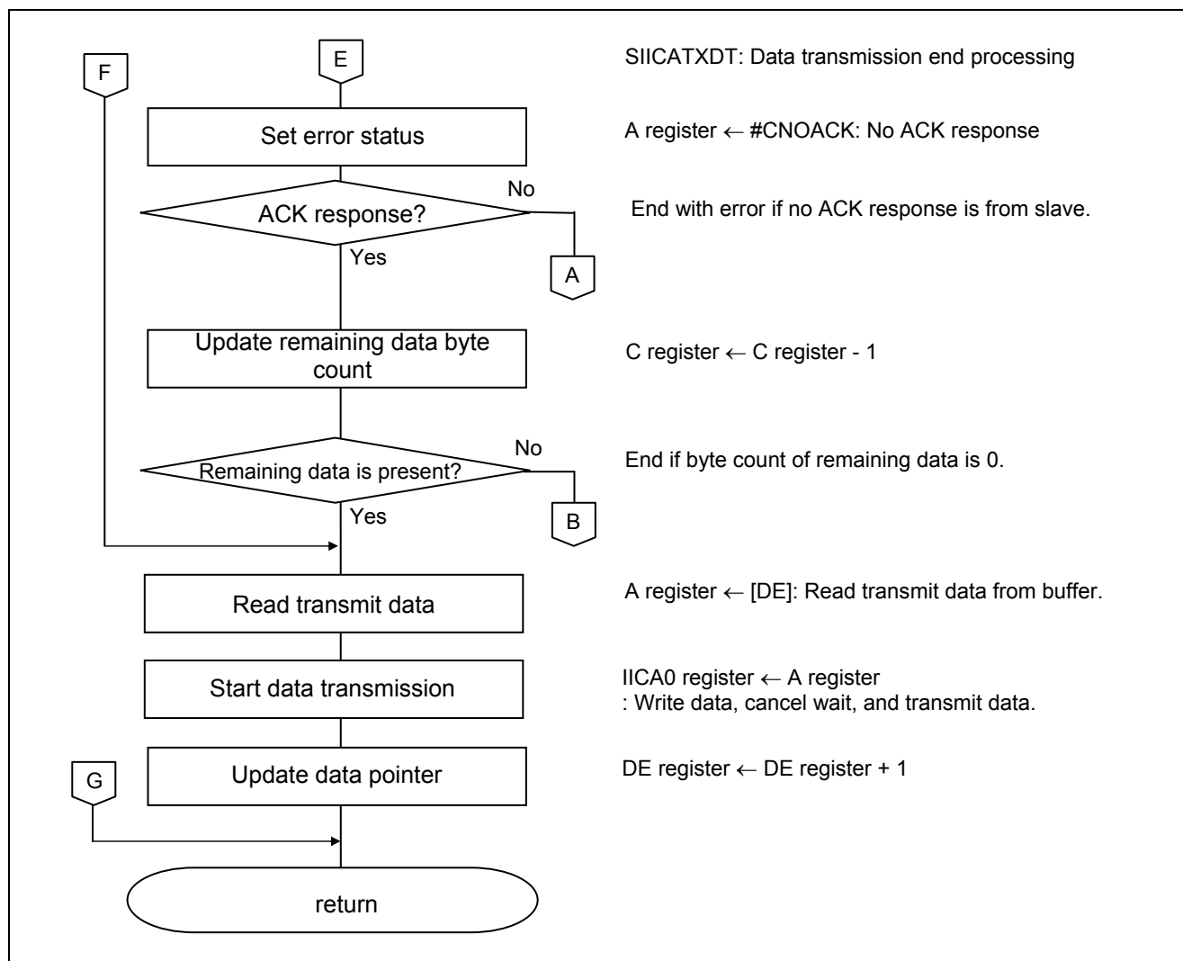
Figure 5.16 IICA0 Master Communication Processing (3/3)
