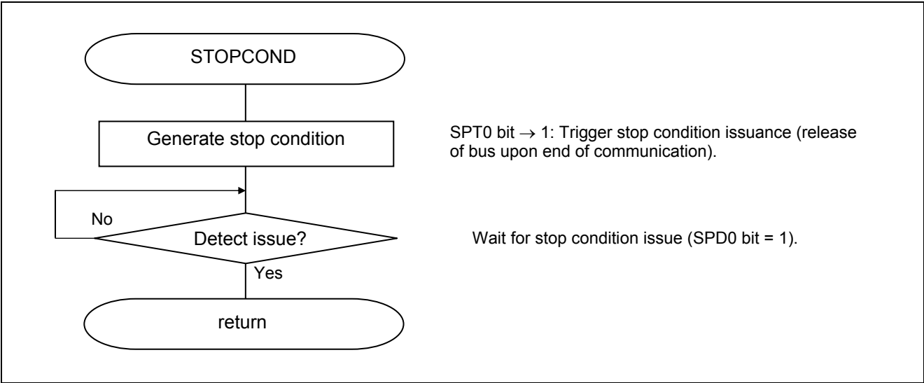
Figure 5.12 Stop Condition Issue
