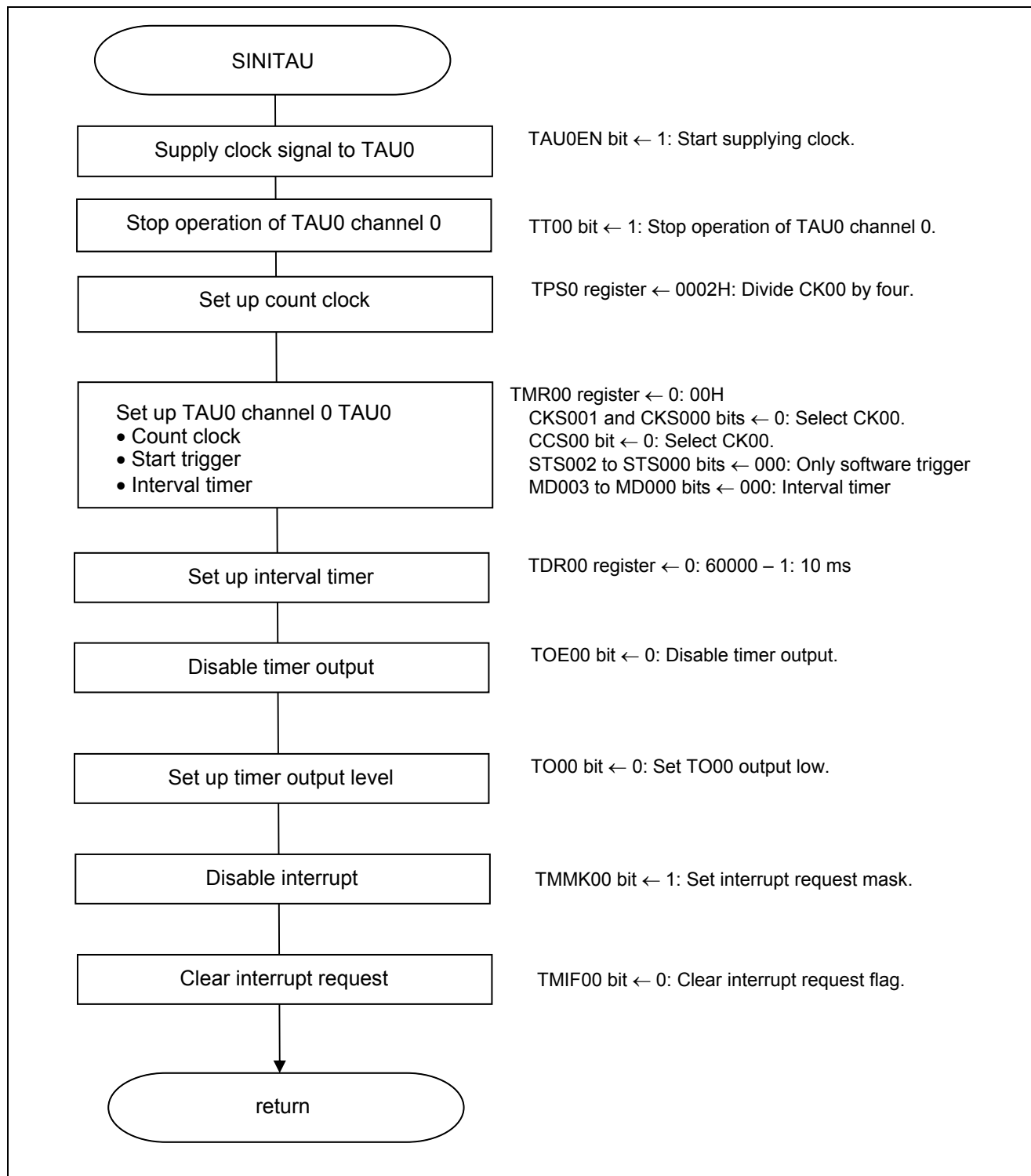
Figure 5.5 TAU0 Initial Setup
