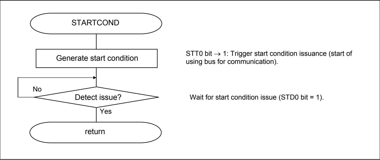
Figure 5.11 Start Condition Issue
