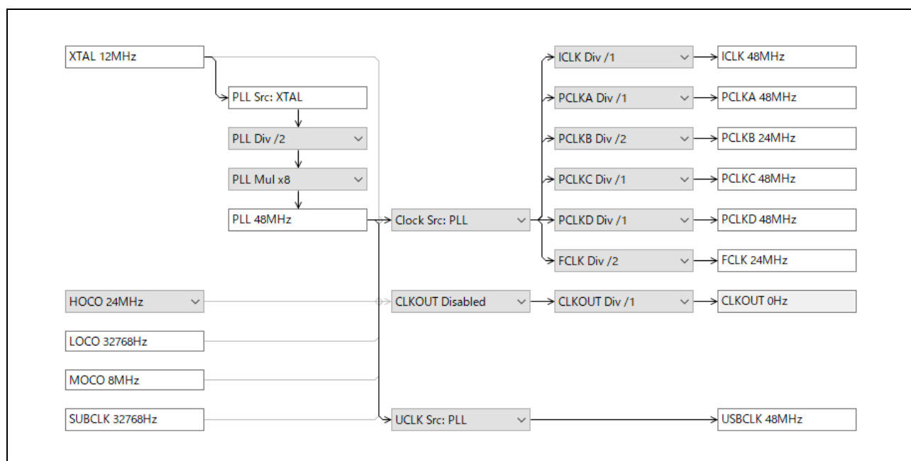
Figure 3.1 Clock Configuration
