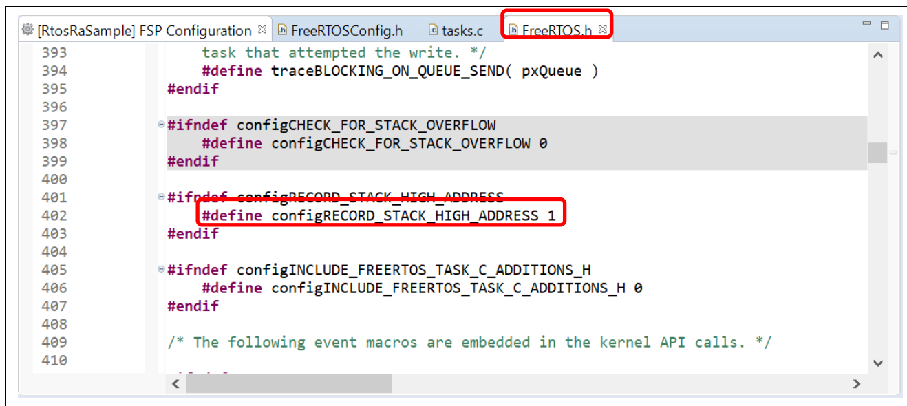
Figure 3-8. Define configRECORD_STACK_HIGH_ADDRESS in FreeRTOS.h
