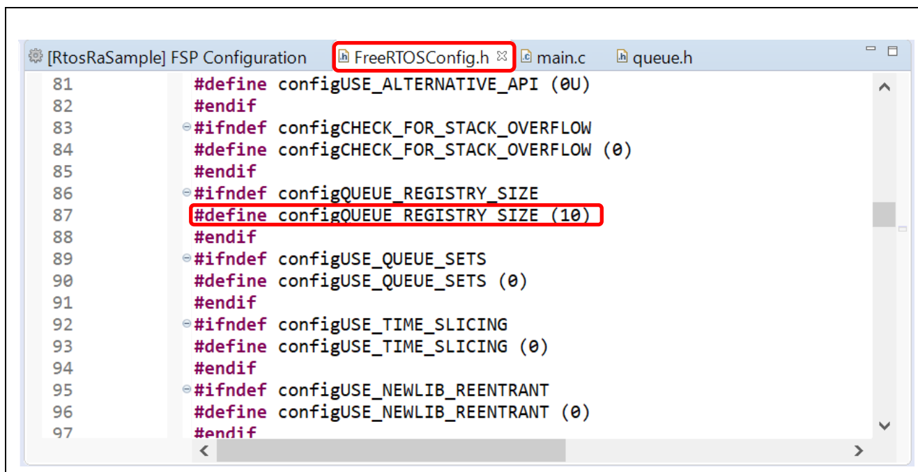
Figure 3-4. Define configQUEUE_REGISTRY_SIZE in FreeRTOSConfig.h
