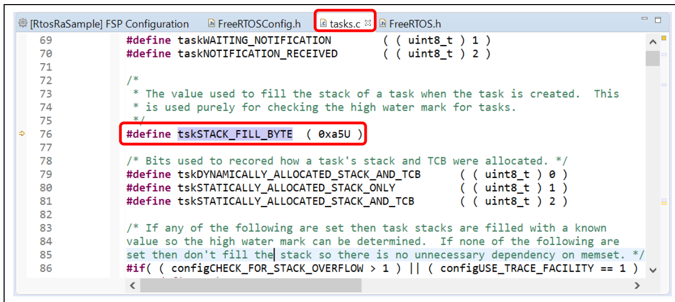
Figure 3-9. Define tskSTACK_FILL_BYTE in task.c
