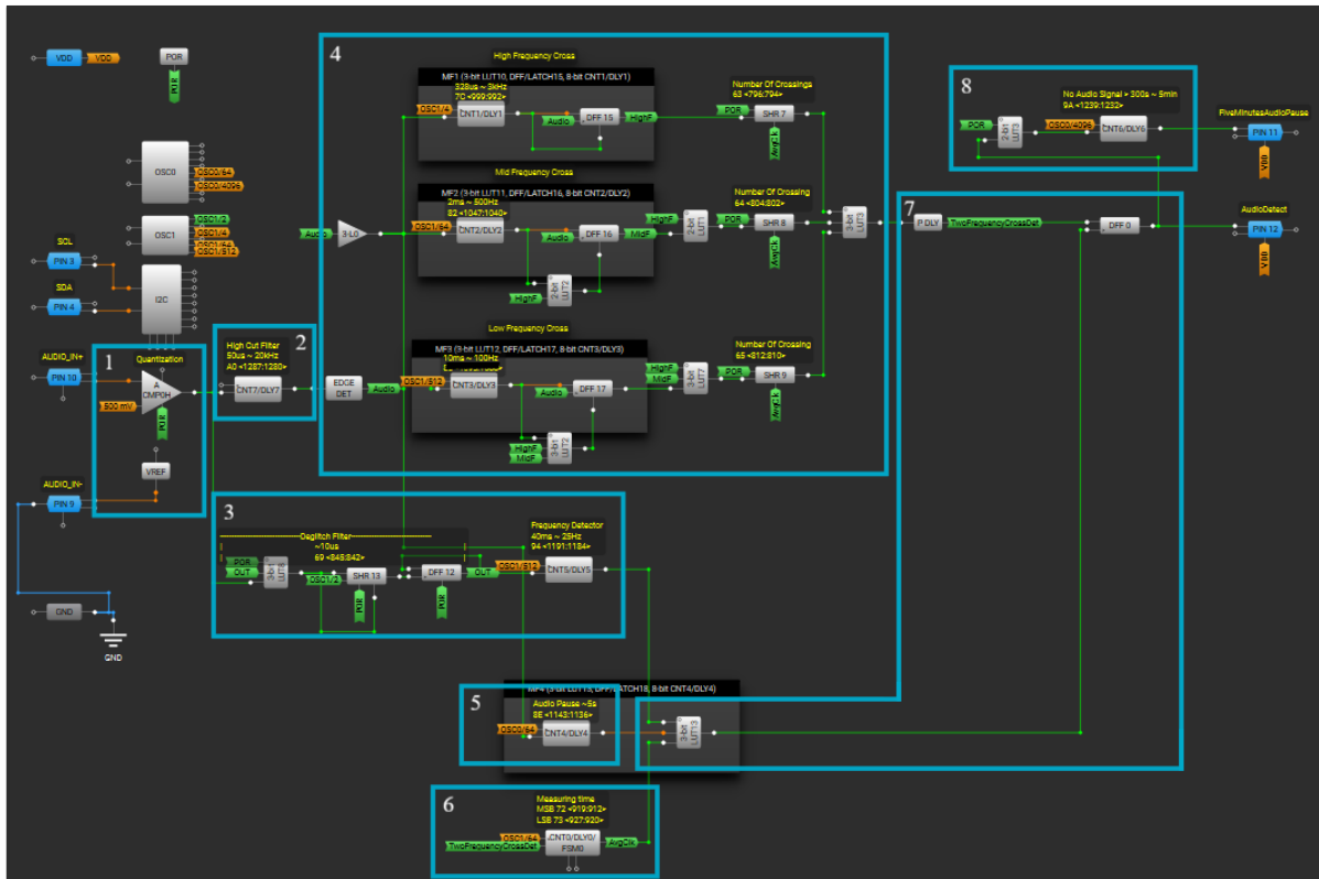
Figure 2: Design Architecture
