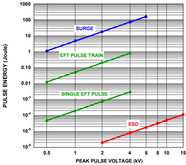
FIGURE 10. COMPARISON OF PULSE ENERGIES FOR VARIOUS TRANSIENT IMMUNITY TESTS
