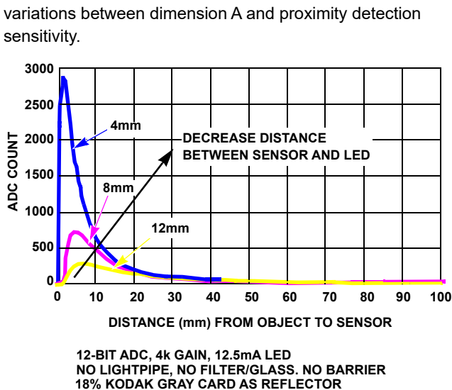
FIGURE 7. PROXIMITY SENSOR OUTPUT VARYING THE DISTANCE BETWEEN THE SENSOR AND LED
