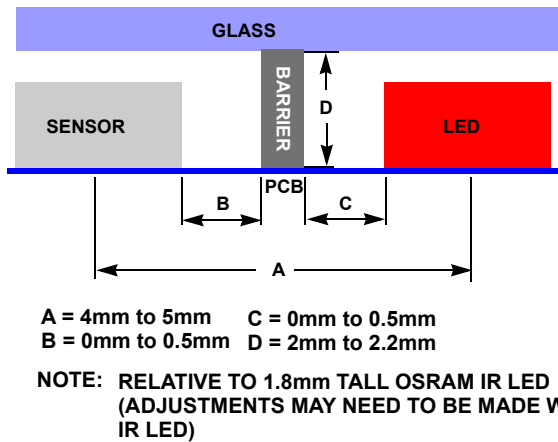
FIGURE 5. TYPICAL MECHANICAL DESIGN DIMENSIONS
