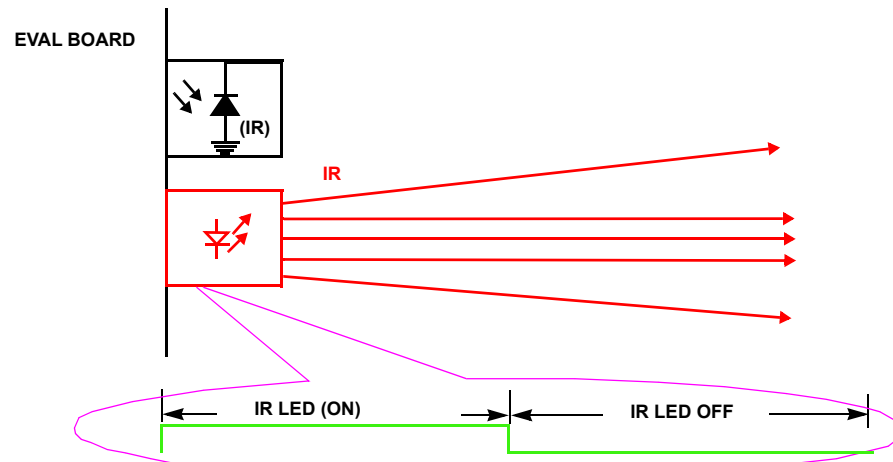
FIGURE 4A. NO SENSING OBJECT IN PROXIMITY DETECTION AREA
