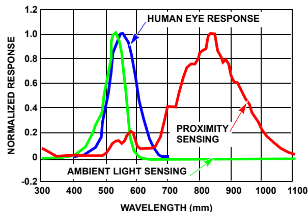
FIGURE 1. SPECTRAL RESPONSE OF AMBIENT LIGHT SENSOR AND PROXIMITY SENSOR
