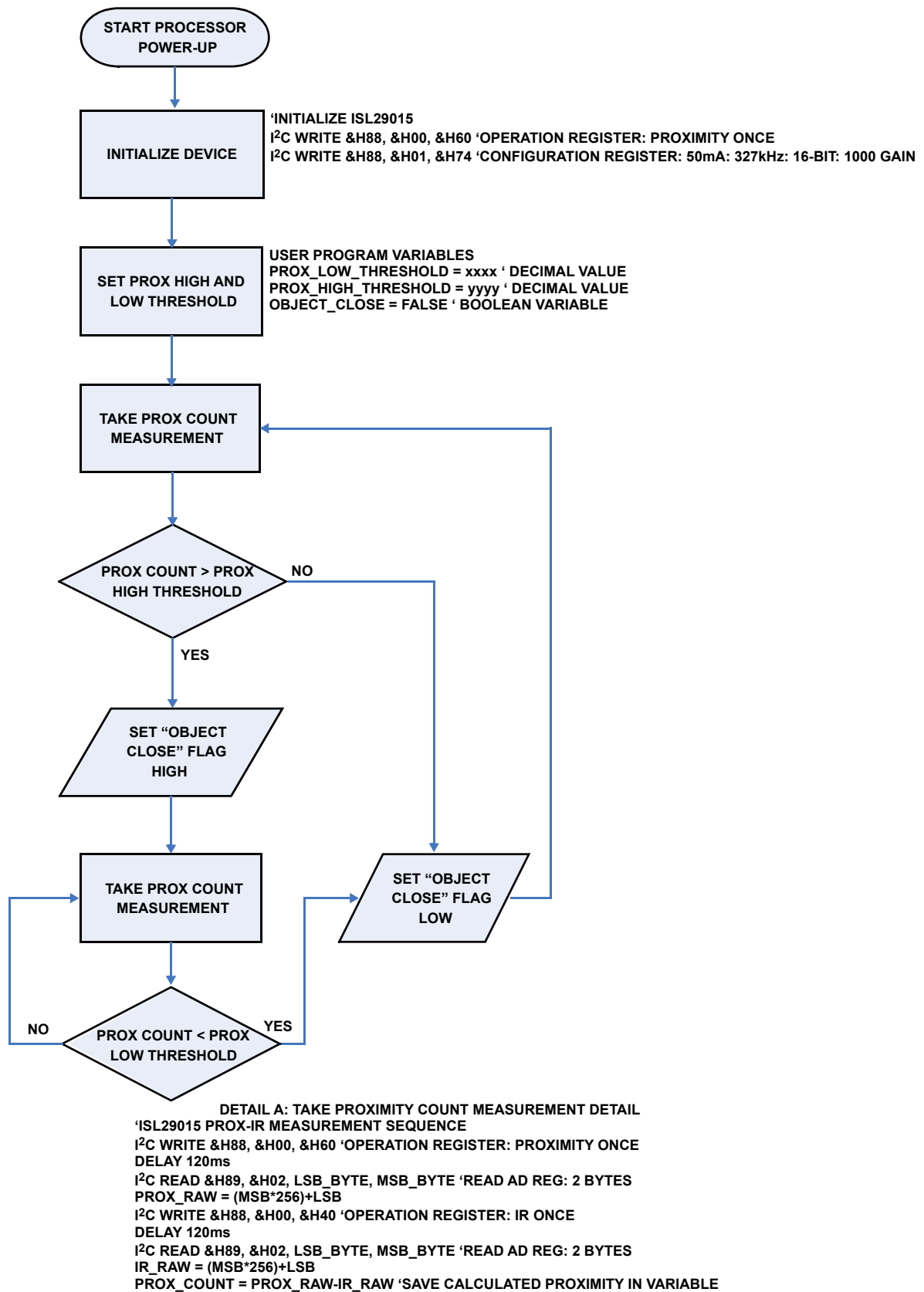
FIGURE 22. FLOW-CHART FOR PROXIMITY SYSTEM DETECTING HUMAN SKIN
