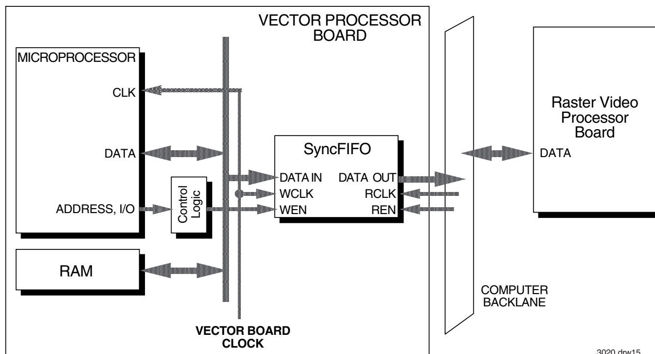
Figure 15. A Graphics System Using the SyncFIFO
