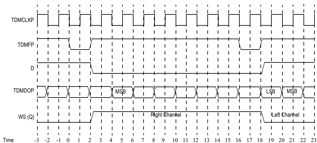
Figure 5 TDM to I 2 S Timing Waveform
