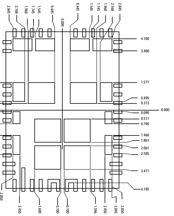
STENCIL PATTERN WITH 23 MOSLP TOP VIEW
