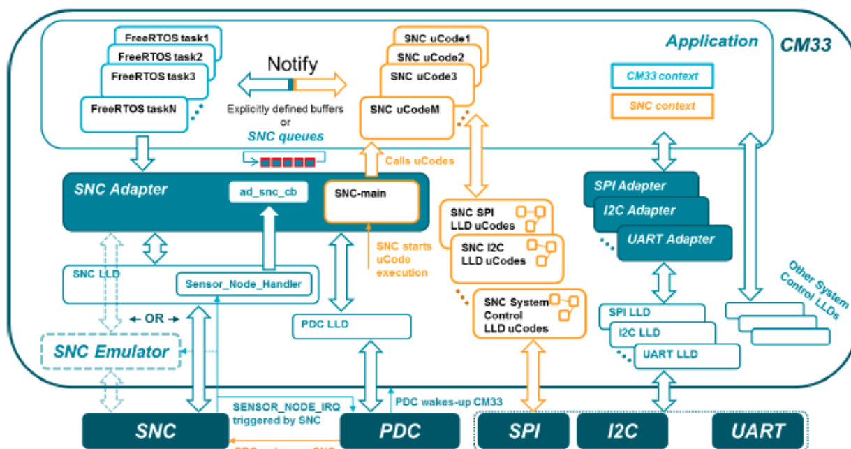
Figure 4: Block diagram of SNC programming framework
