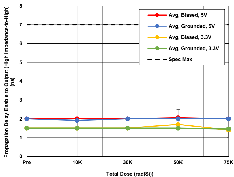
Figure 15. ISL71710SLHM average propagation delay, enable to output, high impedance-to-high ( t_{PZH} ) with V_{DD1} = V_{DD2} = 3.3V and 5V , C_L = 15pF as a function of LDR irradiation. The error bars, if visible, represent the minimum and maximum measured values. The datasheet limit is 7ns maximum.
