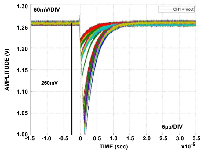
FIGURE 14. COMPOSITE SET PLOT FOR ISL71090SEH12 AT LET 58 V_{IN} = 30V , I_{OUT} = 20mA , C_{OUT} = 0.1\mu F , C_{COMP} = 1nF . THE SCOPE CAPTURE WAS TRUNCATED AT 1.0V
