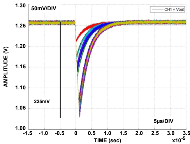
FIGURE 13. COMPOSITE SET PLOT FOR ISL71090SEH12 AT LET 58 V_{IN} = 4V , I_{OUT} = 20mA , C_{OUT} = 0.1\mu F , C_{COMP} = 1nF
