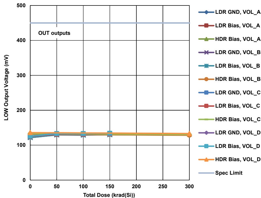
Figure 6. HS-26C31EH output LOW voltage, OUT outputs, channels A through D, as a function of biased HDR total dose irradiation to 300krad(Si) and biased and unbiased (grounded) LDR irradiation to 150krad(Si). The sample size for the HDR cell was 48, while the sample sizes for the LDR cells were 20 each. The SMD limit is 500mV maximum; the internal ATE limit (shown) is 450mV maximum.
