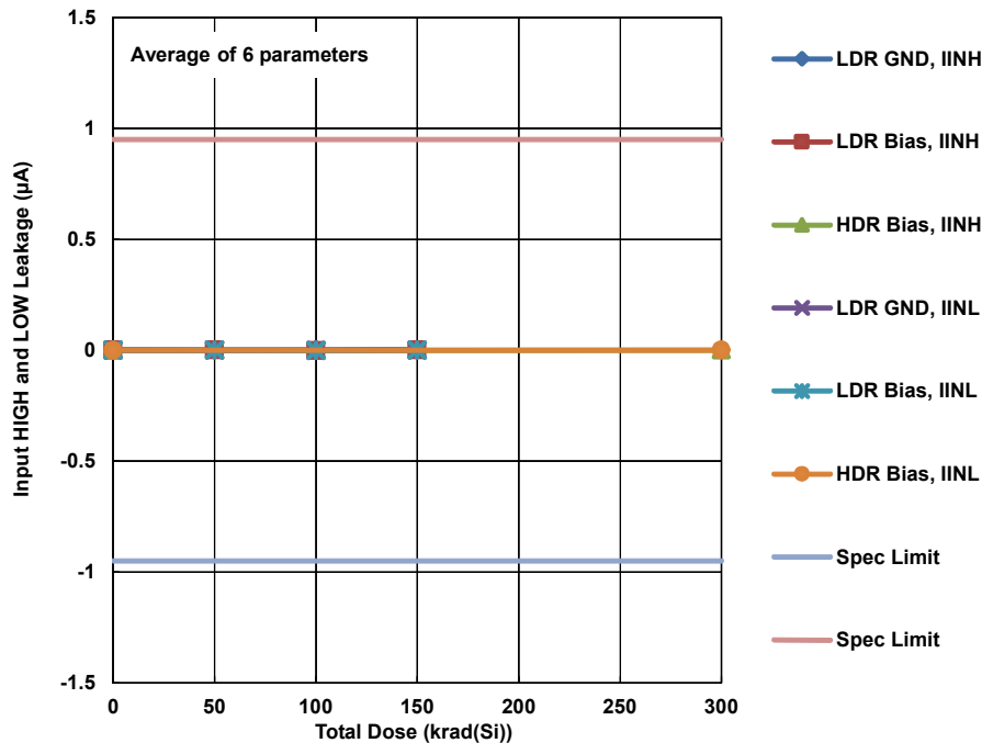
Figure 10. HS-26C31EH input HIGH and LOW leakage, average of channels A through D, ENABLE and ENABLE_BAR, as a function of biased HDR total dose irradiation to 300krad(Si) and biased and unbiased (grounded) LDR irradiation to 150krad(Si). The sample size for the HDR cell was 48, while the sample sizes for the LDR cells were 20 each. The SMD limits are -1.0µA to +1.0µA; the internal ATE limits (shown) are -0.95µA to +0.95µA.
