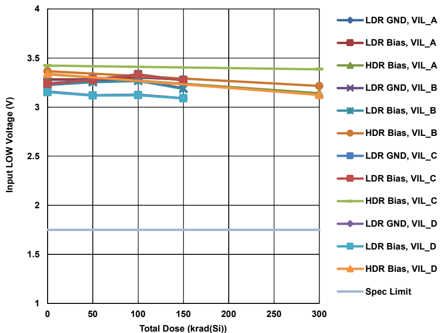
Figure 12. HS-26C31EH input LOW voltage, channels A through D, as a function of biased HDR total dose irradiation to 300krad(Si) and biased and unbiased (grounded) LDR irradiation to 150krad(Si). The sample size for the HDR cell was 48, while the sample sizes for the LDR cells were 20 each. The SMD limit is 1.75V minimum.
