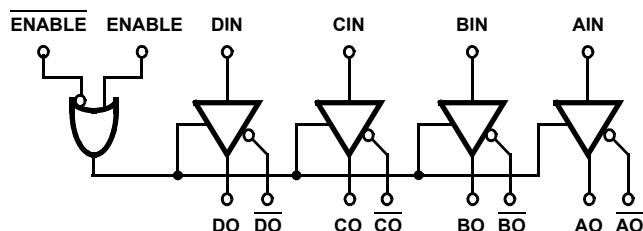
Figure 1. HS-26C31EH Block Diagram
