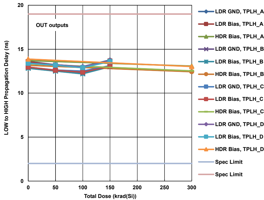
Figure 14. HS-26C31EH LOW to HIGH propagation delay, OUT outputs, channels A through D, as a function of biased HDR total dose irradiation to 300krad(Si) and biased and unbiased (grounded) LDR irradiation to 150krad(Si). The sample size for the HDR cell was 48, while the sample sizes for the LDR cells were 20 each. The SMD limits are 2ns to 22ns; the internal ATE limits (shown) are 2ns to 19ns.
