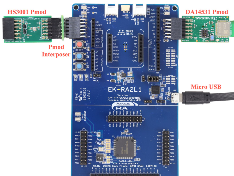
Figure 1. Hardware Components
