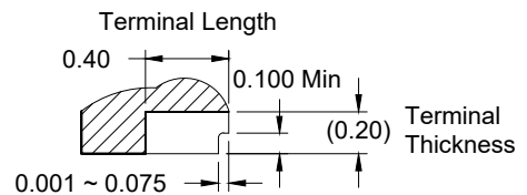
DETAIL A (HALF CUT)
