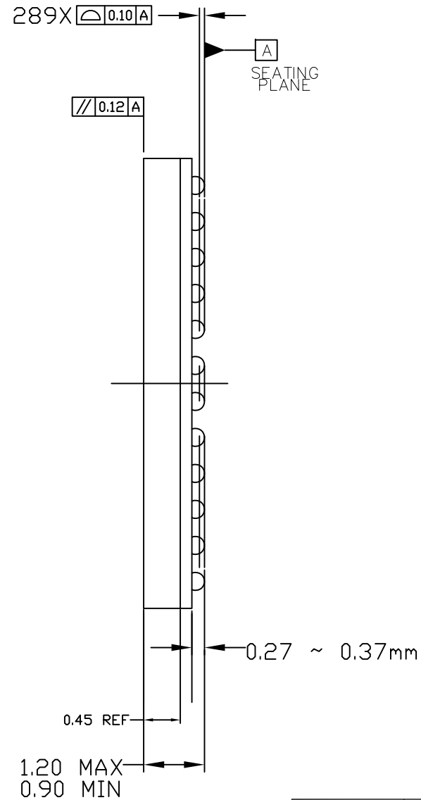
SIDE VIEW
