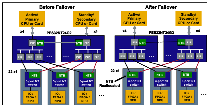
Figure 5 Dual-Star Topology
