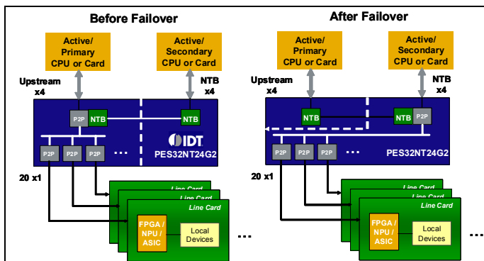
Figure 4 Dual-Host Failover System
