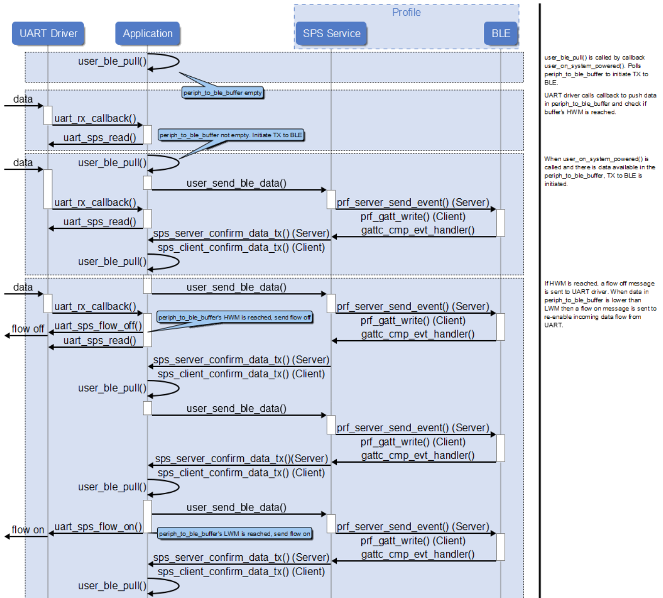
Figure 6: UART to BLE data transfer sequence diagram
