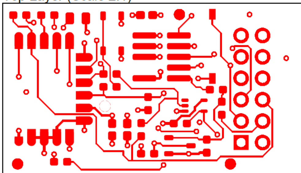
Figure 17. Copper Top
