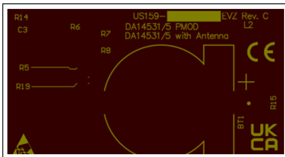
Figure 21. Silkscreen Bottom
