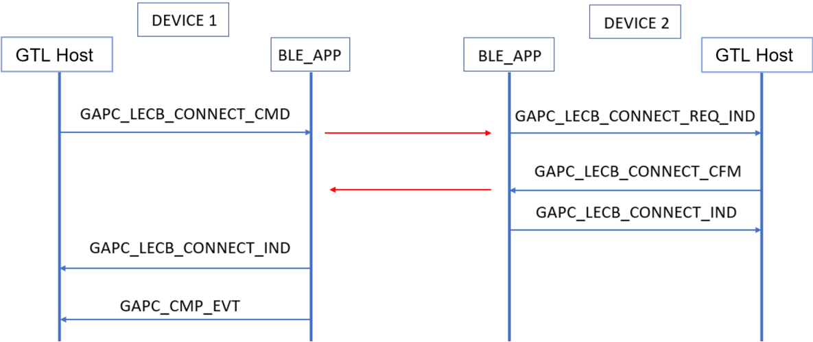
Figure 31. LECB connection procedure
