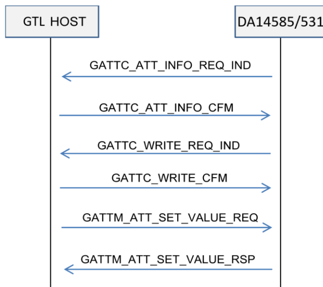
Figure 16. Peer writing attribute values using a prepare write request
