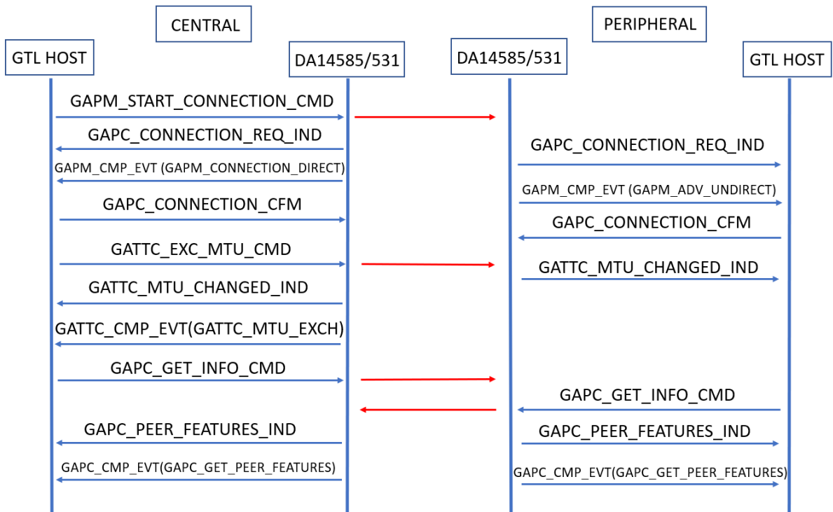
Figure 8. Connection sequence example
