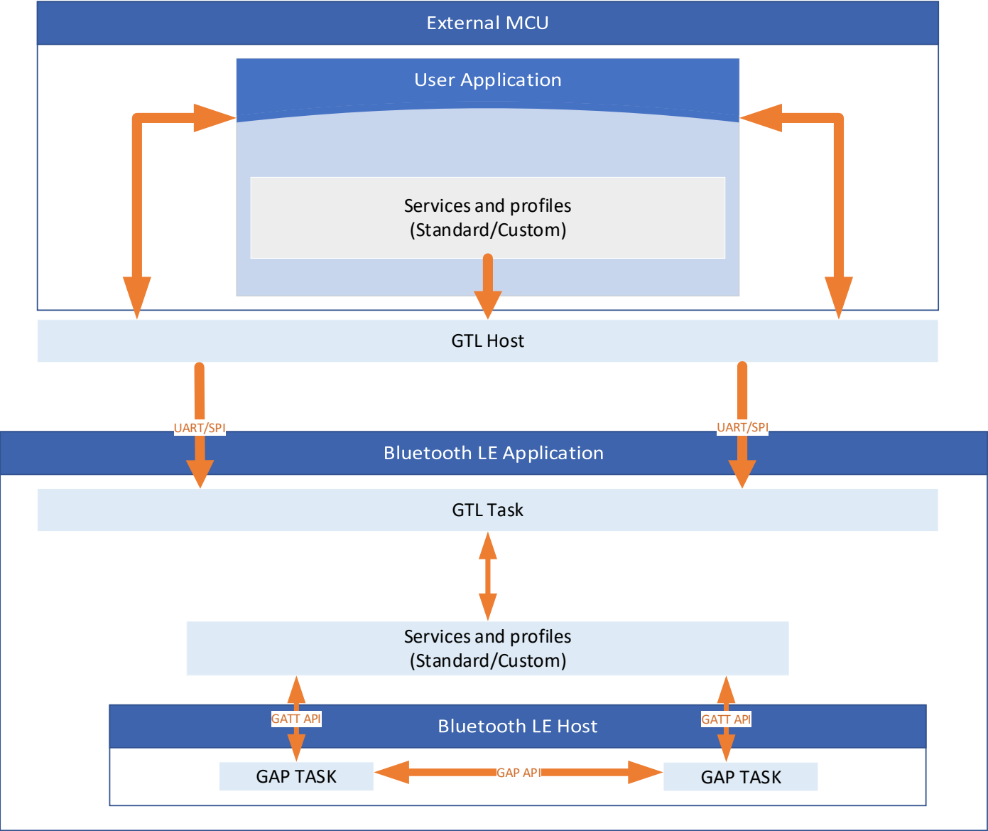
Figure 2. DA1453x/DA1458x GTL project software architecture
