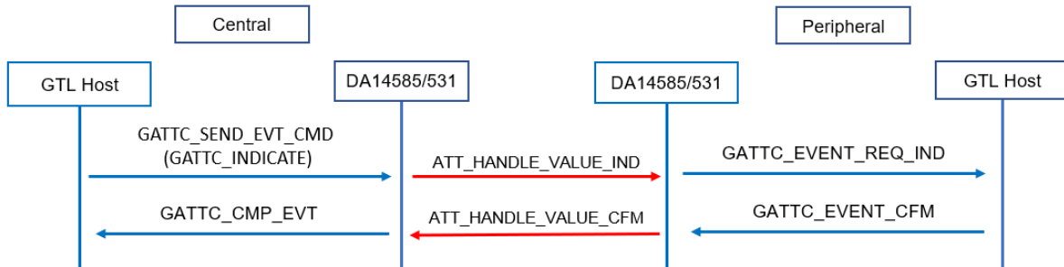
Figure 18. GATTC_SEND_EVT_CMD with an indication
