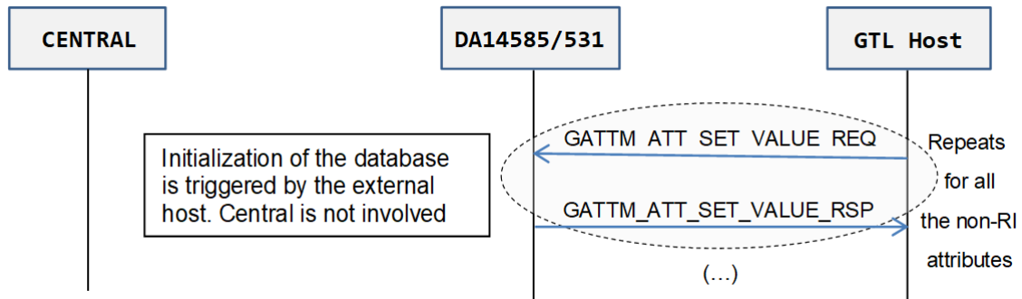
Figure 14. Database value initialization
