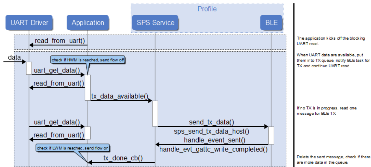
Figure 5 UART to BLE Data Transfer Sequence Diagram
