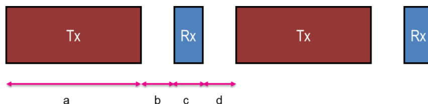
Figure 14 DLE Packet Timing
