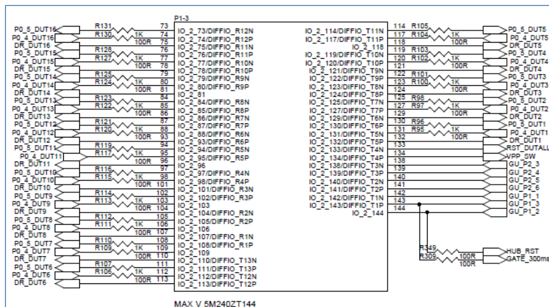
Figure 149: CPLD DUT UART Connections
