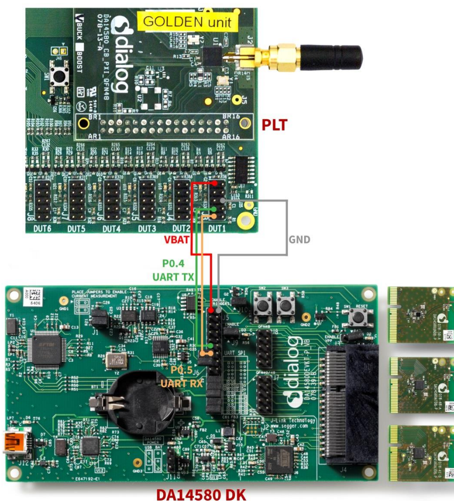
Figure 175: DA14580/5 Pro Motherboard DK Wiring.
