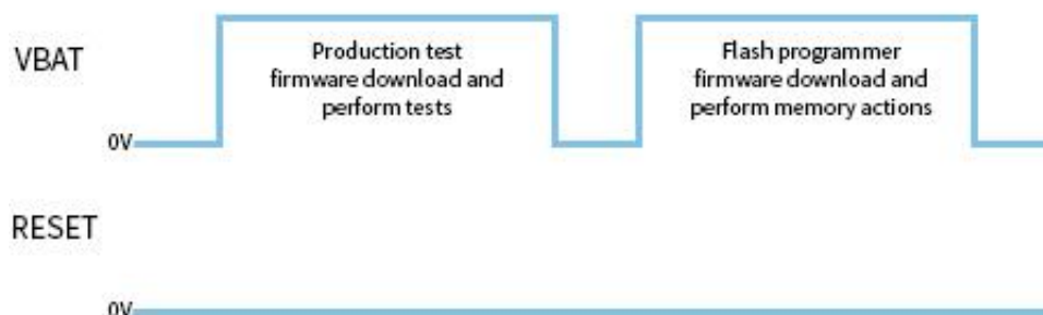
Figure 24: VBAT only
