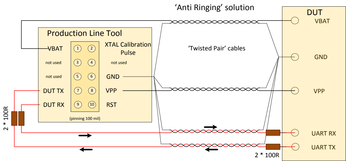
Figure 171: Anti-Ringing Solution
