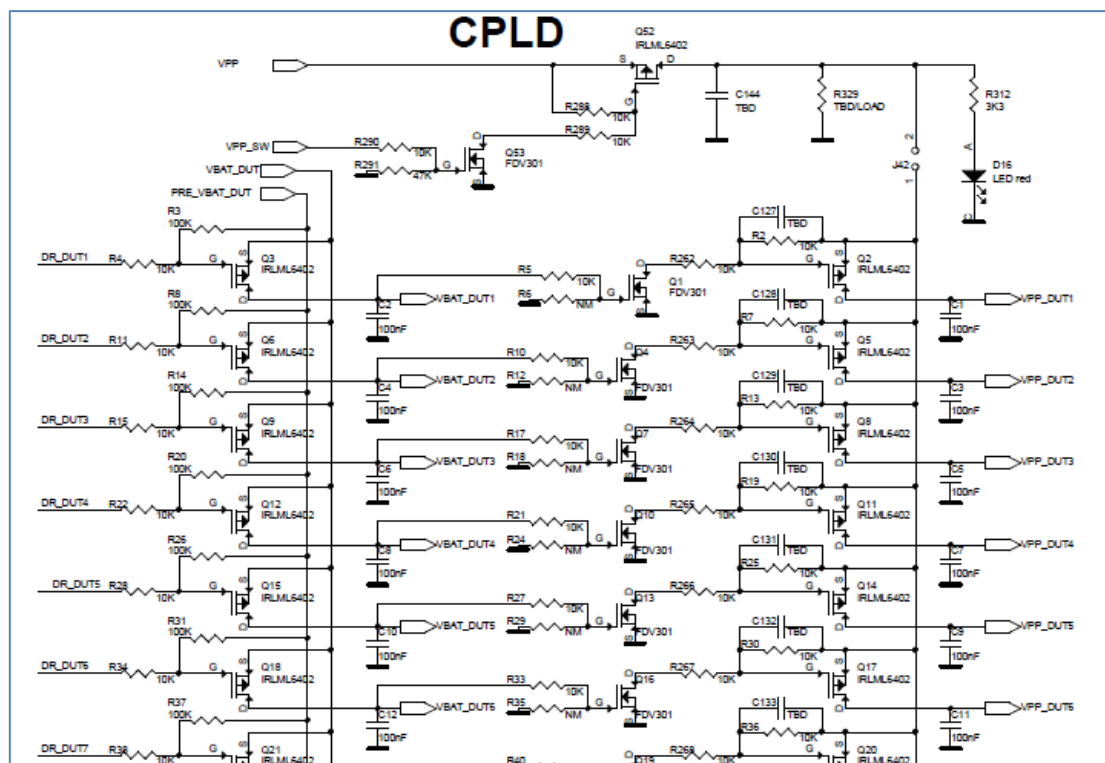
Figure 148: VBAT and VPP Control from CPLD
