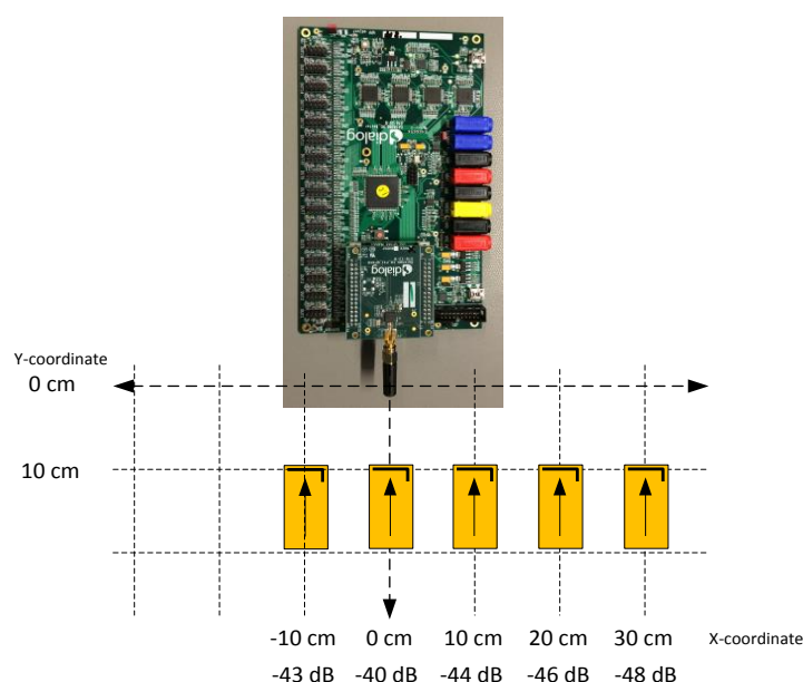
Figure 163: Example Locations and RSSI Readouts of Horizontal Antenna
