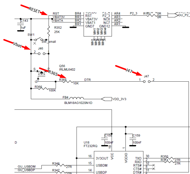
Figure 160: R365, J47 and RESET Shown in Electrical Schematic
