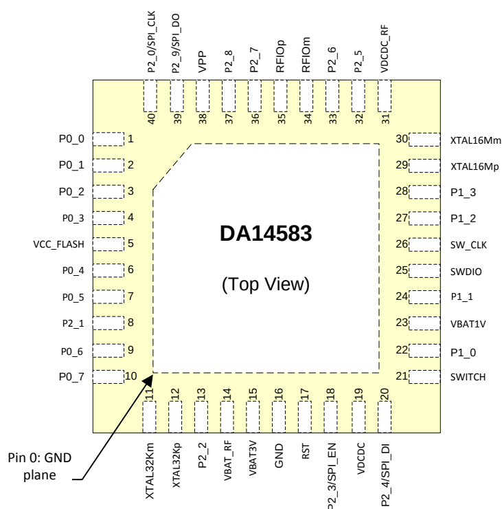
Figure 172: Pin Assignment of DA14583 – QFN40
