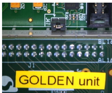
Figure 158: Jumper J47 Added Next to Golden Unit Socket
