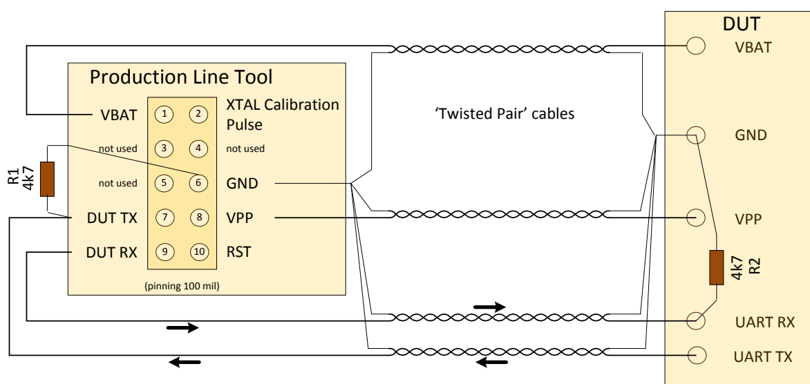
Figure 170: Location of Pull-Down Resistors
