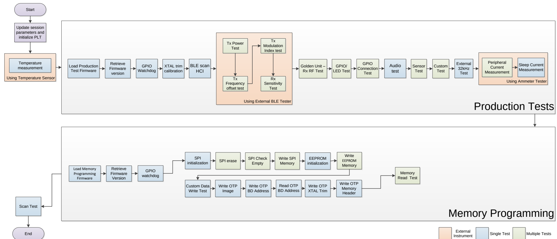
Figure 22: DA1458x Test Sequence
