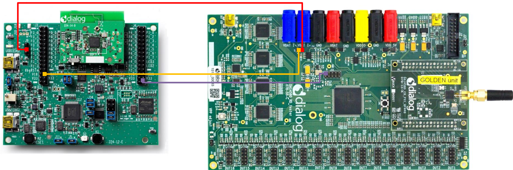
Figure 177: DA1468x PRO DK Ammeter Connection with PLT
