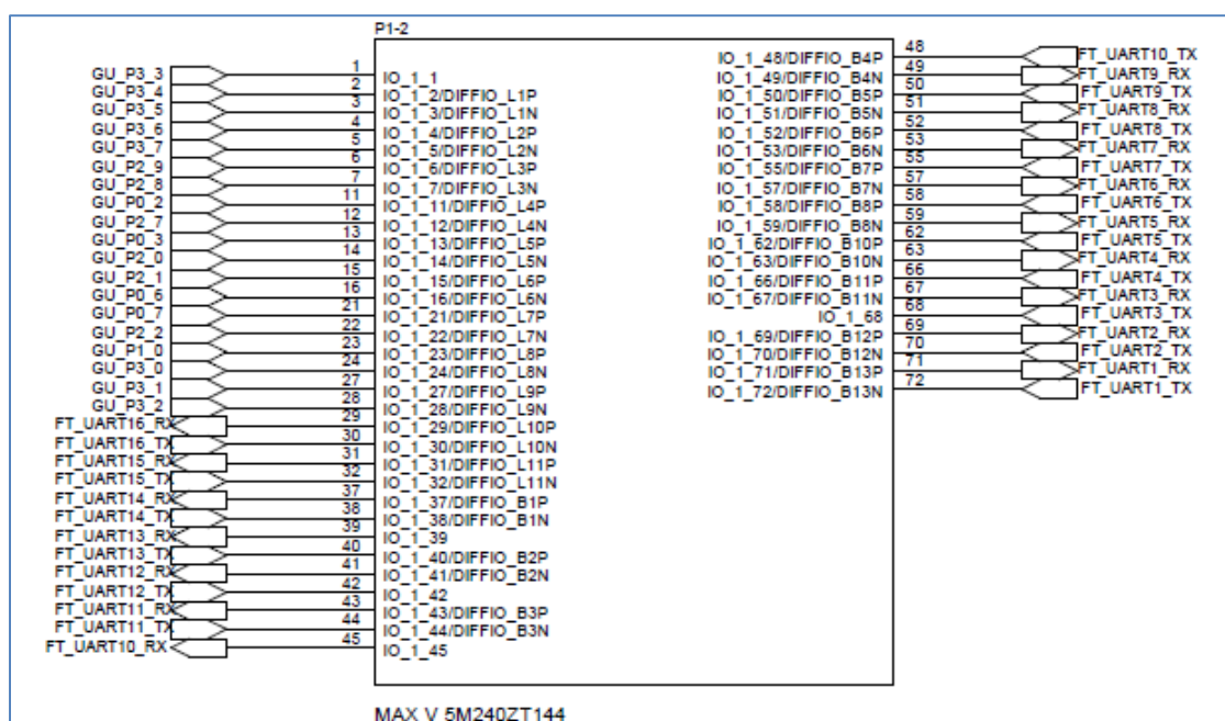
Figure 150: CPLD FTDI and GU Control Connections
