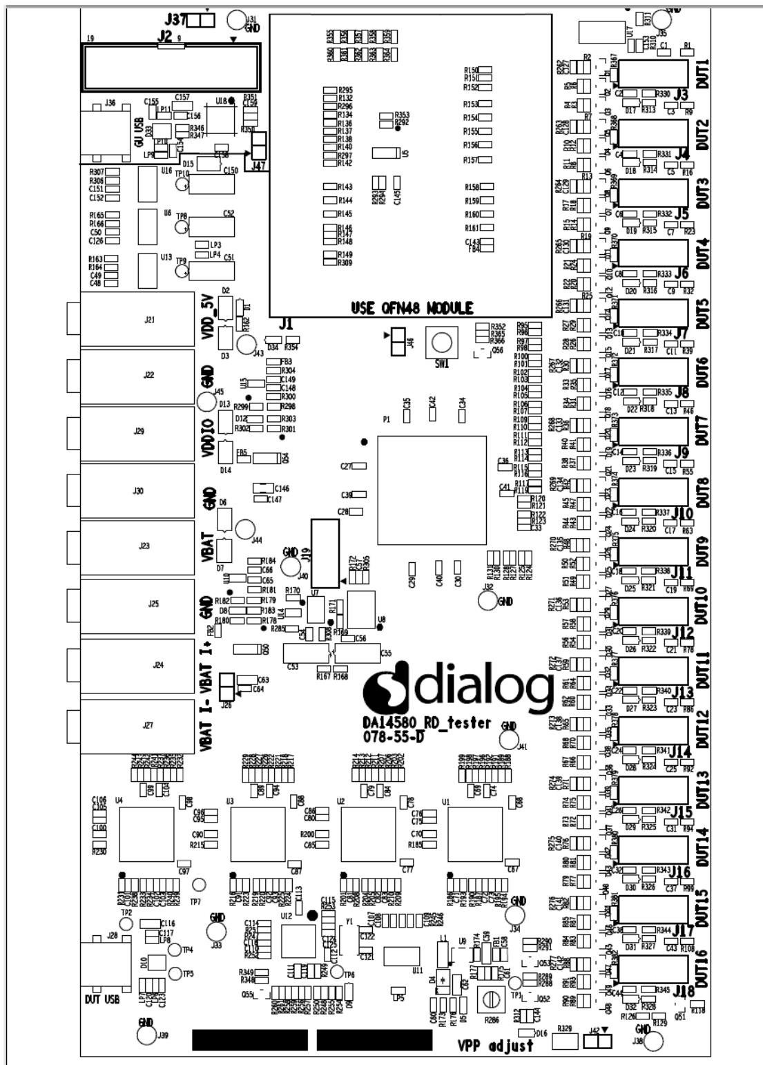
Figure 147: Top-view of PLT PCB Version D
