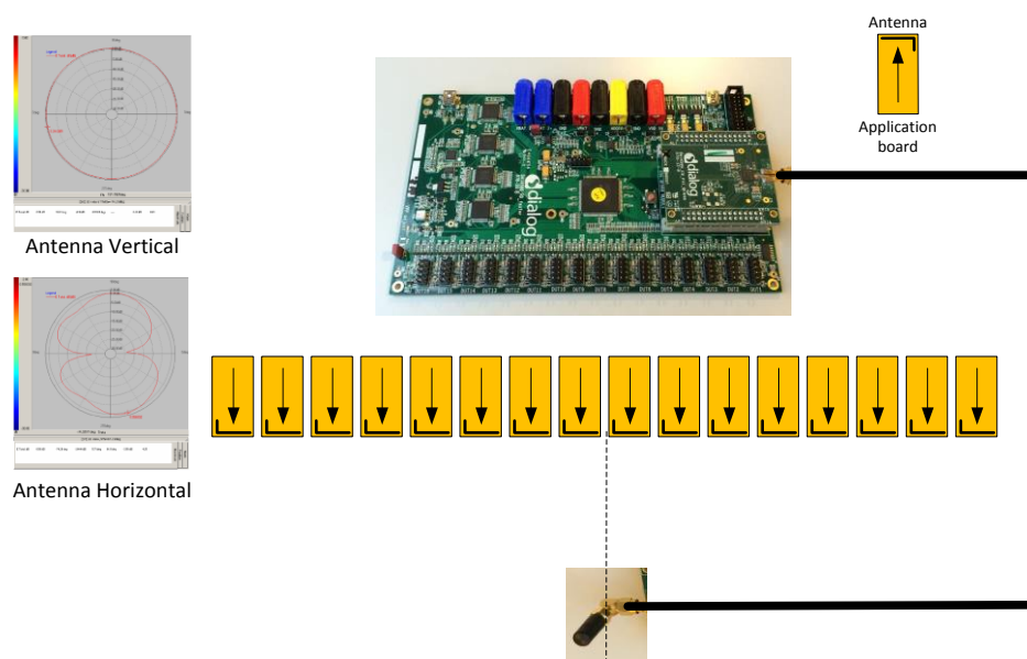
Figure 162: Possible Solution of Antenna on Cable and DUTs Put in Line
