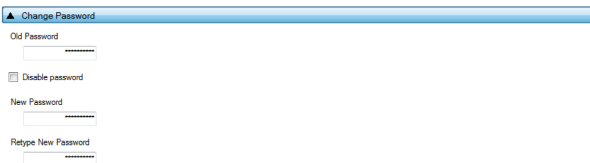
Figure 113: Security
