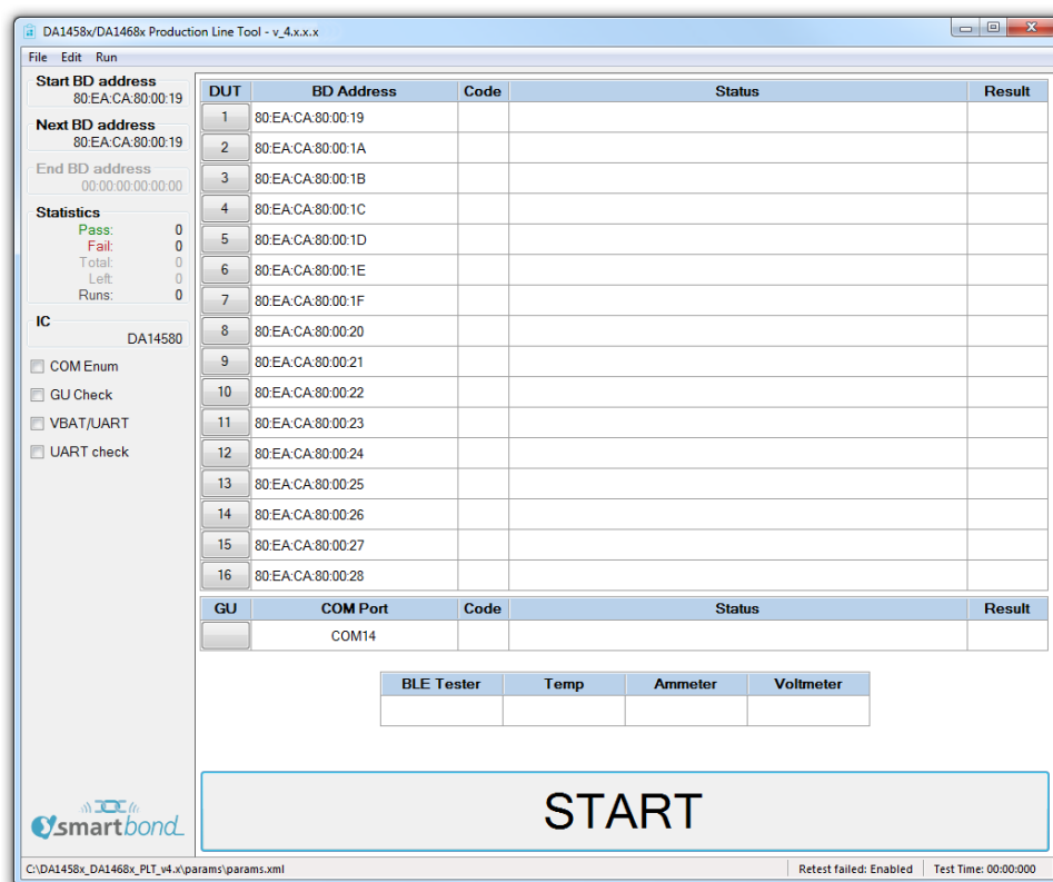
Figure 114: GUI PLT Main Screen
