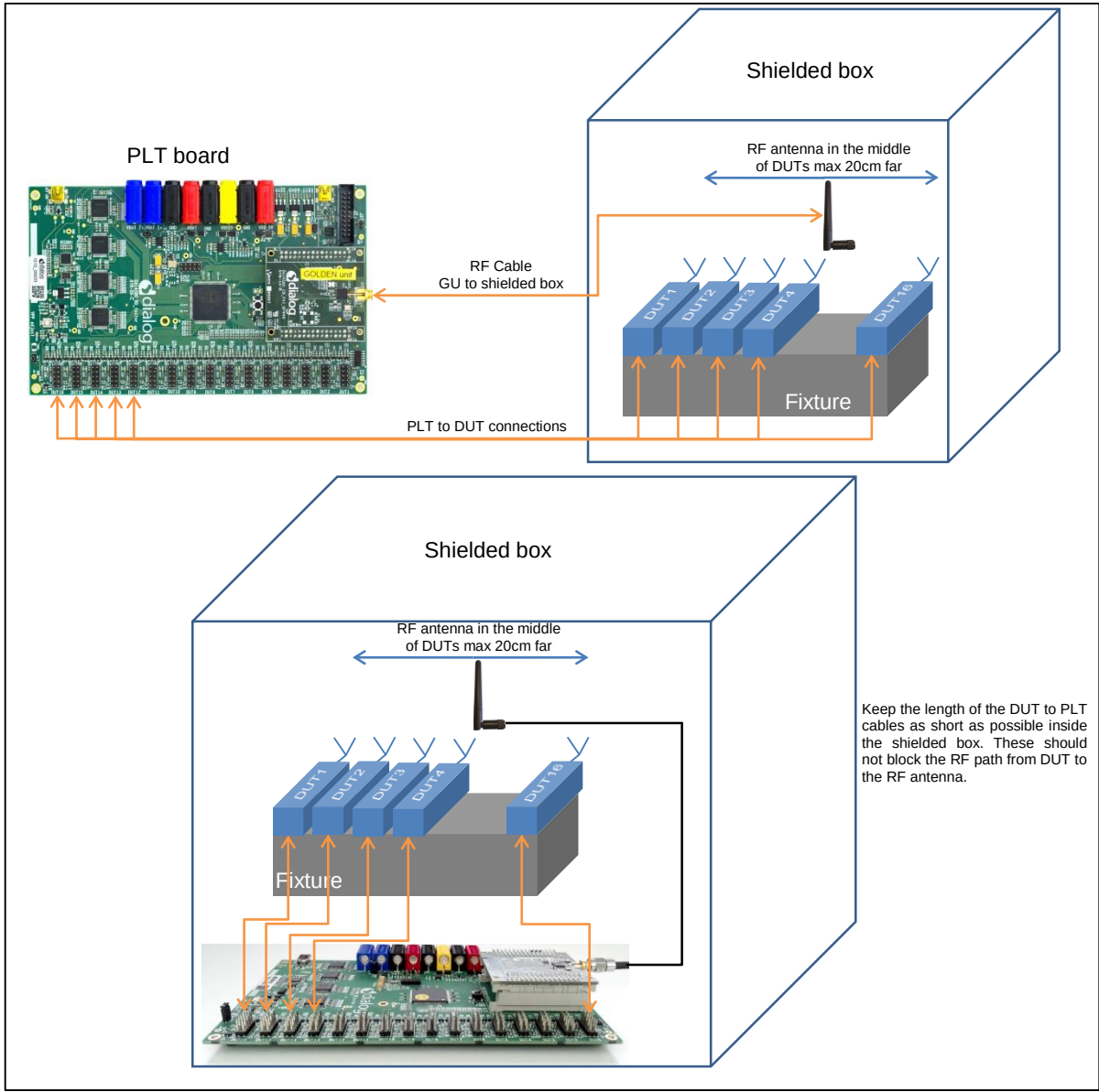
Figure 164: Setup diagram
