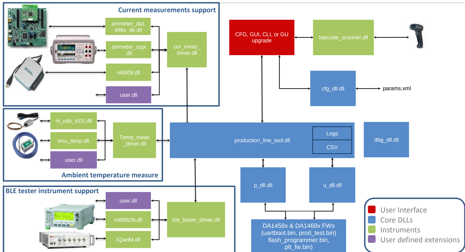
Figure 20: Production Line Tool Software Block Diagram
