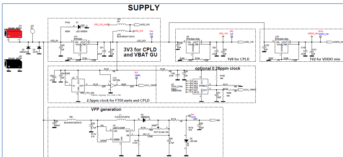
Figure 156: GU Supply and VPP Generation
