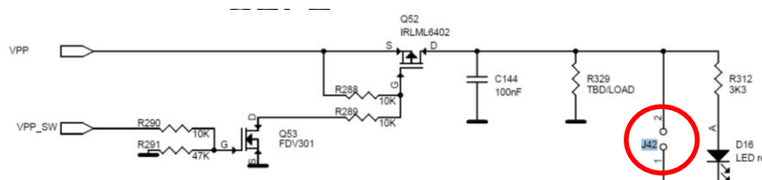
Figure 13: VPP Control Circuit Schematic
