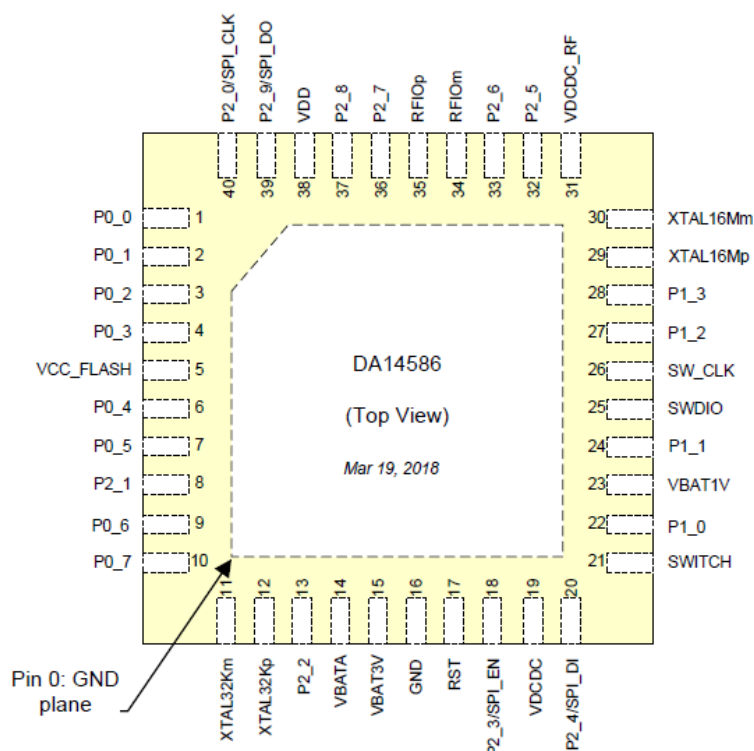
Figure 173: Pin Assignment of DA14586 - QFN40
