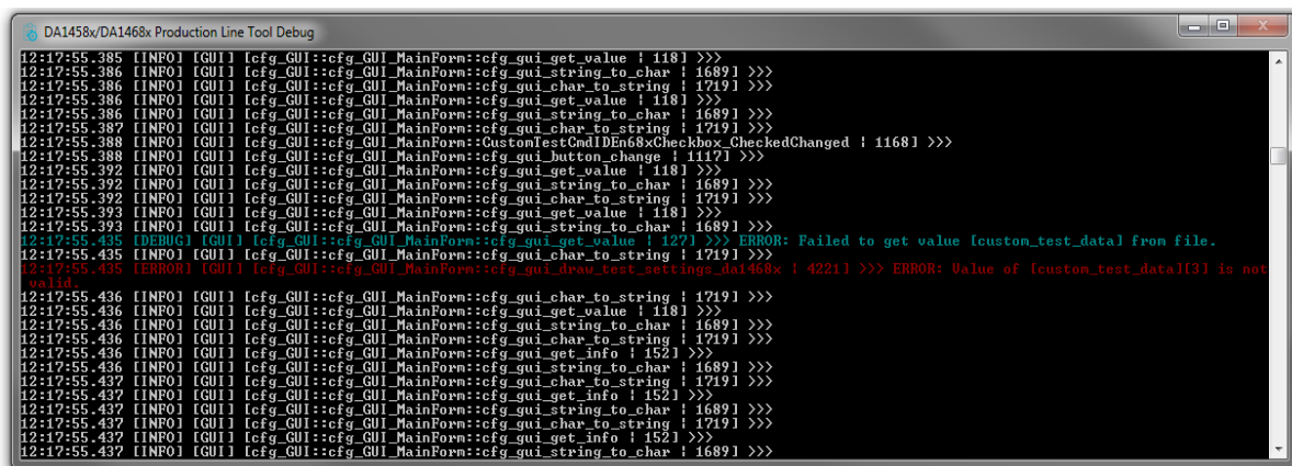
Figure 125: Debug Console
