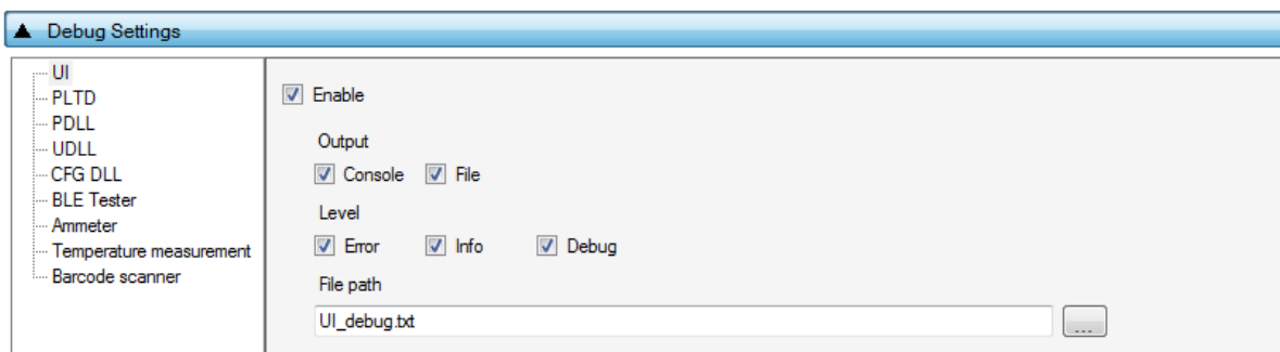
Figure 112: Debug Settings
