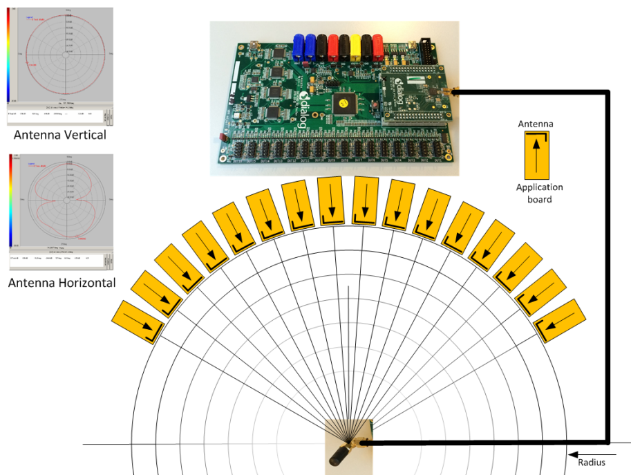
Figure 161: Possible Solution of Antenna on Cable and Fixed Radius of DUTs to Antenna
