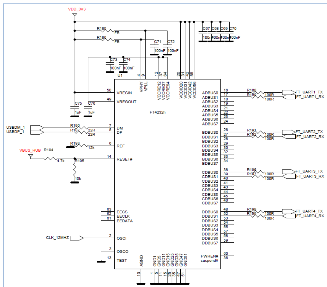
Figure 151: FTDI Chip for USB UART to DUTs 1, 2, 3 and 4
