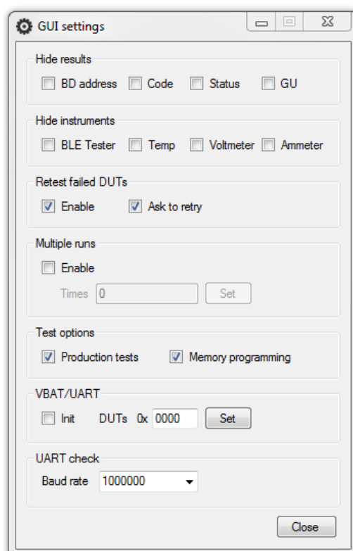
Figure 115: GUI PLT Settings
