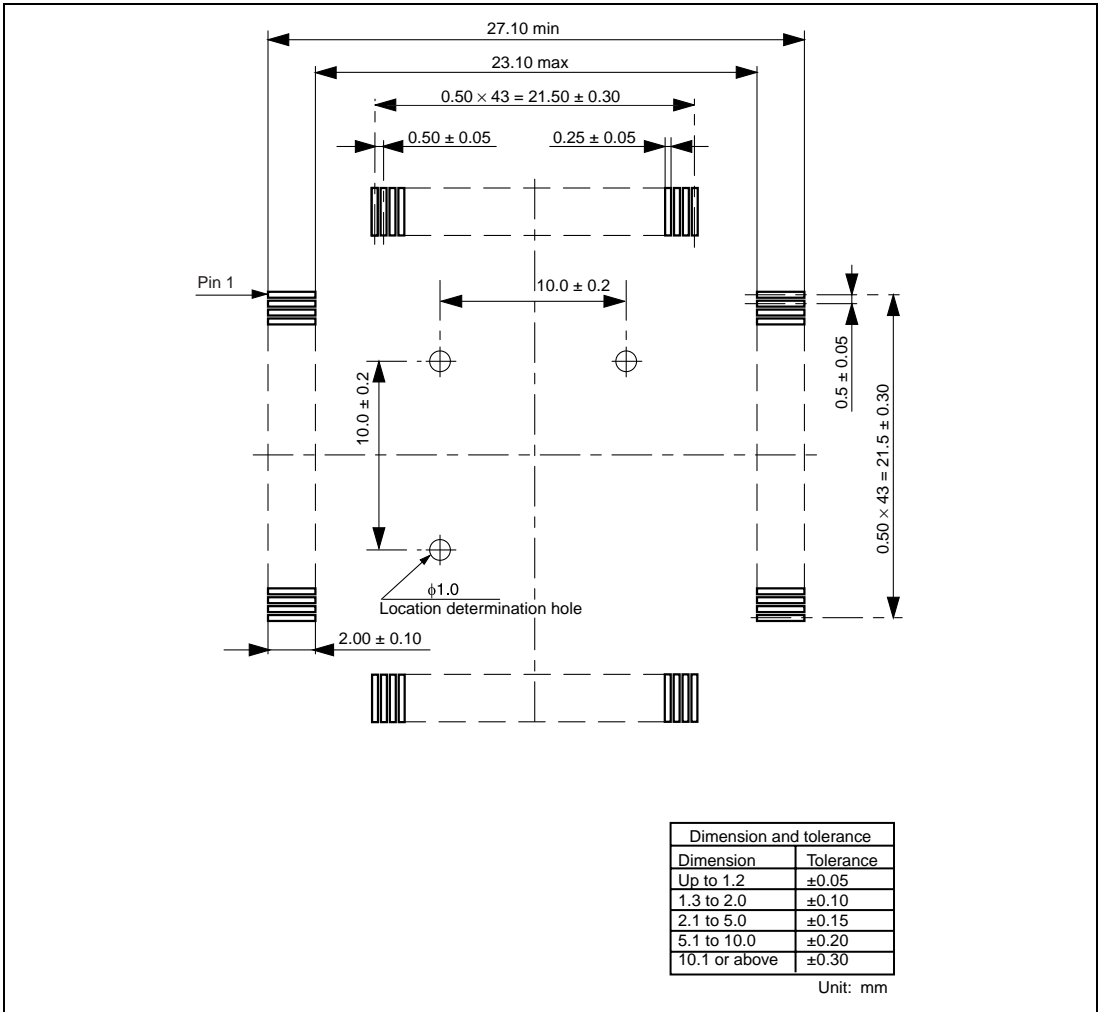
Figure 4 Recommended Dimensions for Mount Pad
