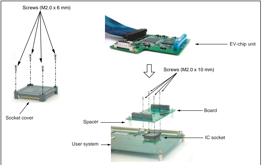
Figure 1 User System Interface Board for the SH7286 PLQP0176KB-A Package
