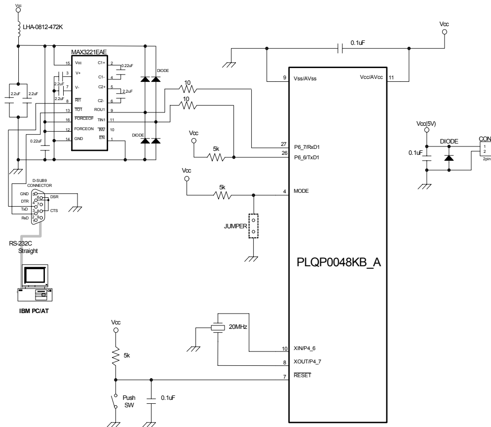
Figure 2 Circuit Example with RS-232C Cable
