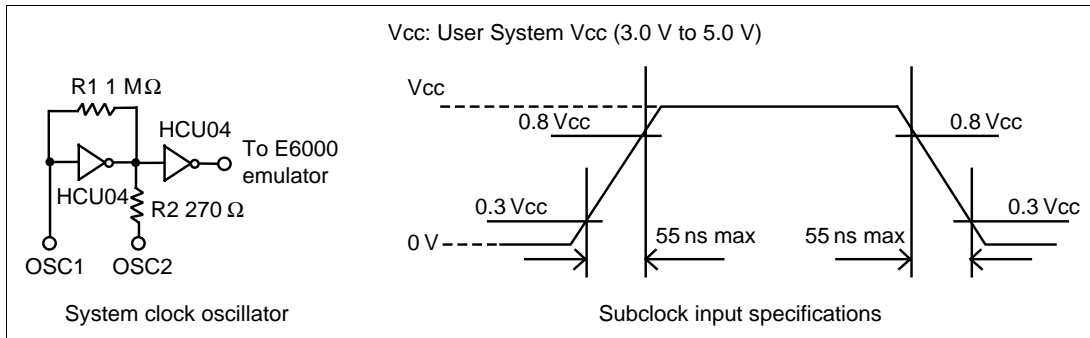
Figure 9 System Clock Oscillator and Subclock Input Specifications
