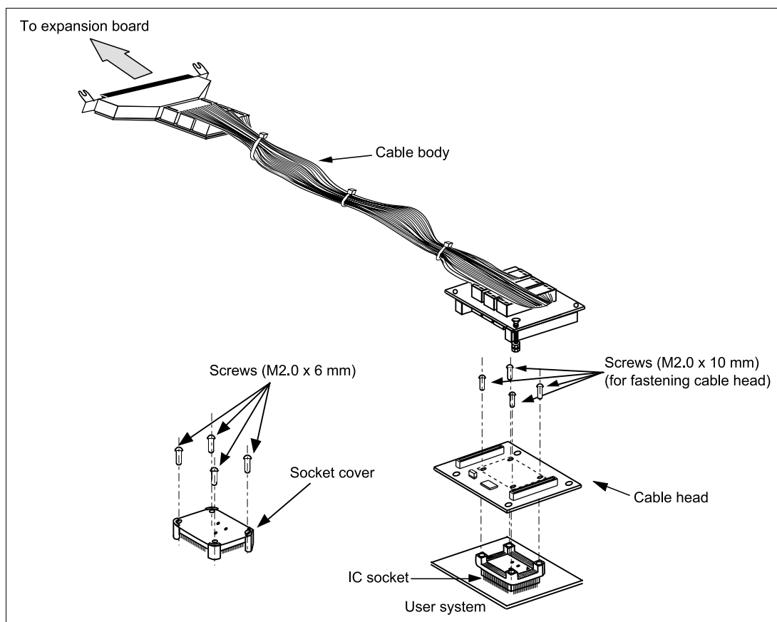
Figure 1 HS3857ECN61H User System Interface Cable
