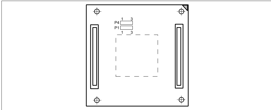
Figure 11 Jumper Socket Location
