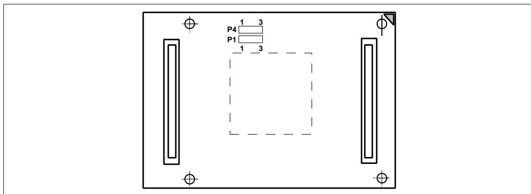
Figure 11 Jumper Location
