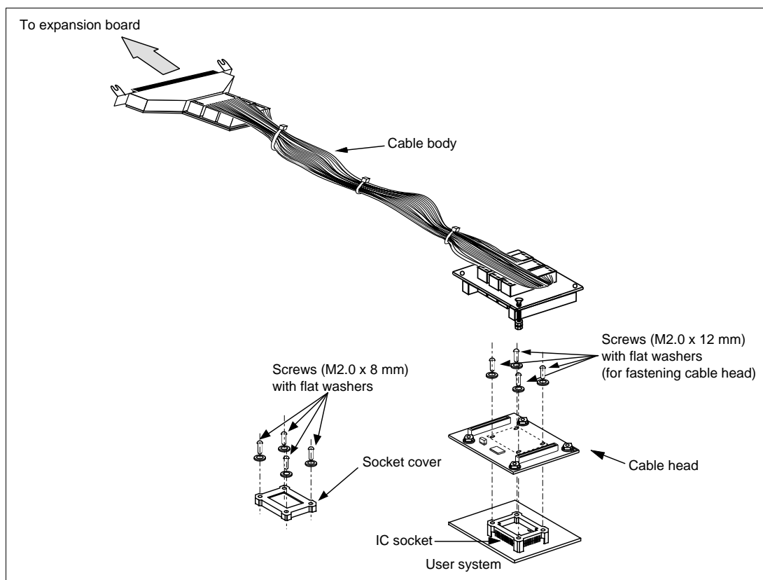
Figure 1 HS3857ECH61H User System Interface Cable
