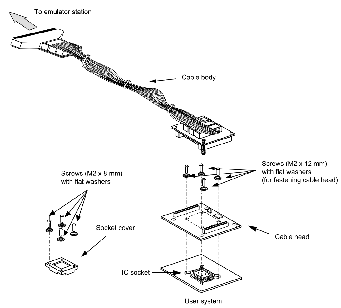
Figure 1 HS3032ECH61H User System Interface Cable
