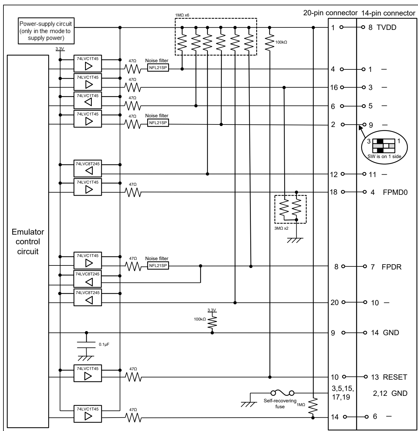
Figure D Interface Circuits in the E2 Emulator (1-Wire UART)
