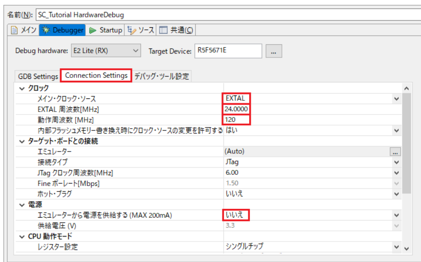
図 6-2 Connection Settings
