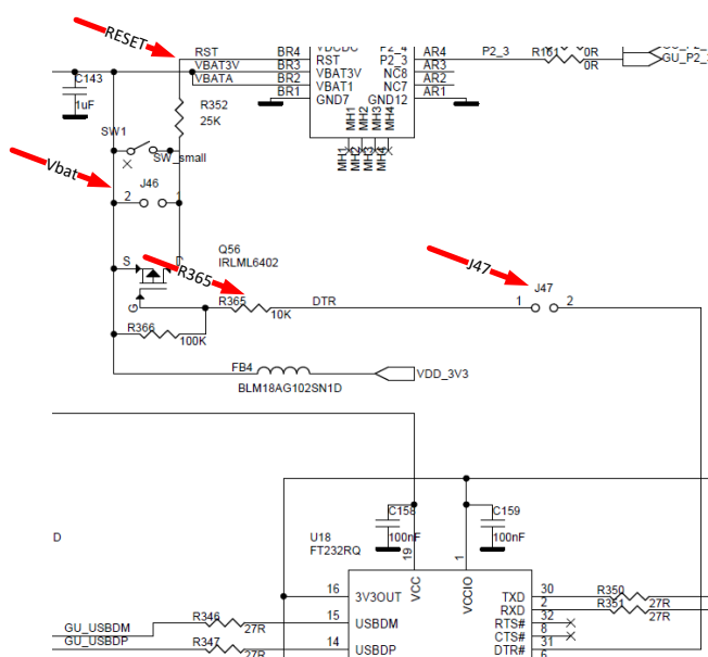
Figure 155: R365, J47 and RESET Shown in Electrical Schematic
