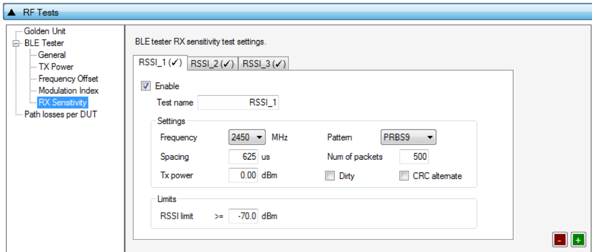
Figure 60: BLE Tester RX Sensitivity - DA14531
