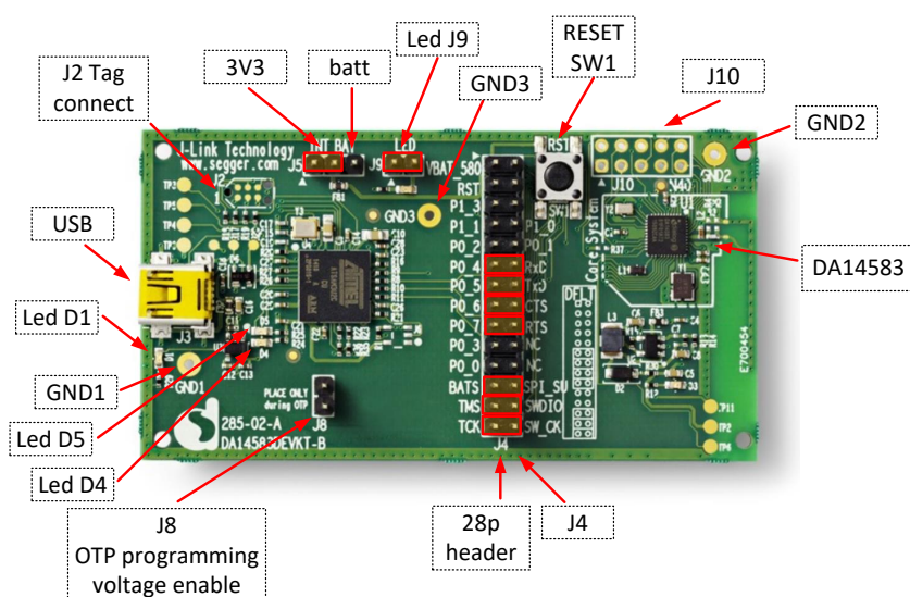
Figure 17: Top view of PCB DA14583 with components and functionalities
