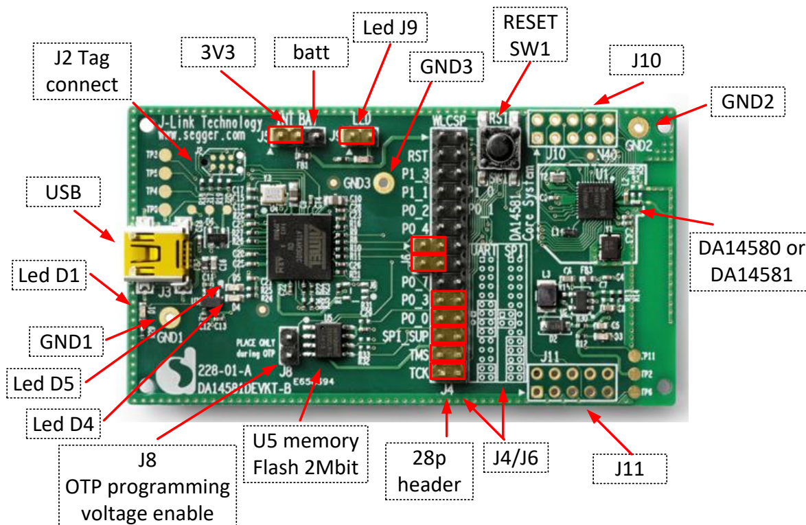
Figure 44: A general overview of the DA14581 development board
