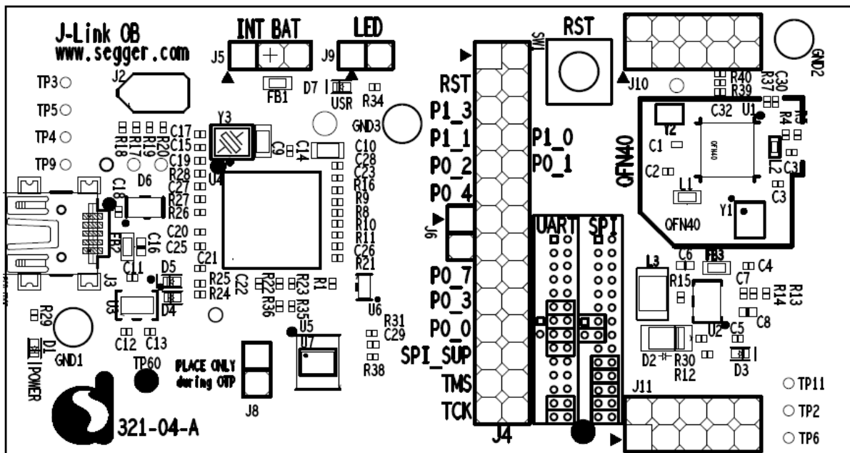
Figure 19: Components on PCB top layer of the DA14585/6 Basic kit (321-04-A)
