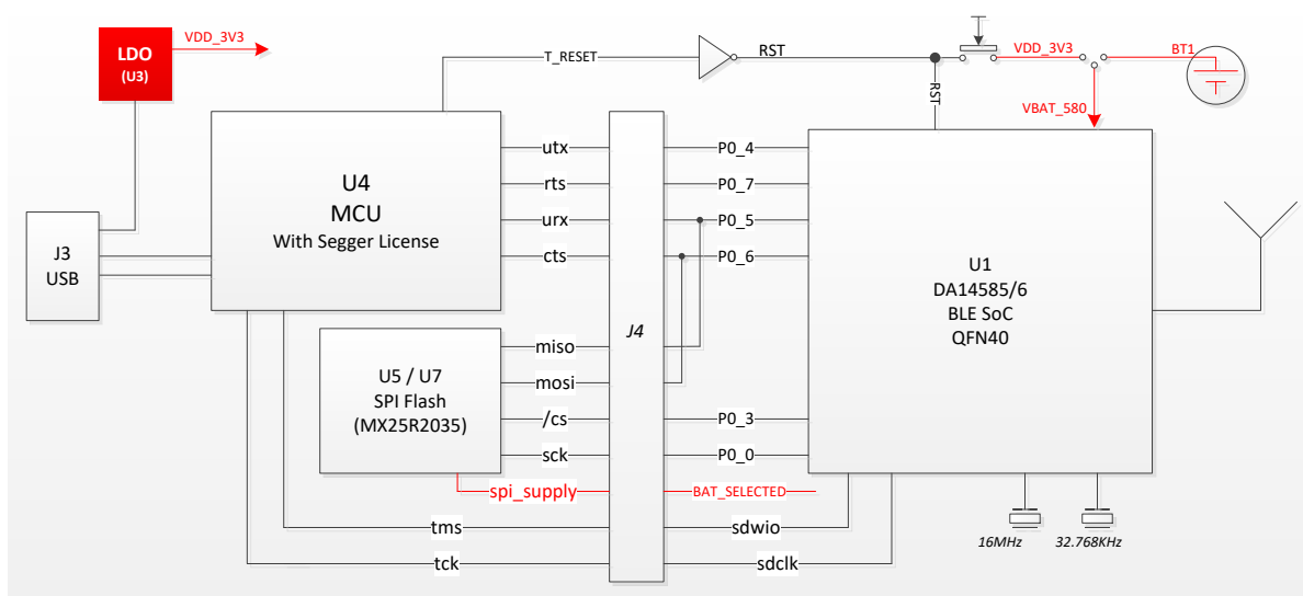
Figure 18: DA1458x DEKT-B block diagram
