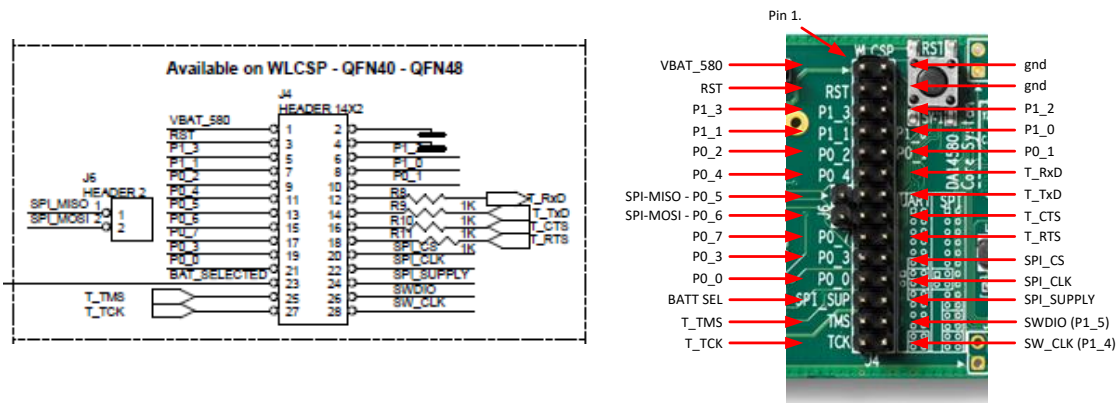
Figure 32: DA14580/581 layout of headers J4 and J6
