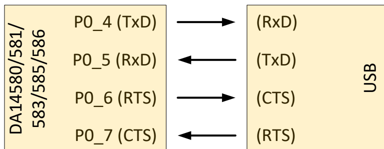
Figure 38: Data direction of UART within J4
