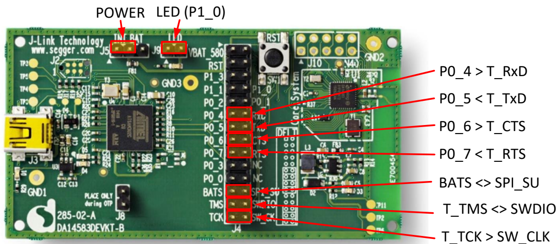
Figure 33: (Fabrication Default) DA14583 UART boot settings (Tx P0_4 and Rx P0_5)
