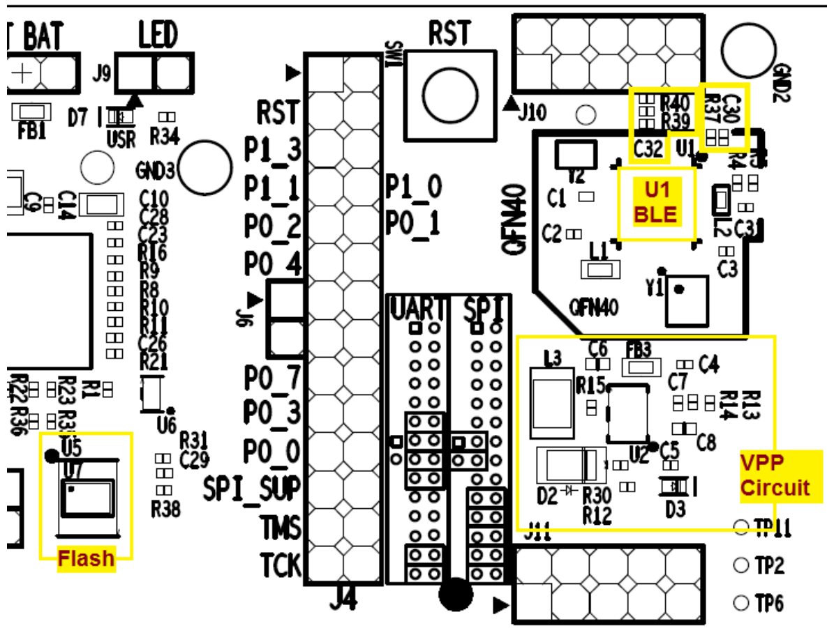
Figure 51: Location of the components that enables various versions of DA1458x family
