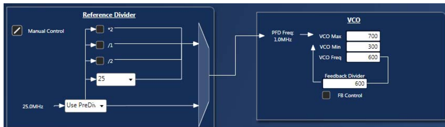
Figure 12. Internal Block of PLL1
