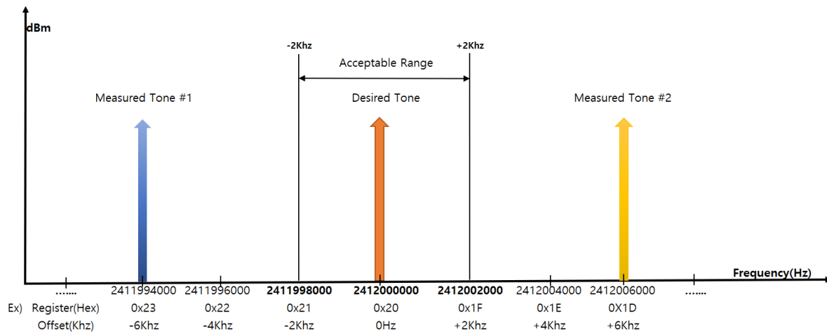
Figure 2. Offset in frequency domain
