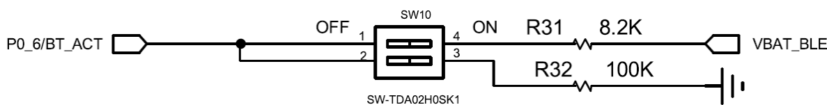
Figure 9. RF switch setup on DA16600 EVB
