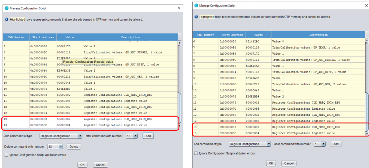
Figure 13. OTP register check for XTAL trimming
