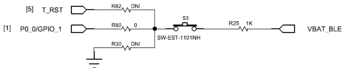
Figure 8. DA14531 hardware reset on DA16600 EVB
