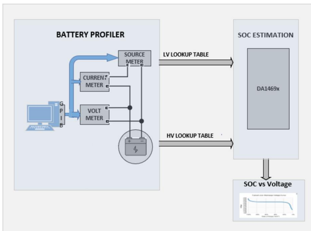
Figure 8: Bench Setup for Battery Profiling
