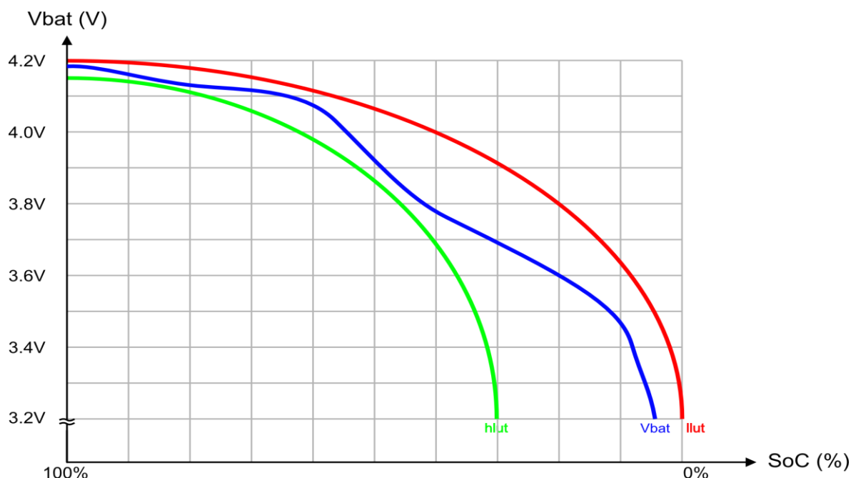
Figure 11: SoC Graph
