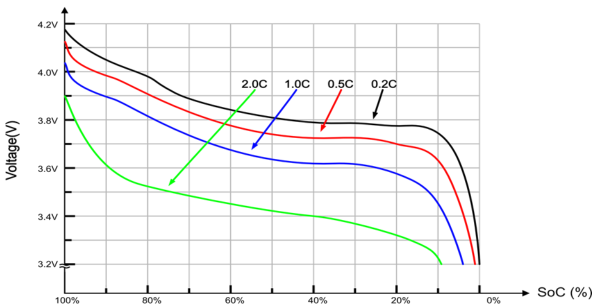
Figure 2: Open Circuit Voltage versus State of Charge for Different Discharge Rates
