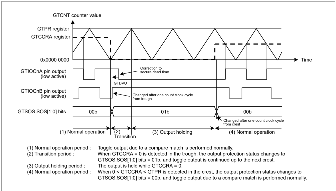
Figure 21.174 Example of Output Protection Function Operation When GTCCRA is Set to 0x0000 0000 during Buffer Transfer at Troughs (Restored to 0 < \text{GTCCRA} < \text{GTPR} during Buffer Transfer at Crests, Active Level: Low) (n = 0 to 9)
