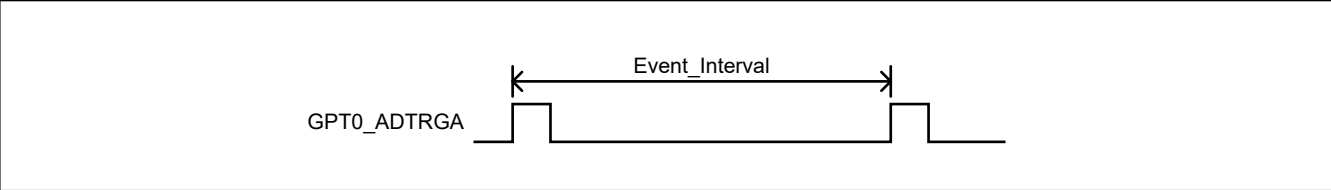
Figure 17.3 Example of GPT0_ADTRGA Event Interval
