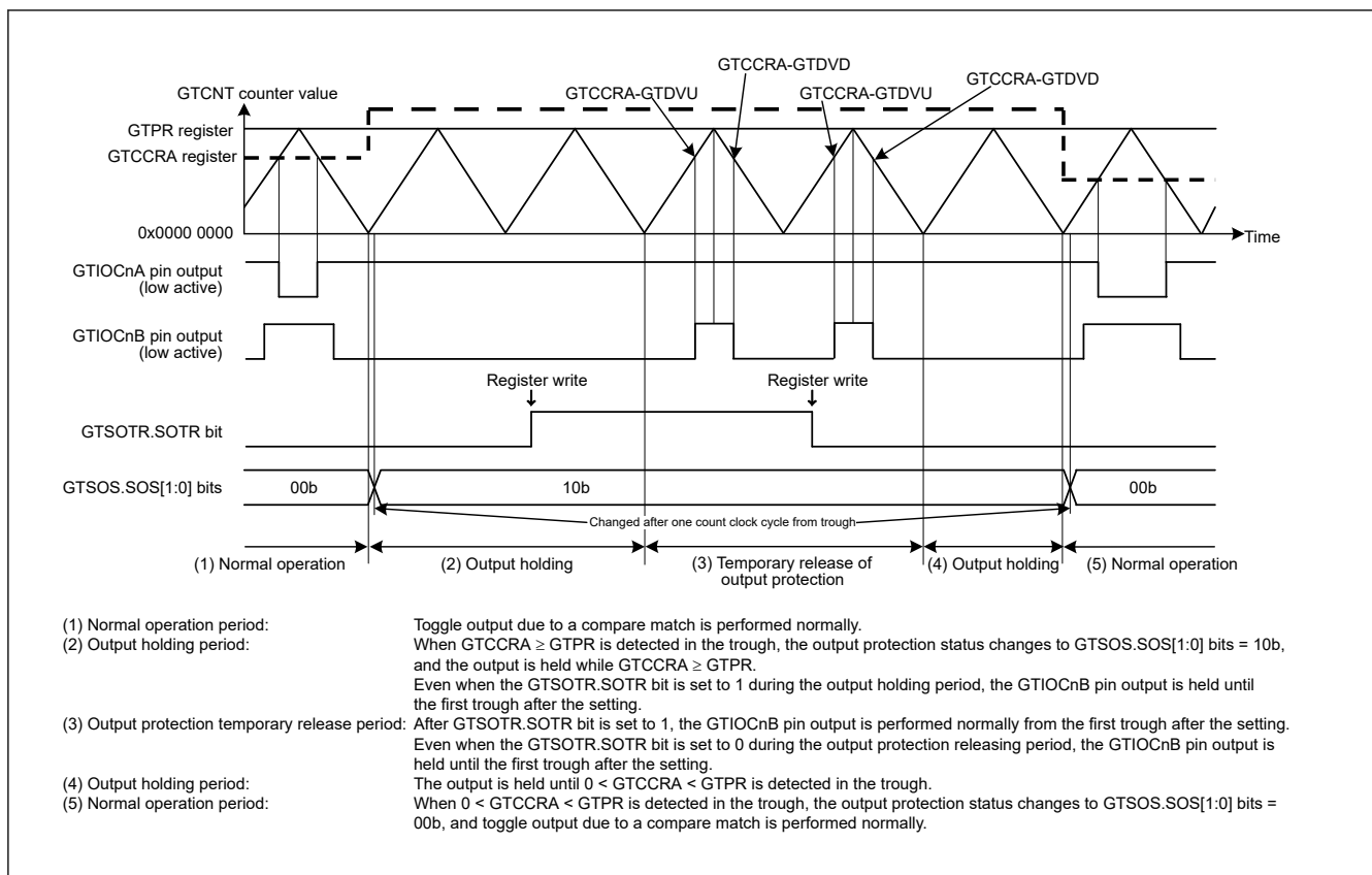
Figure 21.181 Example of Temporary Release of Output Protection When the Setting of the GTCCRA \geq GTPR during Buffer Transfer at Troughs (Restored to 0 < \text{GTCCRA} < \text{GTPR} during Buffer Transfer at Troughs, Active Level: Low) (n = 0 to 9)
