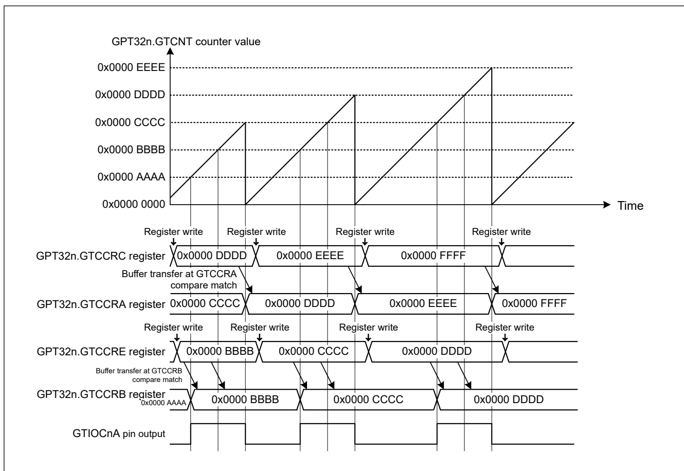
Figure 21.26 Example of GTCCRA and GTCCRB Registers Buffer Operation (Output Compare, Saw-Wave PWM Mode 2, Buffer Transfer at GTCCRA Register Compare Match, Counter Clearing, Low Output, Buffer Transfer at GTCCRB Register Compare Match, High Output) (n = 4 to 9)
