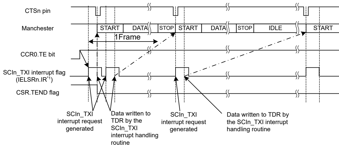
Figure 26.51 Example of Start-of-Transmission Operation for Serial Transmission in Manchester Mode (Without Preface but with the CTS Function)
