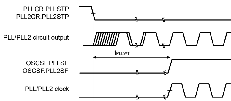
Figure 46.6 PLL/PLL2 clock oscillation start timing
