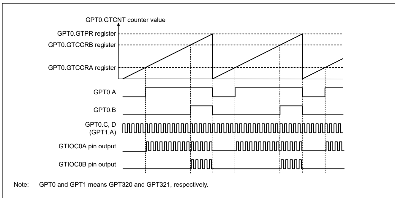
Figure 21.139 Example of Inter Channel Logical Operation
