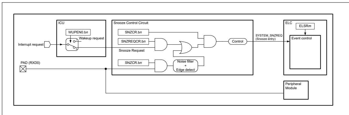
Figure 10.5 Snooze mode entry configuration
