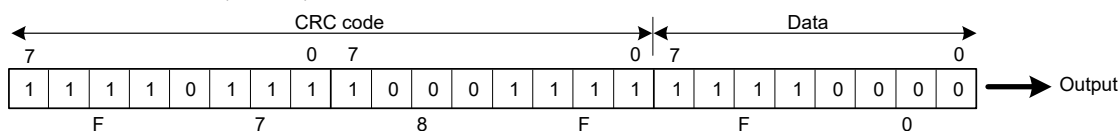
Figure 31.2 LSB-first data transmission
