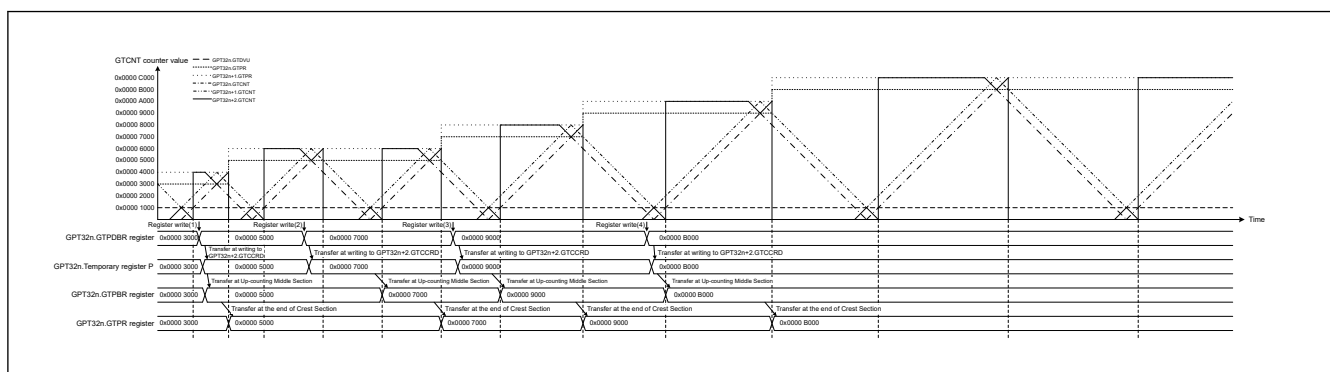
Figure 21.22 Example of GTPR double buffer operation with complementary PWM mode 1
