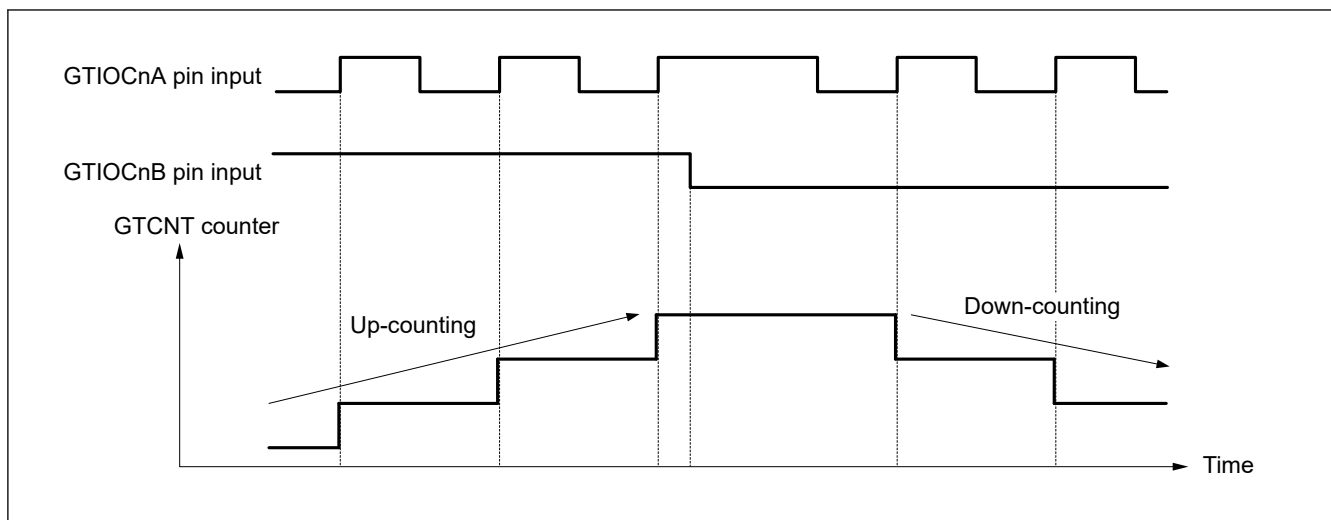
Figure 21.122 Example of phase counting mode 2 (B)
