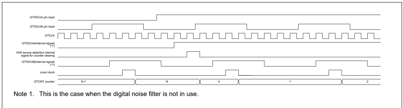
Figure 21.102 Examples of the Timing of Operations for Counter Clearing in Response to a Rising Edge of the Input on the GTIOcA Pin (During Counting Triggered by Hardware Source)
