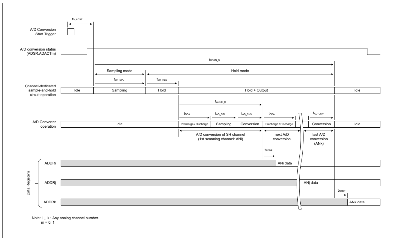
Figure 36.53 A/D conversion processing time (SAR mode with channel-dedicated sample-and-hold circuit)
