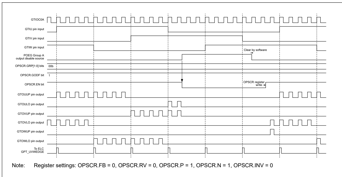
Figure 21.137 Example of GPT_OPS Output Disable Control Operation
