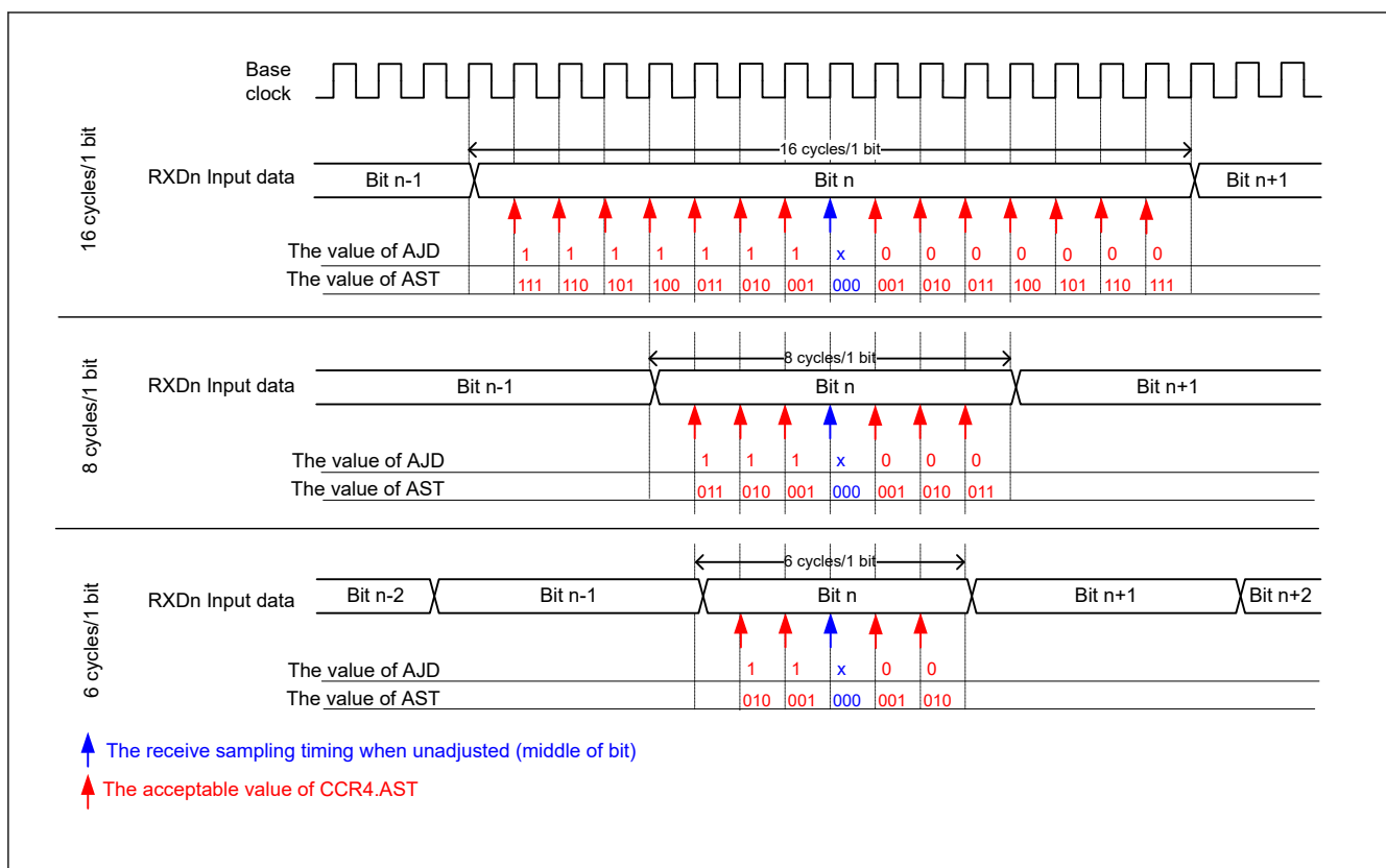
Figure 26.27 Overview of the adjustment operation for the reception sampling timing (asynchronous mode using internal clock)
