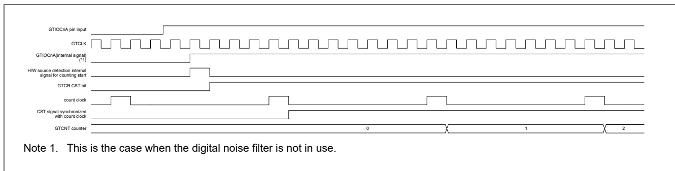
Figure 21.88 Example of Timing of Operations to Start Counting in Response to a Rising Edge of the Input on the GTIOCnA Pin
