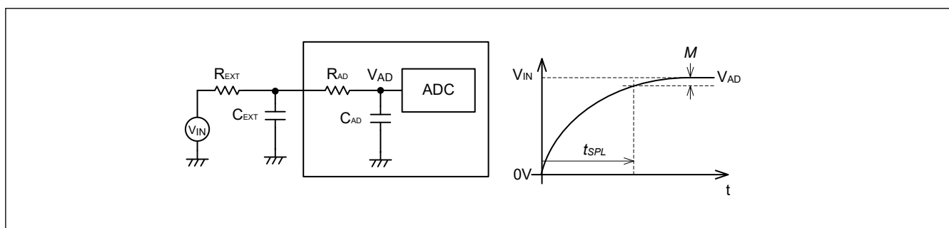
Figure 36.60 Simplified model of sample-and-hold circuit for A/D converter
