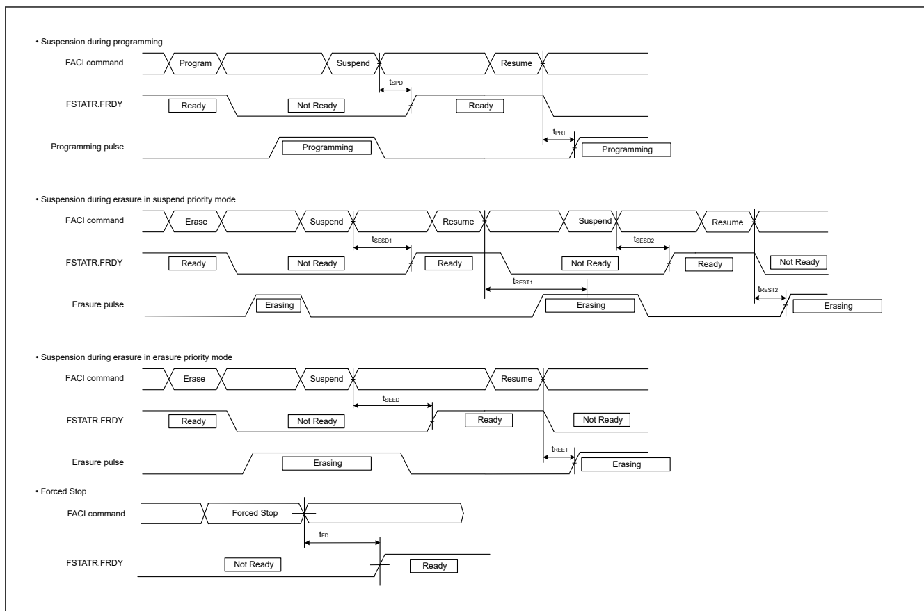
Figure 46.59 Suspension and forced stop timing for flash memory programming and erasure
