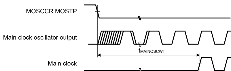
Figure 46.4 Main clock oscillation start timing
