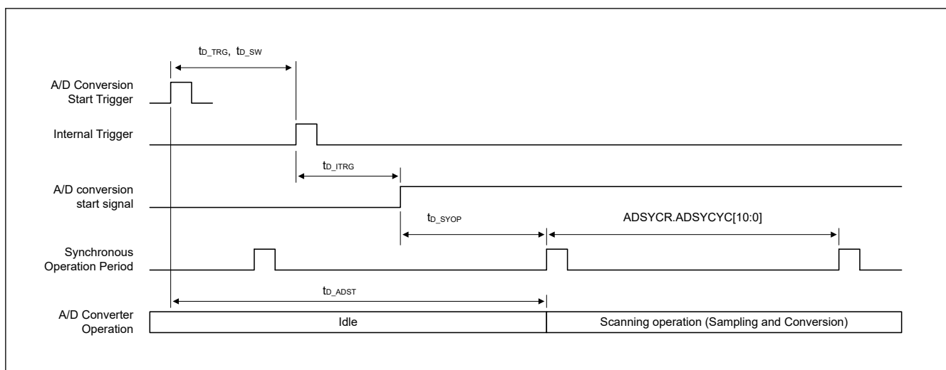
Figure 36.51 Scan start processing time
