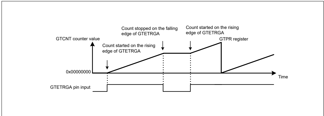
Figure 21.91 Example of count start/stop operation by a hardware source started on the rising edge of GTETRGA pin input, and stopped on the falling edge of GTETRGA pin input
