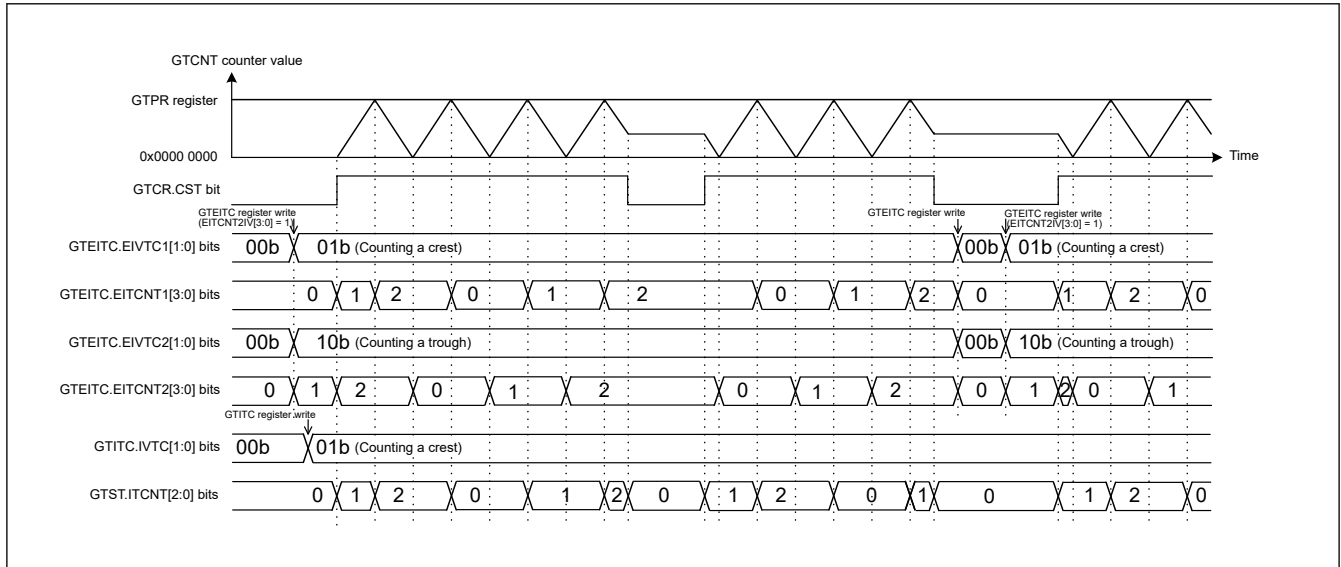
Figure 21.146 Example of Counter Operation for Interrupt Skipping
