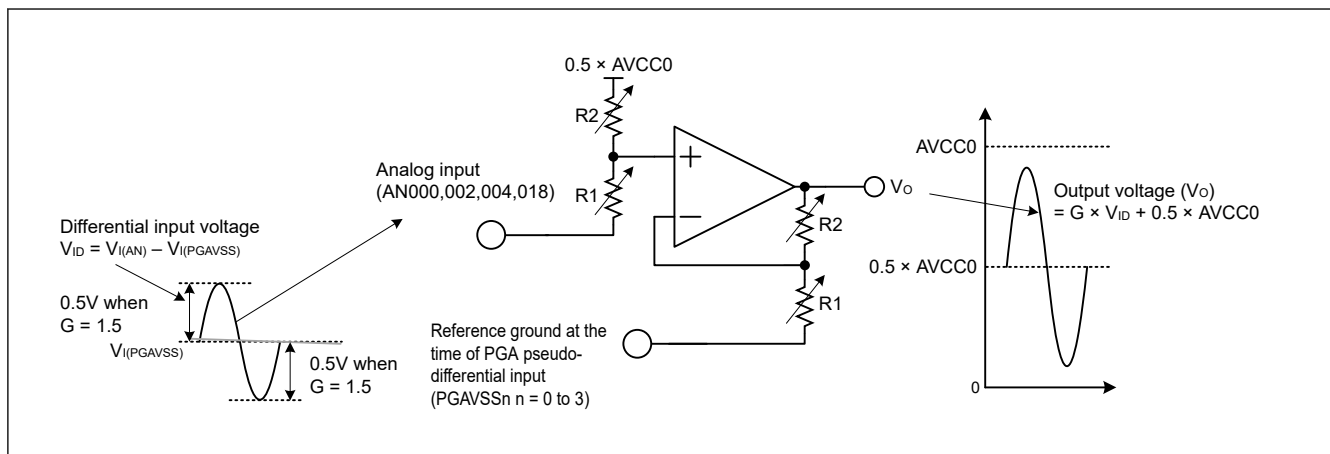
Figure 46.53 Input and Output Signal Levels with the PGA's Pseudo-Differential Setting
