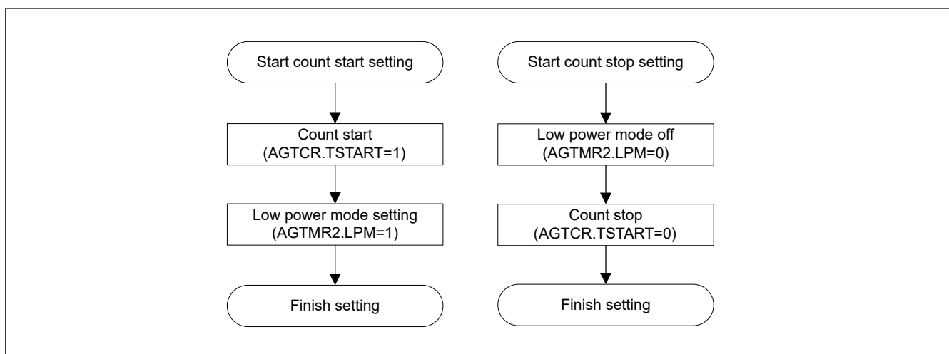
Figure 23.2 LPM how to write flow chart
