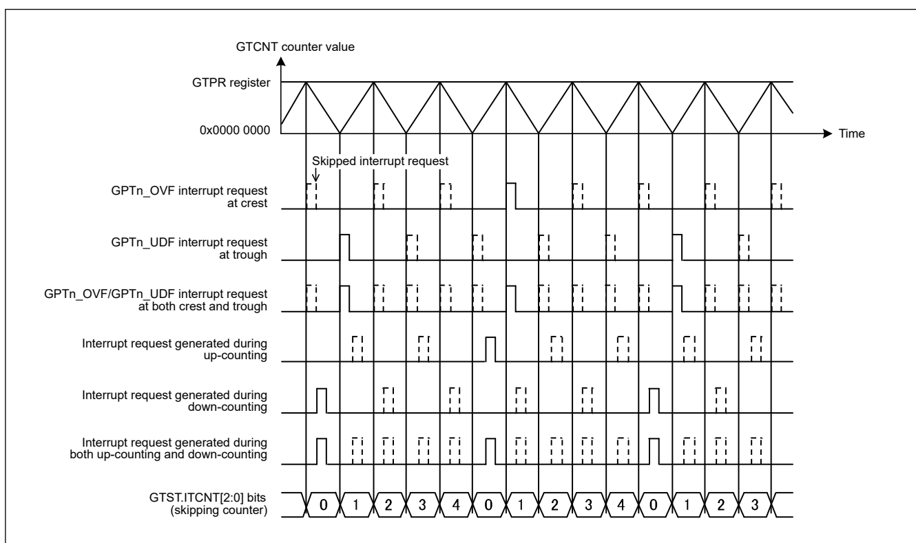
Figure 21.142 Example of Interrupt Skipping Function Operation (Triangle Waves, Counting and Skipping Both Troughs and Crests, Skipping Count: 4)
