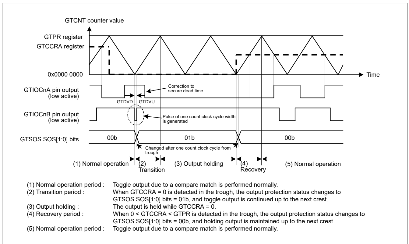
Figure 21.175 Example of Output Protection Function Operation When GTCCRA is Set to 0x0000 0000 during Buffer Transfer at Crests (Restored to 0 < \text{GTCCRA} < \text{GTPR} during Buffer Transfer at Troughs, Active Level: Low) (n = 0 to 9)
