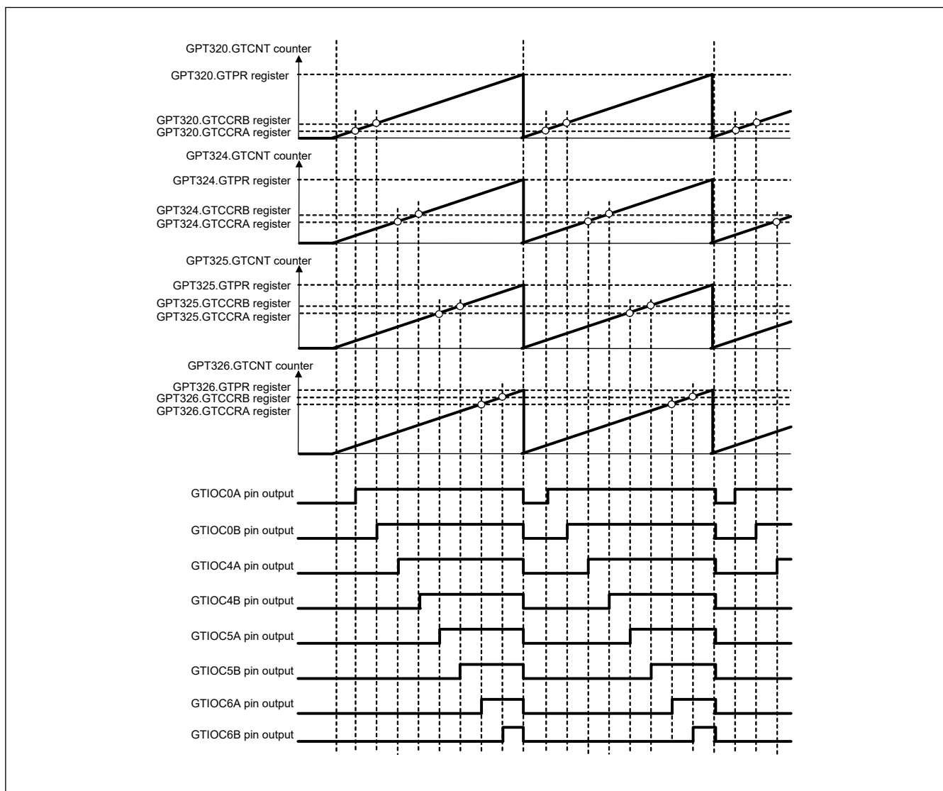
Figure 21.112 Example of synchronized PWM output
