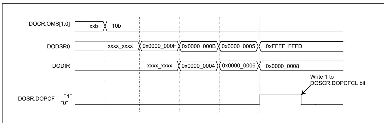
Figure 40.9 Example of Operation in Data Subtraction Mode
