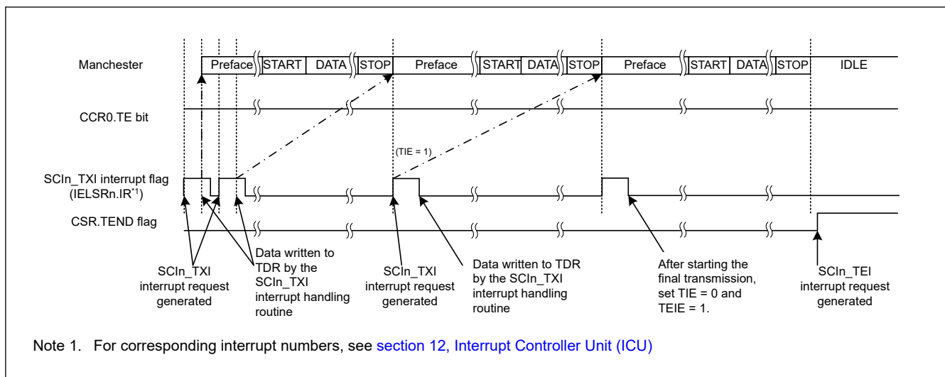
Figure 26.52 Example of End-of-Transmission Operation for Serial Transmission in Manchester Mode (with Preface but Without the CTS Function)
