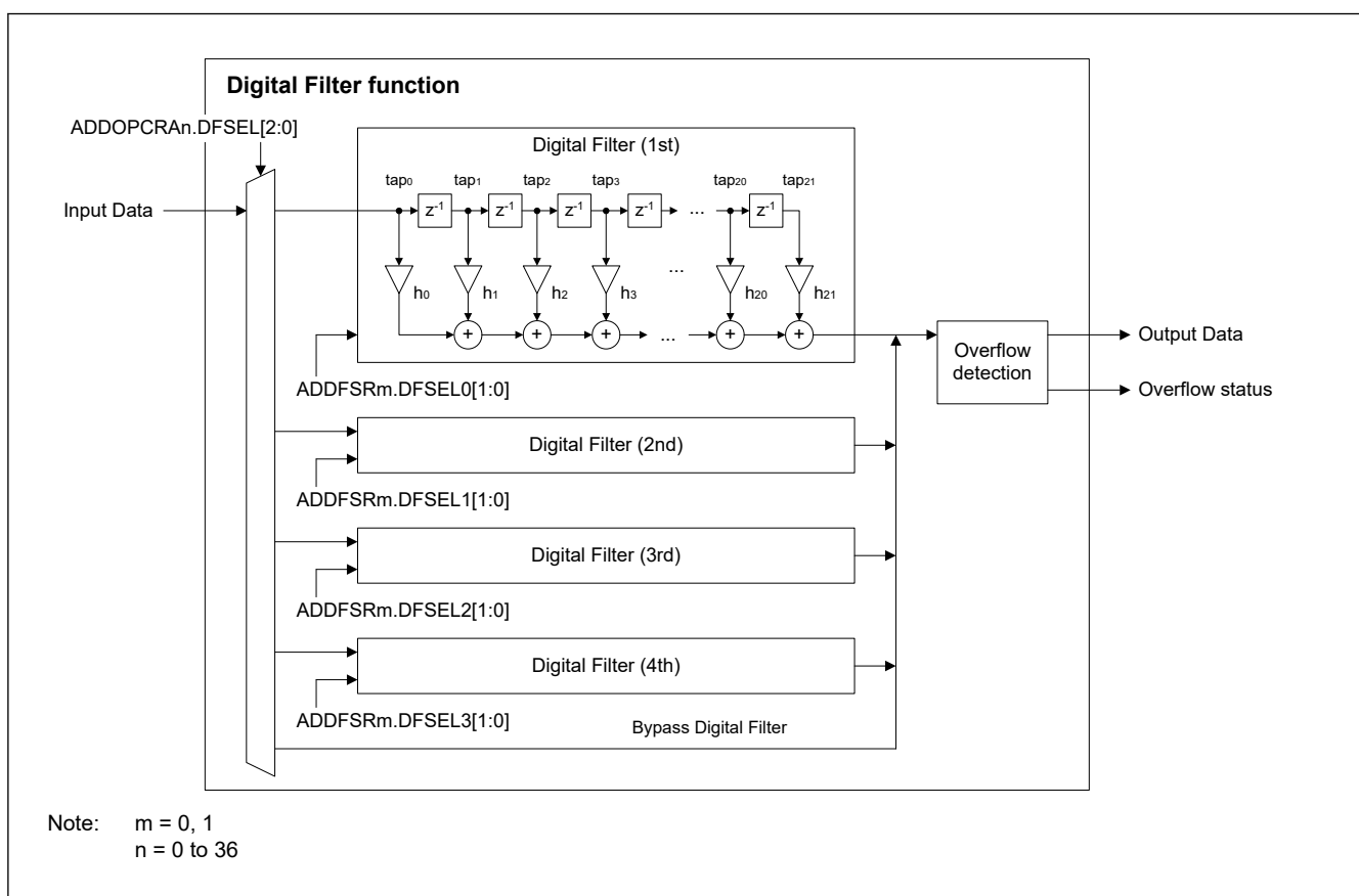
Figure 36.32 Block diagram of Digital Filter
