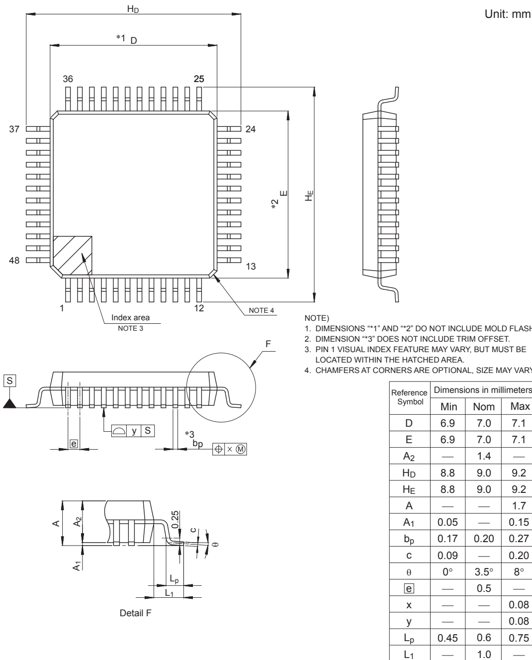
Figure A2.4 LQFP 48-pin
