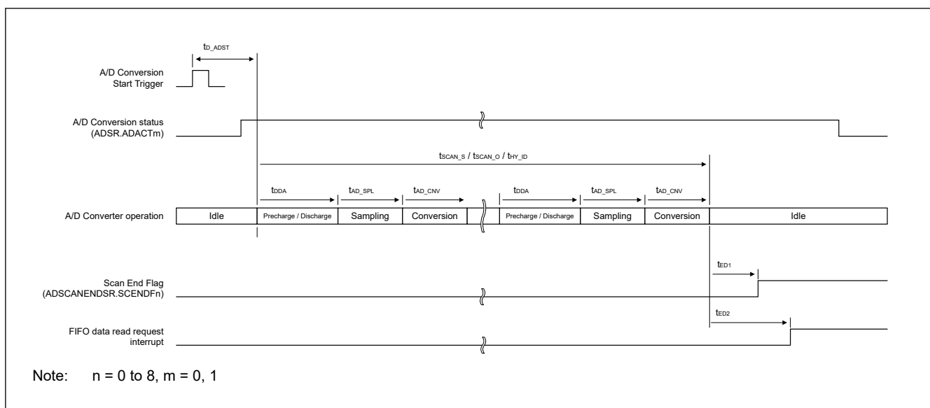
Figure 36.57 Scan end processing time (SAR/Oversampling/Hybrid mode – Single scan mode)
