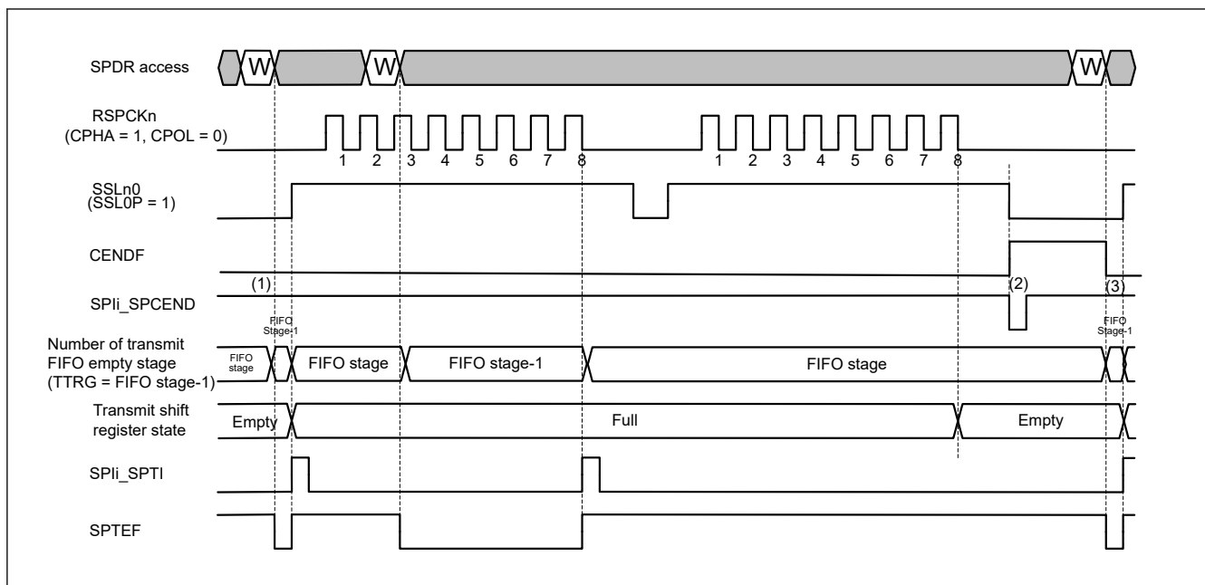
Figure 30.40 Example of Communication End Interrupt Operation (Transmit-Receive/Transmit Slave mode on SPI Operation/Motorola-SPI)
