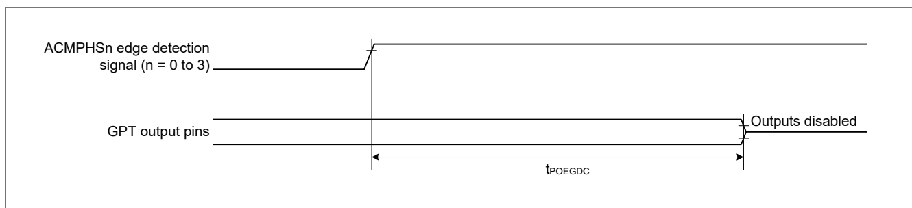
Figure 46.18 Output Disable Time for POEG in Response to Edge Detection Signal from ACMPHS
