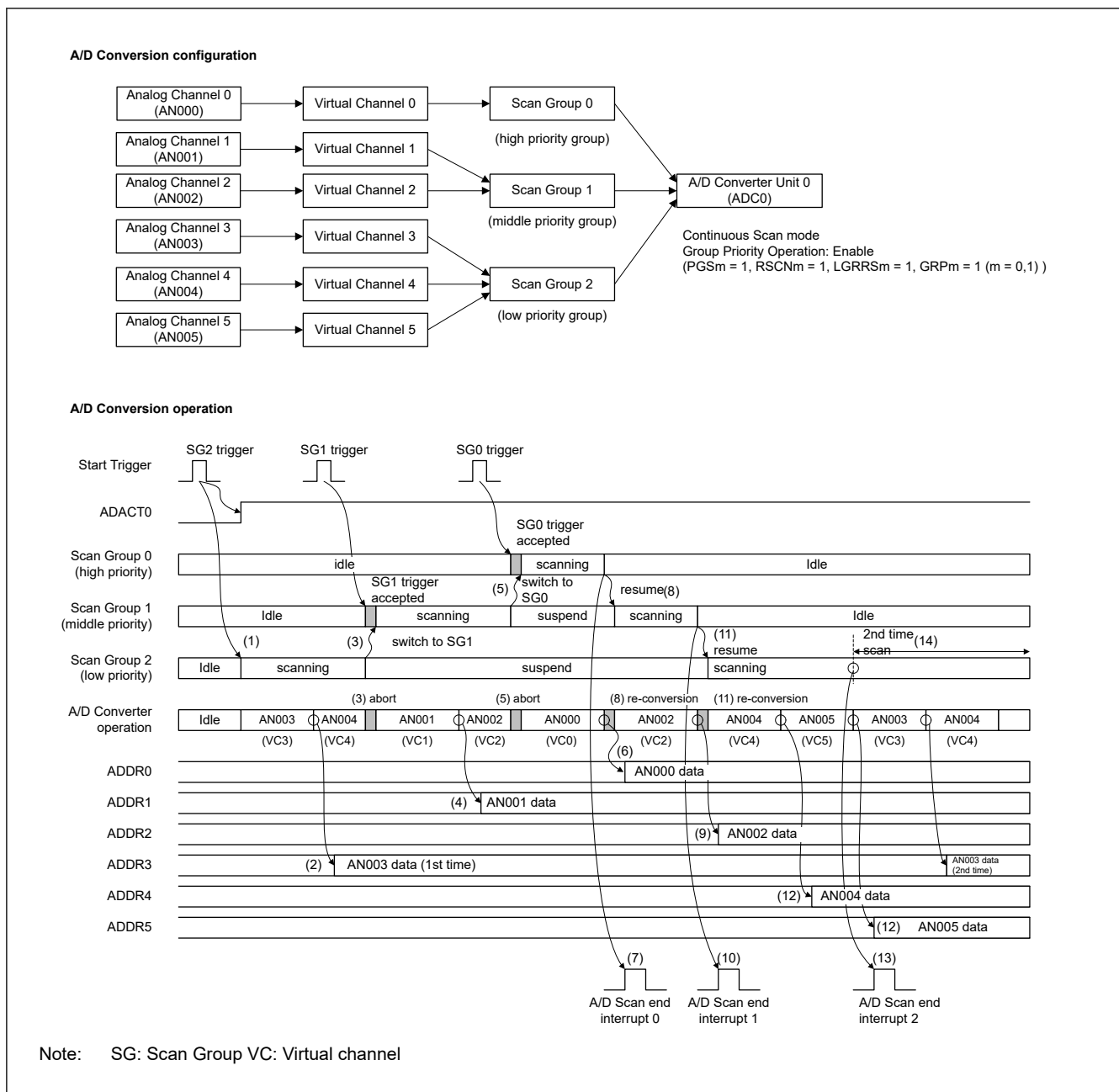
Figure 36.28 Example of group priority operation in SAR mode – Continuous scan mode (3 groups)
