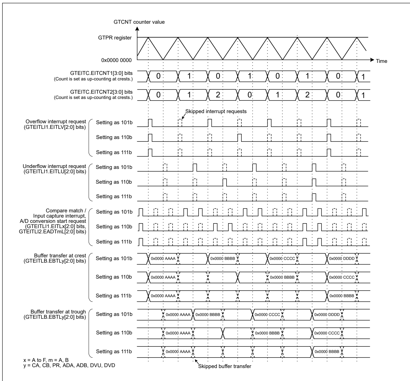
Figure 21.151 Example of Extended Interrupt Skipping Function Operation (Triangle Waves, Counting Crests, Extended Interrupt Skipping 1 Skipping Count: 1, Counting Crests, Extended Interrupt Skipping 2 Skipping Count: 2, Extended Interrupt Skipping Counter 2 Initial Value: 0, Skipped in the Period other than GTEITC.EITCNTk bits (k = 1, 2) as GTEITC.EIVTTk bits.)
