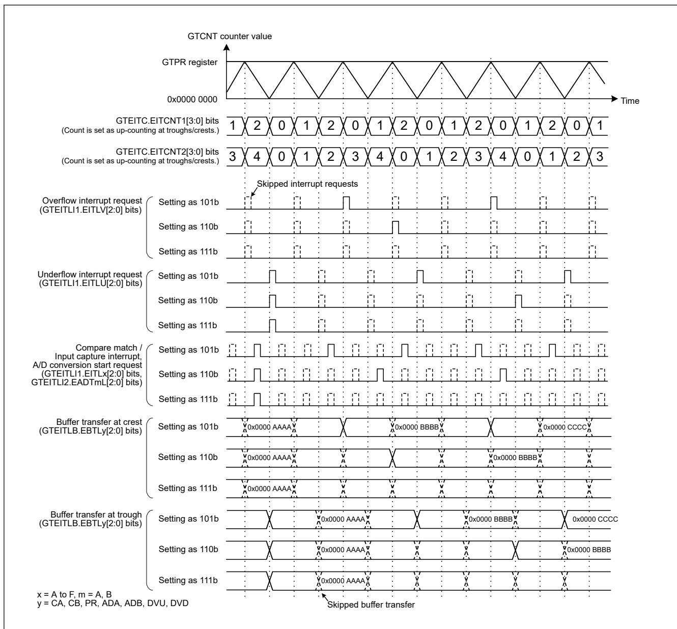
Figure 21.153 Example of Extended Interrupt Skipping Function Operation (Triangle Waves, Counting both Crests and Troughs, Extended Interrupt Skipping 1 Skipping Count: 2, Counting both Crests and Troughs, Extended Interrupt Skipping 2 Skipping Count: 4, Extended Interrupt Skipping Counter 2 Initial Value: 0, Skipped in the Period other than GTEITC.EITCNTk bits (k = 1, 2) as GTEITC.EIVTTk bit.)
