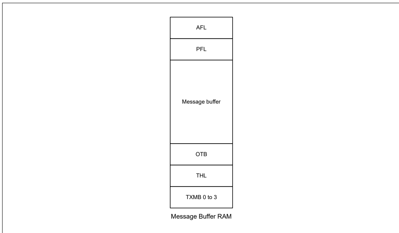
Figure 28.55 RAM area grouping
