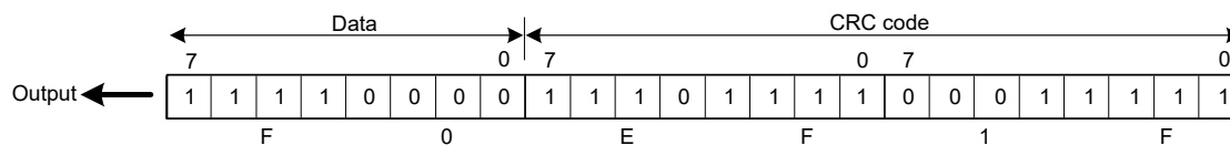
Figure 31.3 MSB-first data transmission
