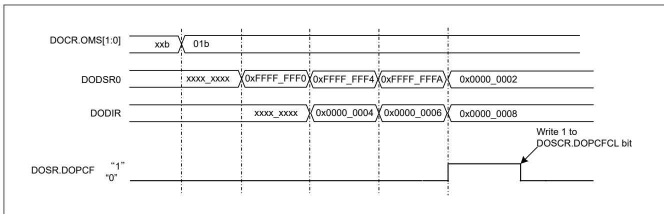
Figure 40.8 Example of Operation in Data Addition Mode
