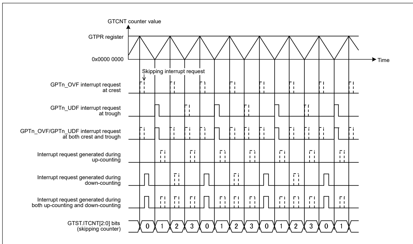
Figure 21.143 Example of Interrupt Skipping Function Operation (Triangle Waves, Counting and Skipping Both Troughs and Crests, Skipping Count: 3, Skipping Started at Up-Counting)
