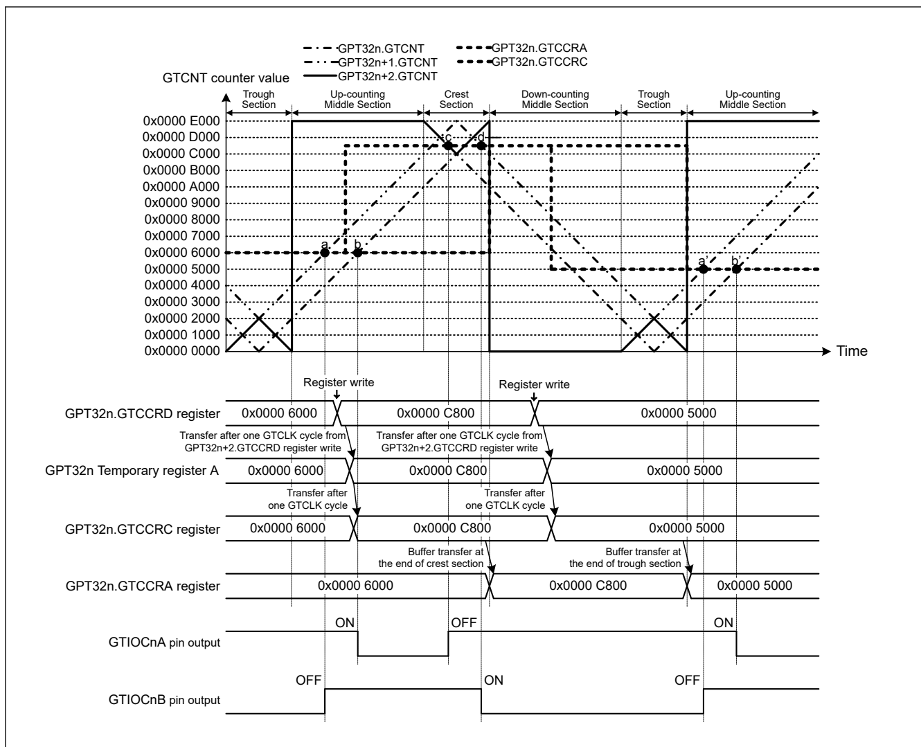
Figure 21.56 Example of Compare Match Generation Sequence Operation in Complementary PWM Mode Complementary PWM mode 3 single buffer operation, GTIOCnA pin = Low / GTIOCnB pin = High at GTCCRA register compare match during up-counting, GTIOCnA pin = High / GTIOCnB pin = Low at GTCCRA register compare match during down-counting, the dead time value is 0x0000 2000, compare match generation order: a → b → c → d) (n = 4, 7)
