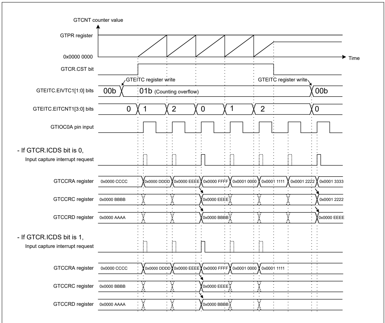
Figure 21.156 Example of Input Capture Operation in the Extended Interrupt Skipping Function Operation (Up-Counting Saw Waves, Counting Overflow, Extended Interrupt Skipping 1 Skipping Count: 2, Skipped in the Period other than the EITCNT1 as 0, Input Capture at the Input Rising)
