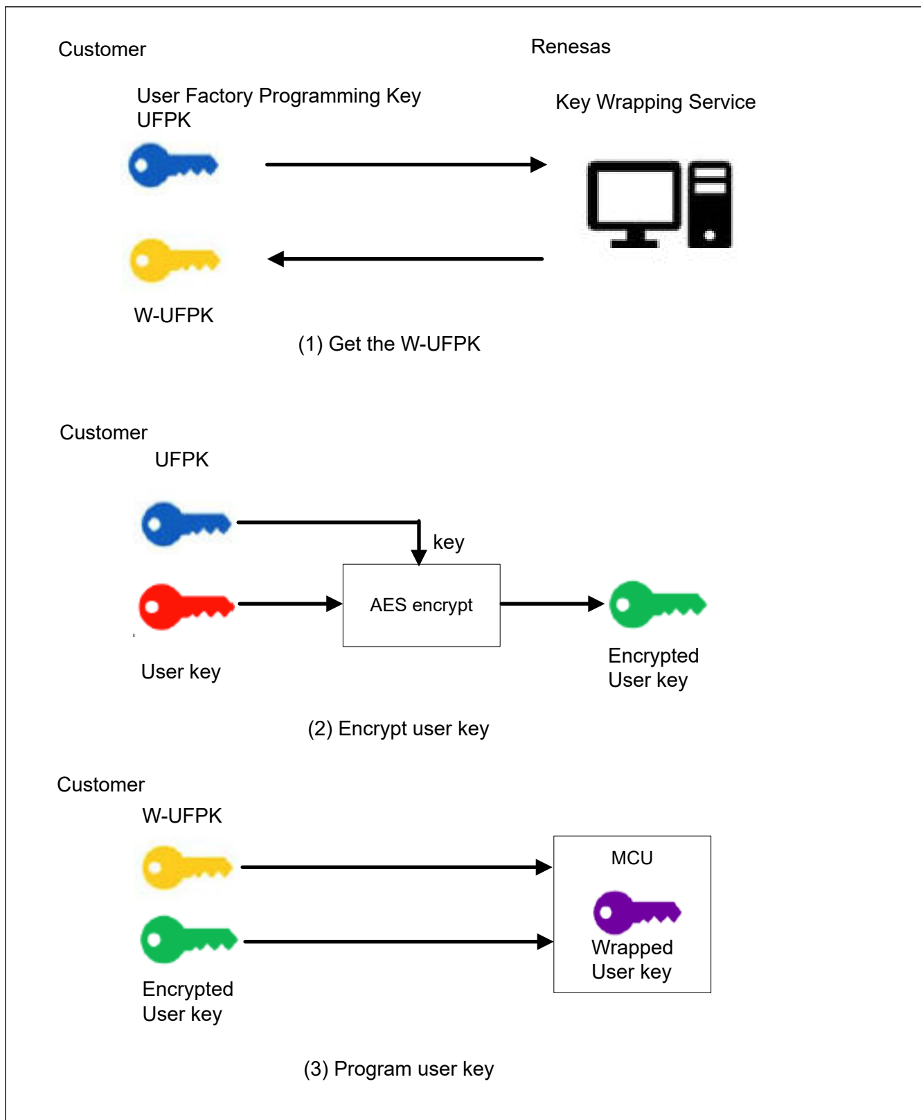
Figure 45.3 Key Injection
