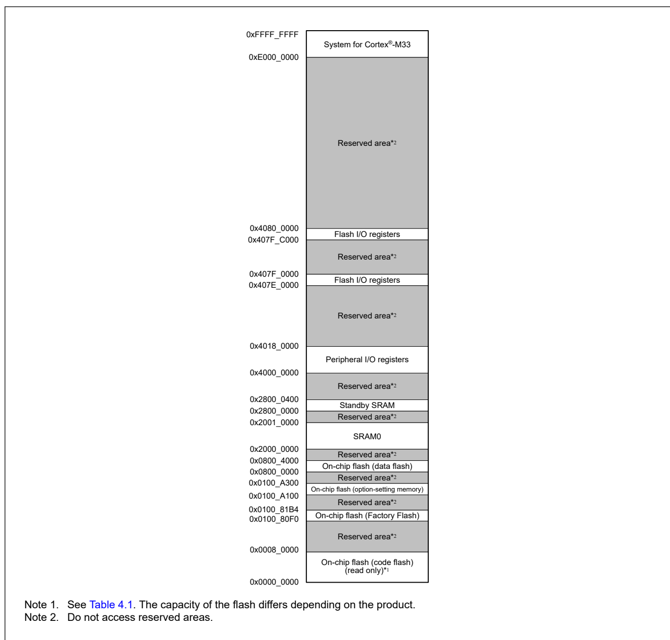
Figure 4.1 Memory map
