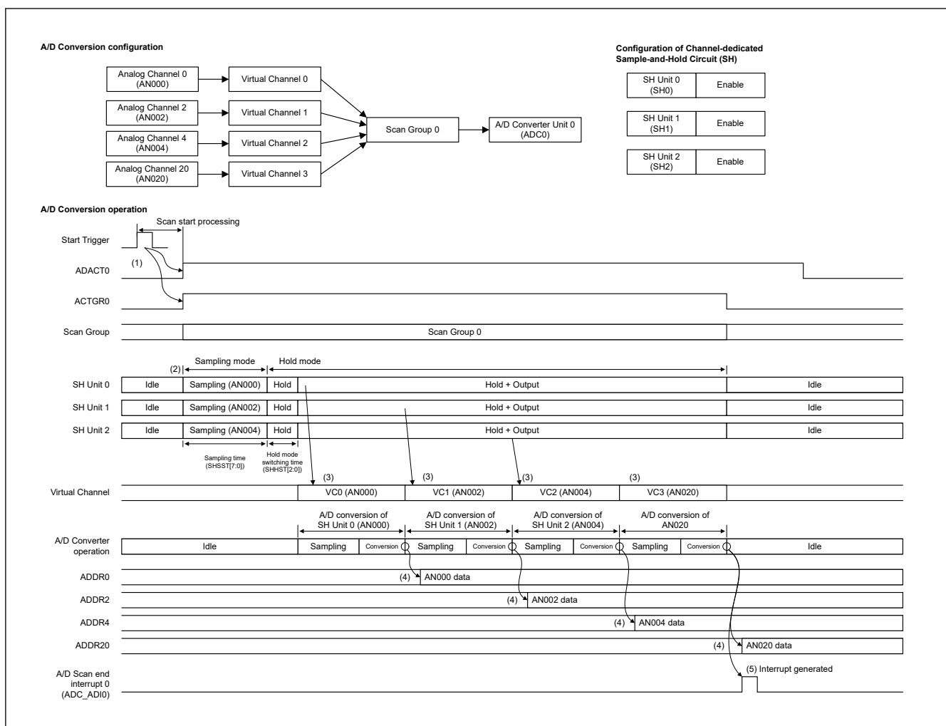
Figure 36.18 Basic operation of channel-dedicated sample-and-hold circuit in SAR mode
