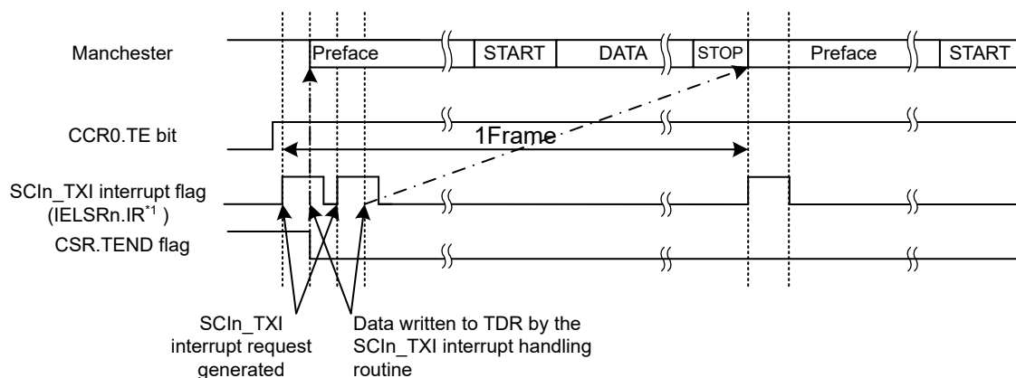
Figure 26.50 Example of Start-of-Transmission Operation for Serial Transmission in Manchester mode (with Preface but Without the CTS Function)
