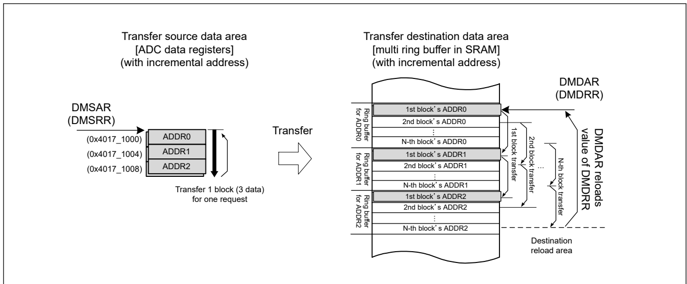
Figure 15.19 Example of Use Case: from Single Block to Multi Ring Buffer
