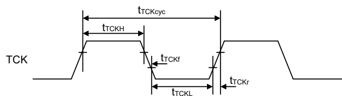
Figure 46.60 Boundary scan TCK timing
