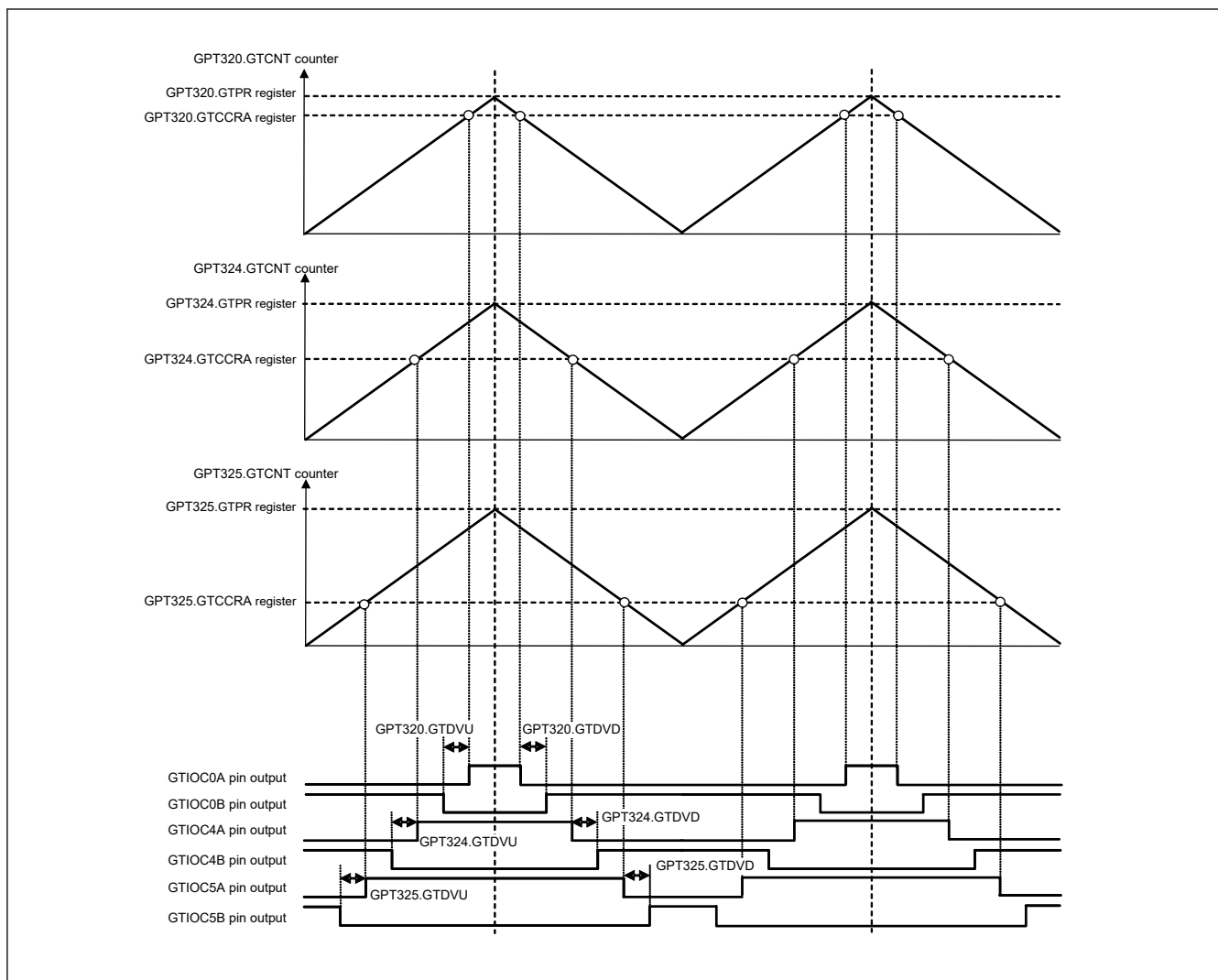
Figure 21.116 Example of 3-phase triangle-wave complementary PWM output with automatic dead time setting
