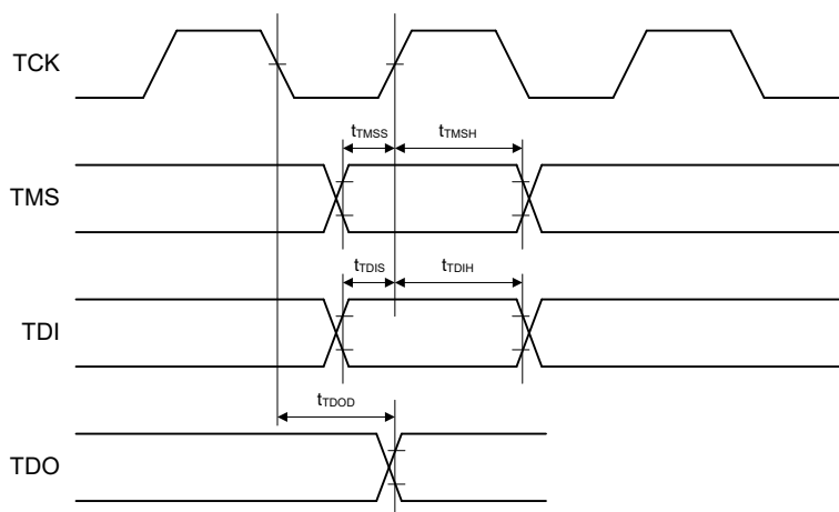
Figure 46.61 Boundary scan input/output timing
