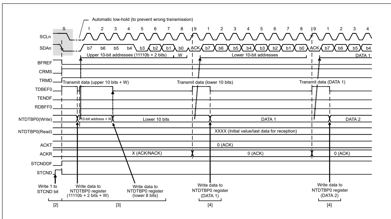
Figure 27.3 Master transmit operation timing (2) (10-bit address format)
