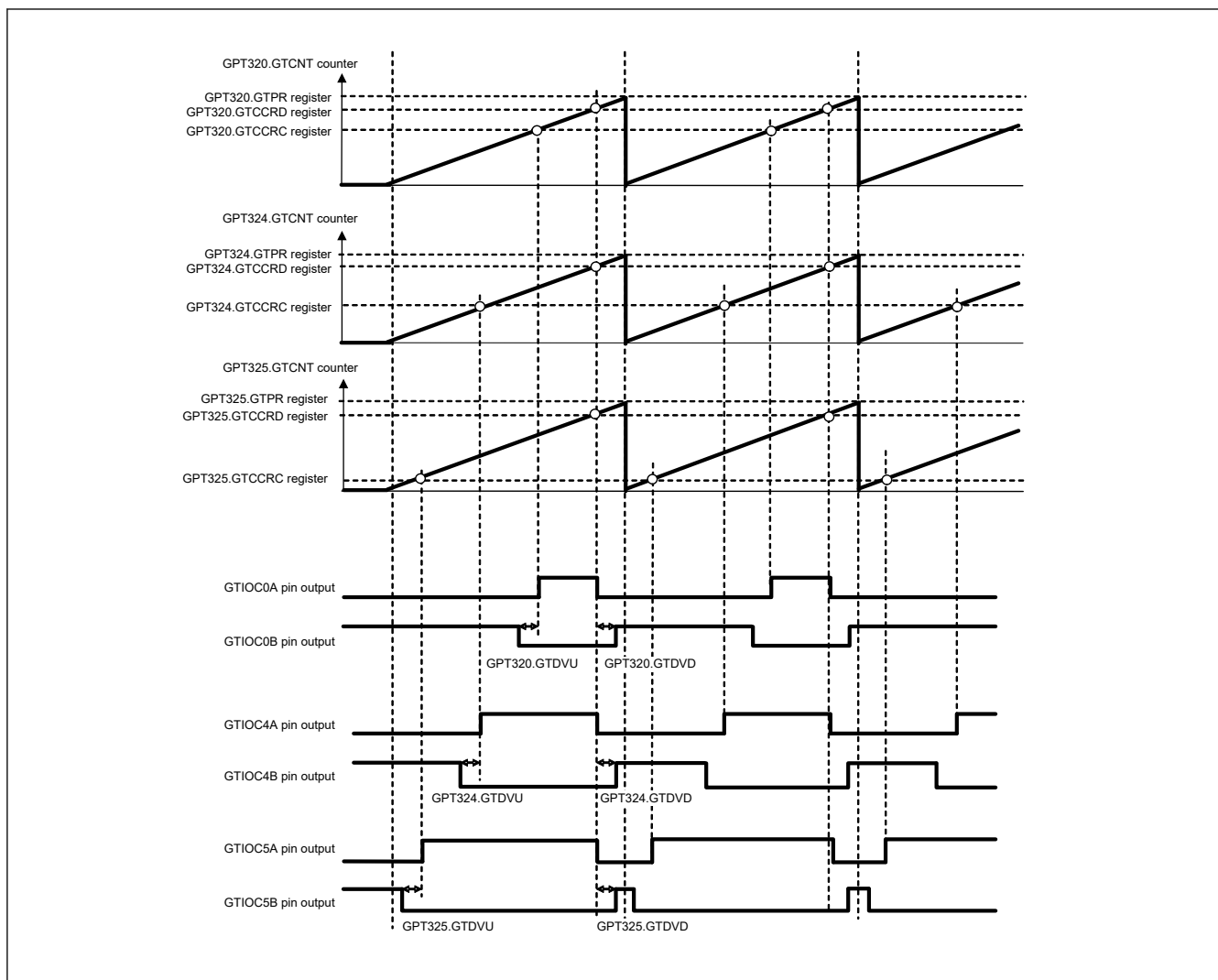
Figure 21.114 Example of 3-phase saw-wave complementary PWM output with automatic dead time setting
