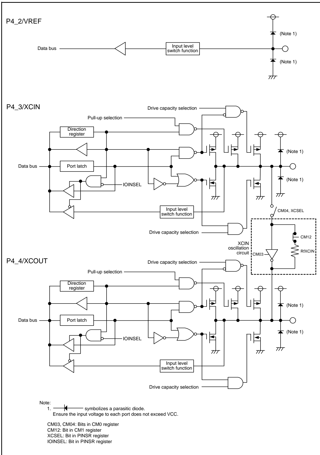
Figure 7.9 Configuration of I/O Ports (9)
