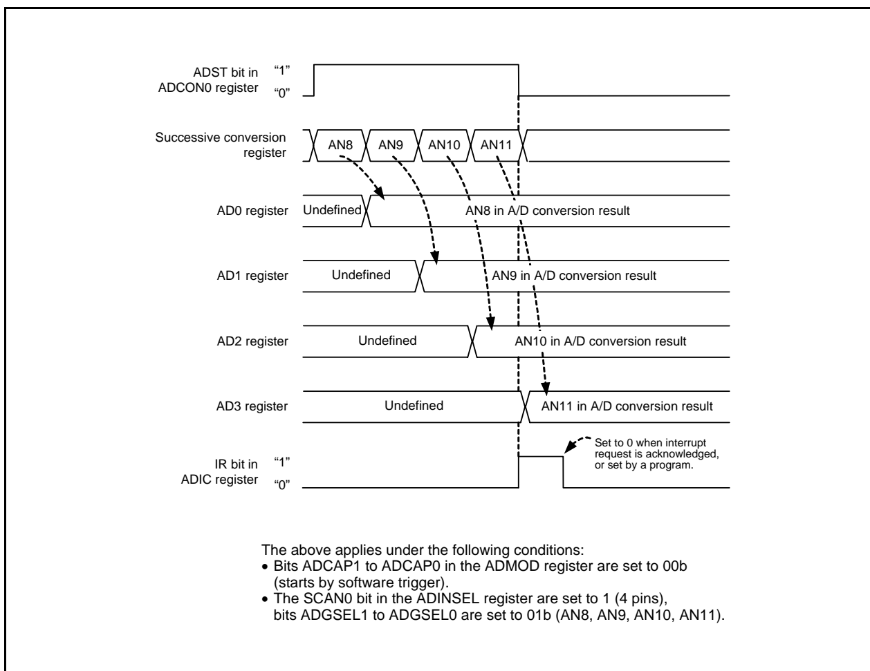
Figure 28.8 Operating Example of Single Sweep Mode
