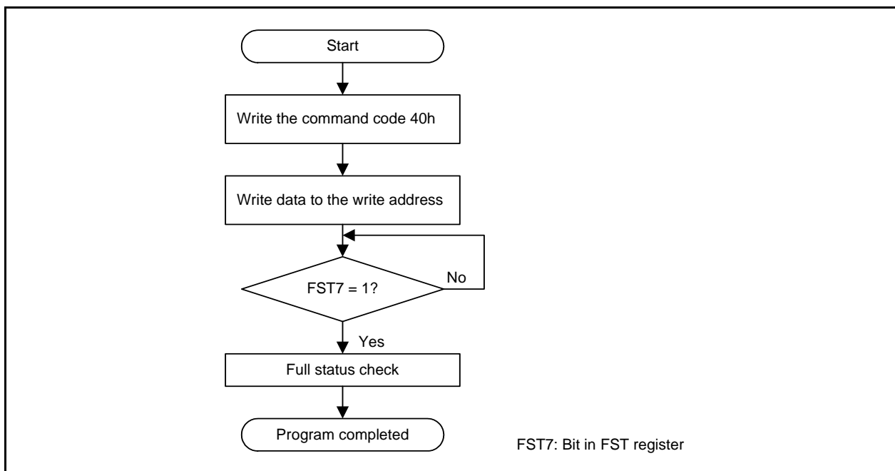
Figure 32.7 Program Flowchart (Flash Ready Status Interrupt Disabled)
