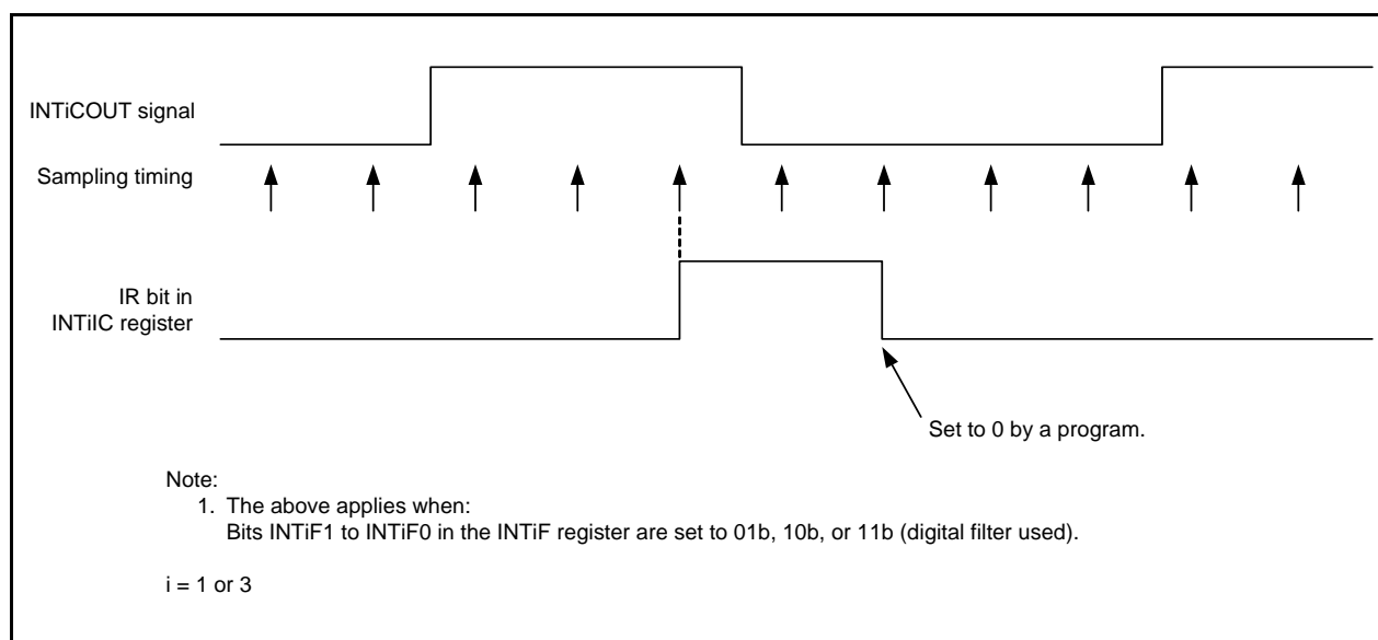
Figure 31.4 Operating Example of Comparator Bi Digital Filter
