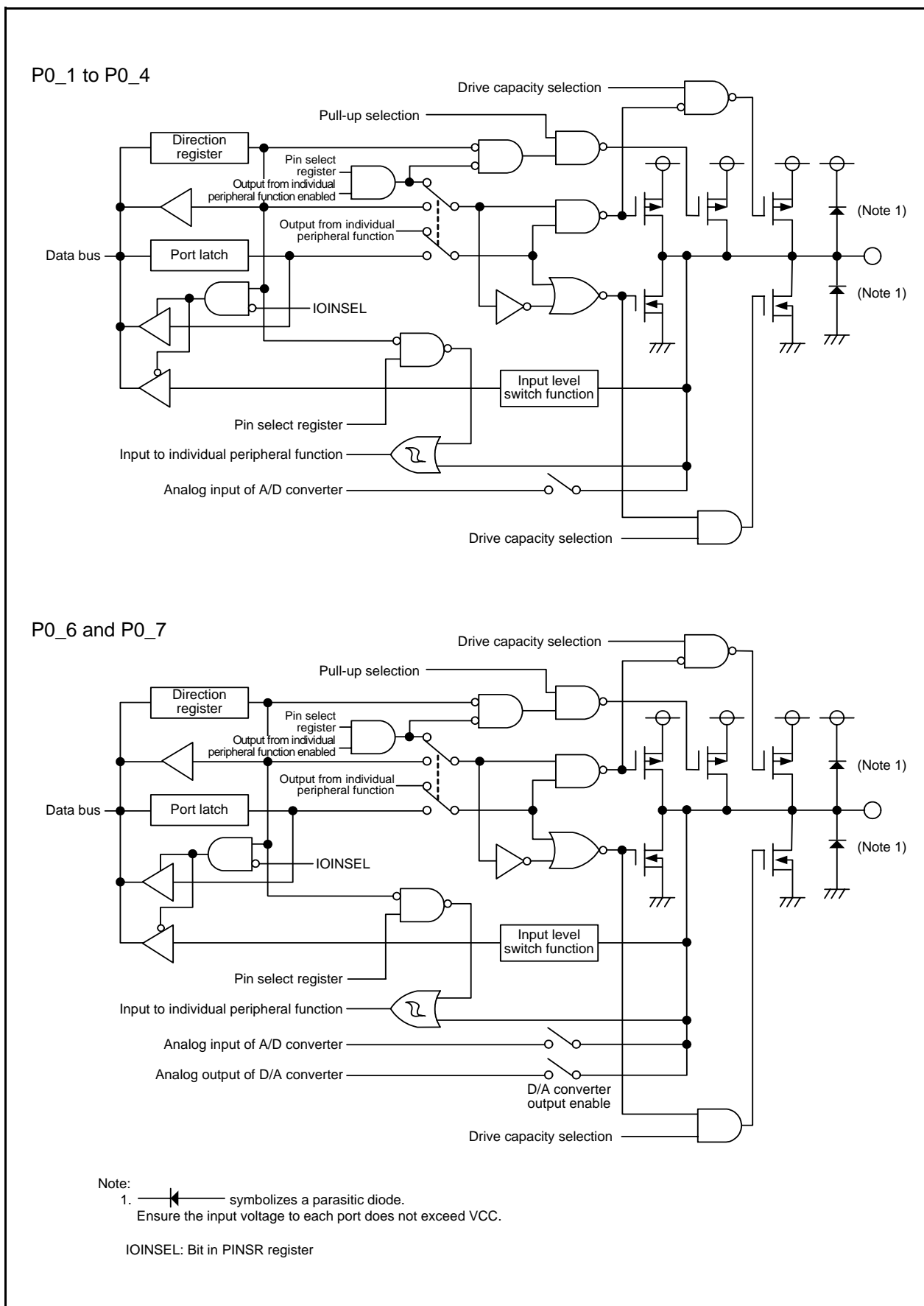
Figure 7.1 Configuration of I/O Ports (1)
