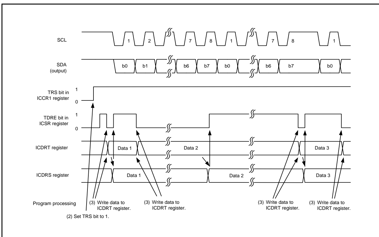
Figure 26.14 Operating Timing in Transmit Mode (Clock Synchronous Serial Mode)
