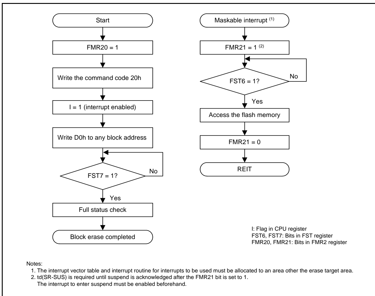
Figure 32.10 Block Erase Flowchart (Flash Ready Status Interrupt Disabled and Suspend Enabled)
