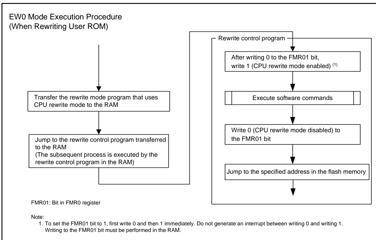
Figure 32.3 How to Set and Exit EW0 Mode
