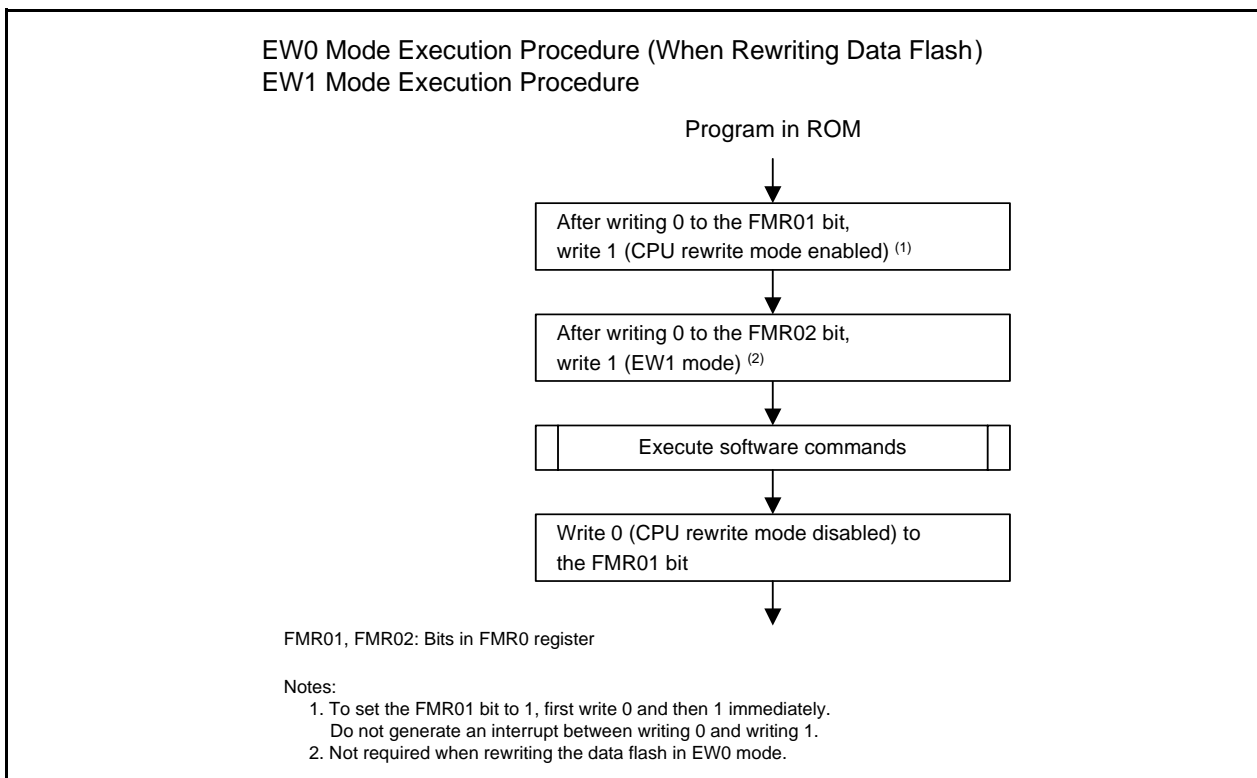
Figure 32.4 How to Set and Exit EW0 Mode (When Rewriting Data Flash) and EW1 Mode
