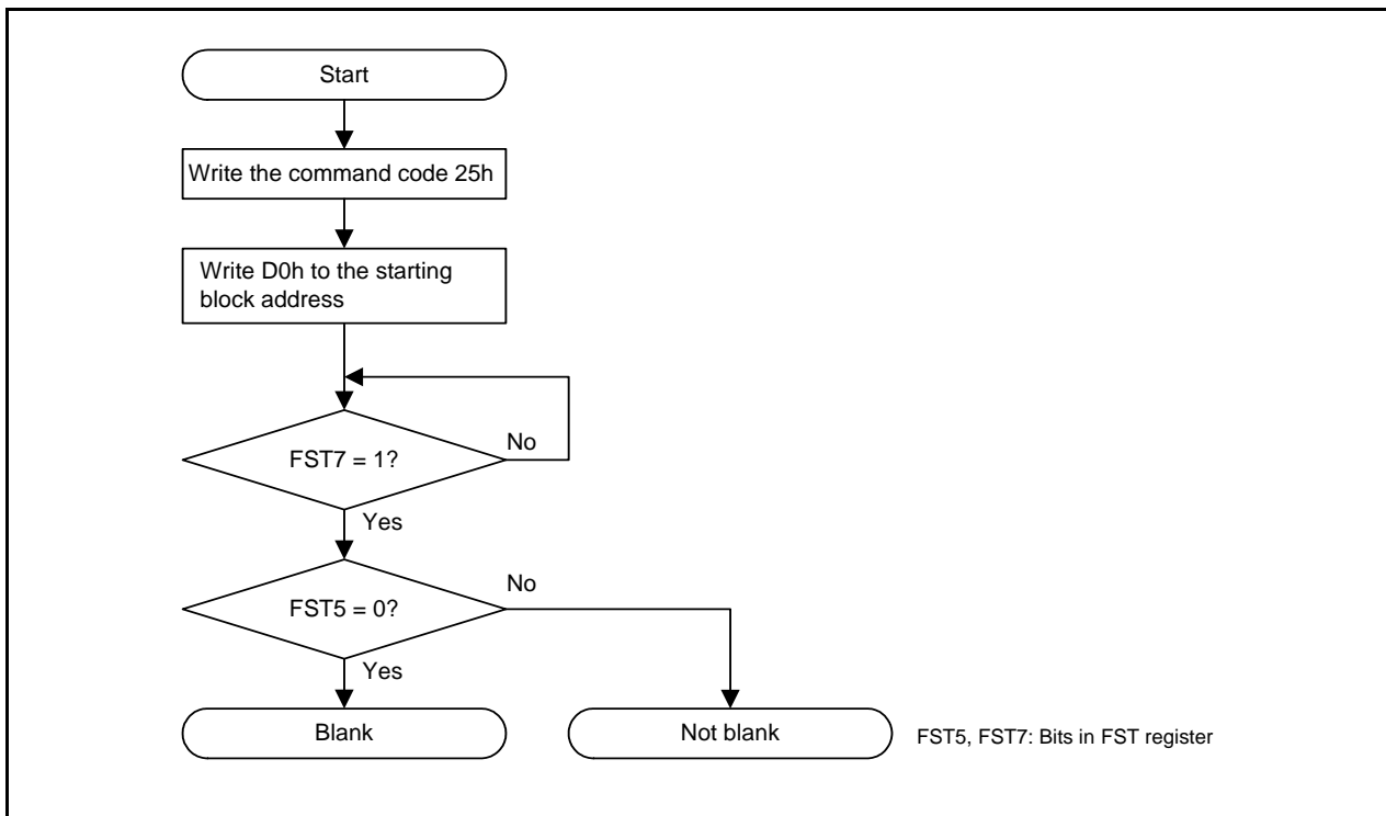
Figure 32.14 Block Blank Check Flowchart
