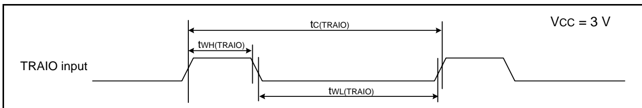
Figure 34.13 TRAIO Input Timing Diagram when V_{CC} = 3\text{ V}
