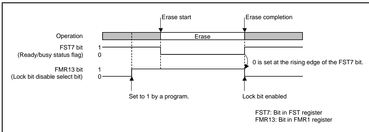
Figure 32.6 FMR13 Bit Operation Timing
