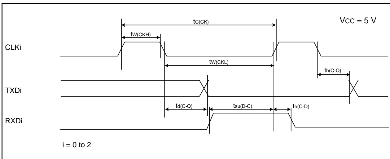
Figure 34.10 Serial Interface Timing Diagram when Vcc = 5 V
