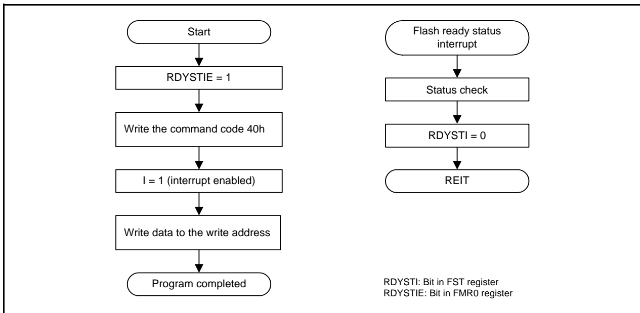
Figure 32.8 Program Flowchart (Flash Ready Status Interrupt Enabled)
