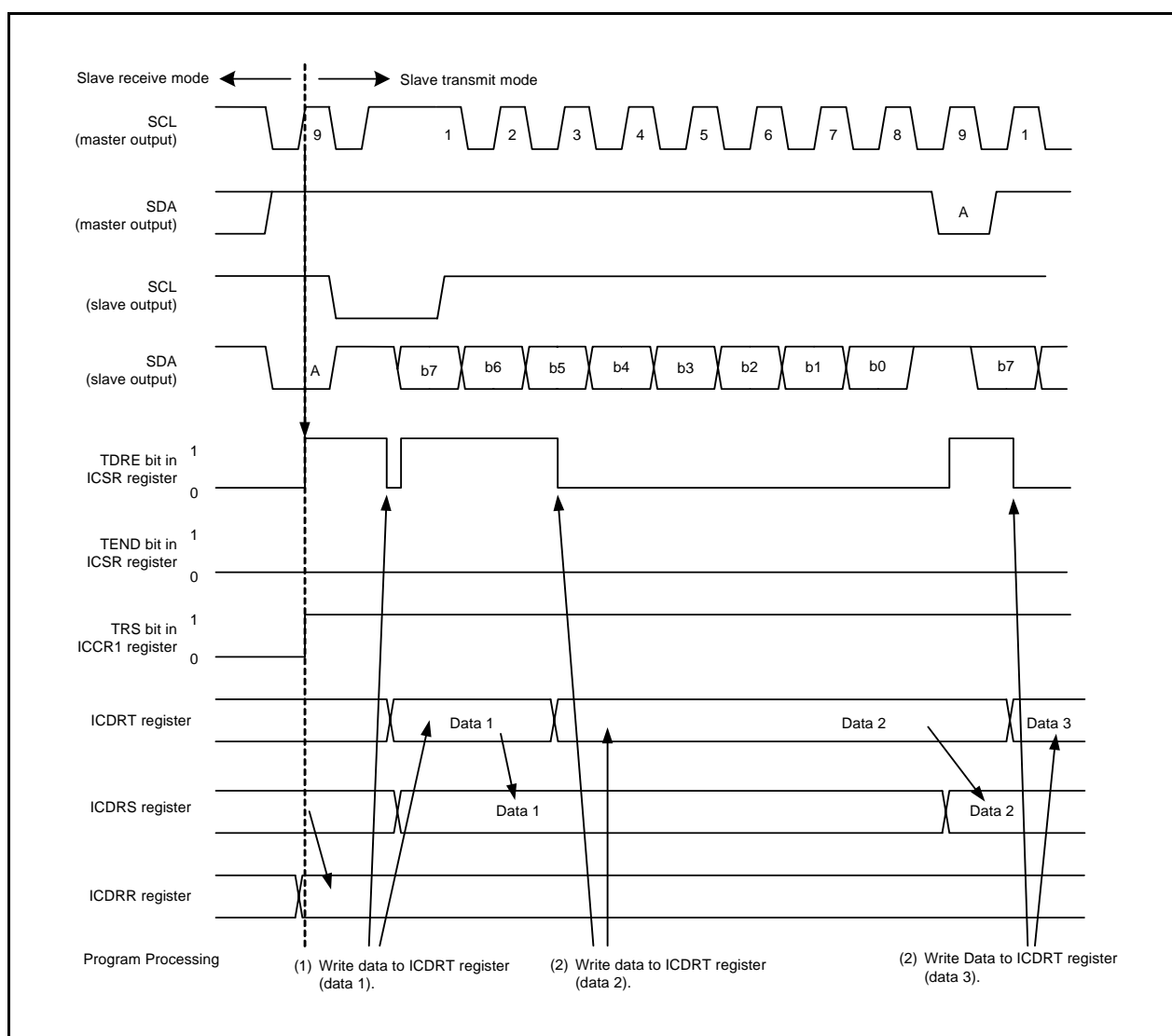
Figure 26.9 Operating Timing in Slave Transmit Mode (I 2 C bus Interface Mode) (1)
