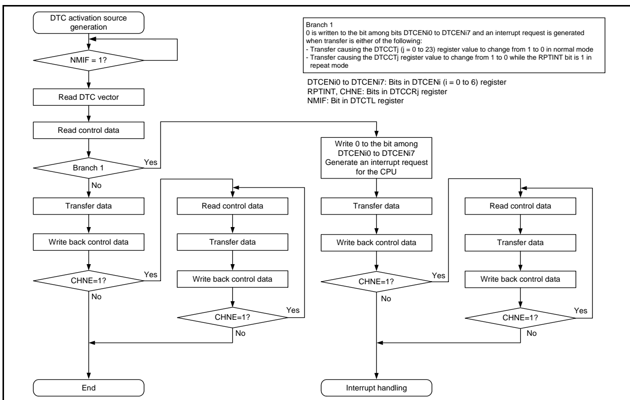
Figure 15.3 DTC Internal Operation Flowchart When DTC Activation Source is not SSU/I²C bus, Timer RC, Timer RD, or Flash Memory Interrupt Source
