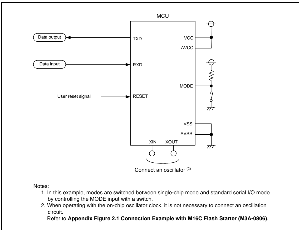
Figure 32.16 Pin Handling in Standard Serial I/O Mode 2
