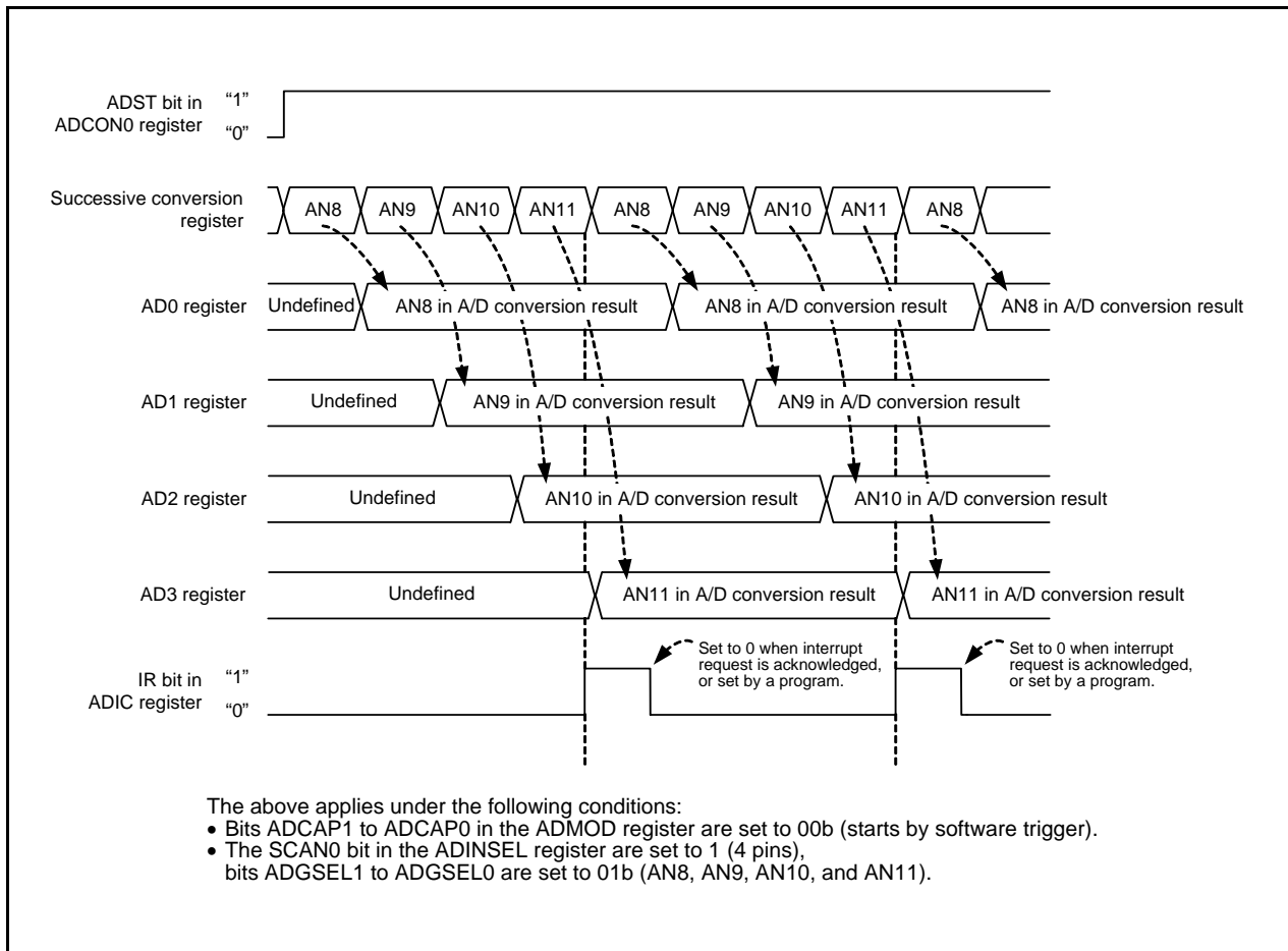
Figure 28.9 Operating Example of Repeat Sweep Mode
