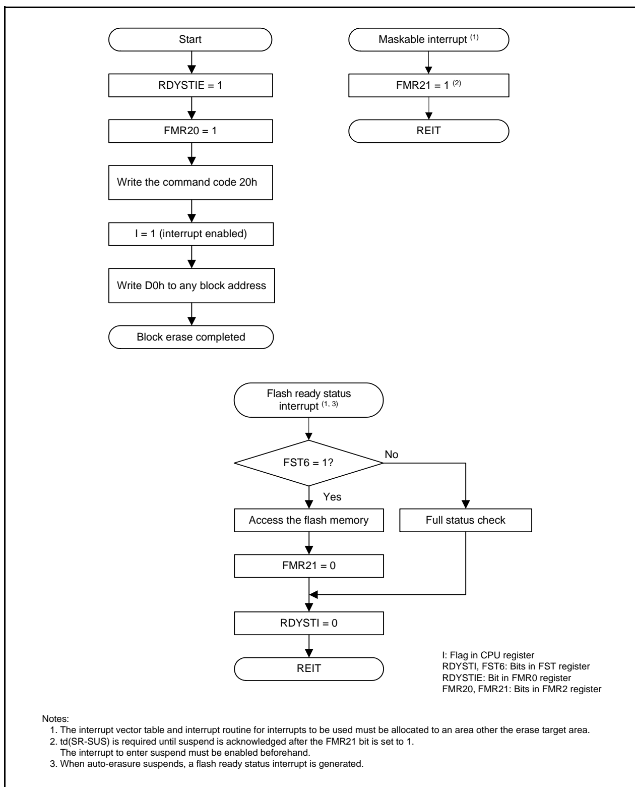
Figure 32.11 Block Erase Flowchart (Flash Ready Status Interrupt Enabled and Suspend Enabled)
