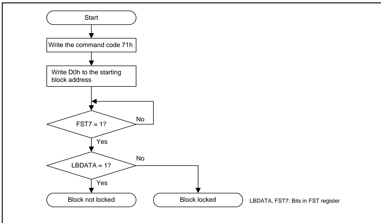
Figure 32.13 Read Lock Bit Status Flowchart
