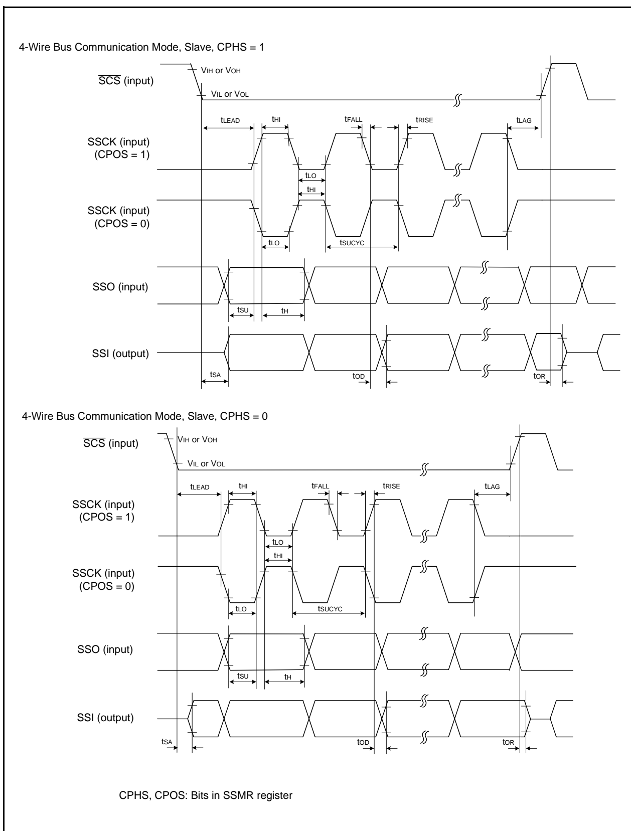
Figure 34.5 I/O Timing of Clock Synchronous Serial I/O with Chip Select (Slave)
