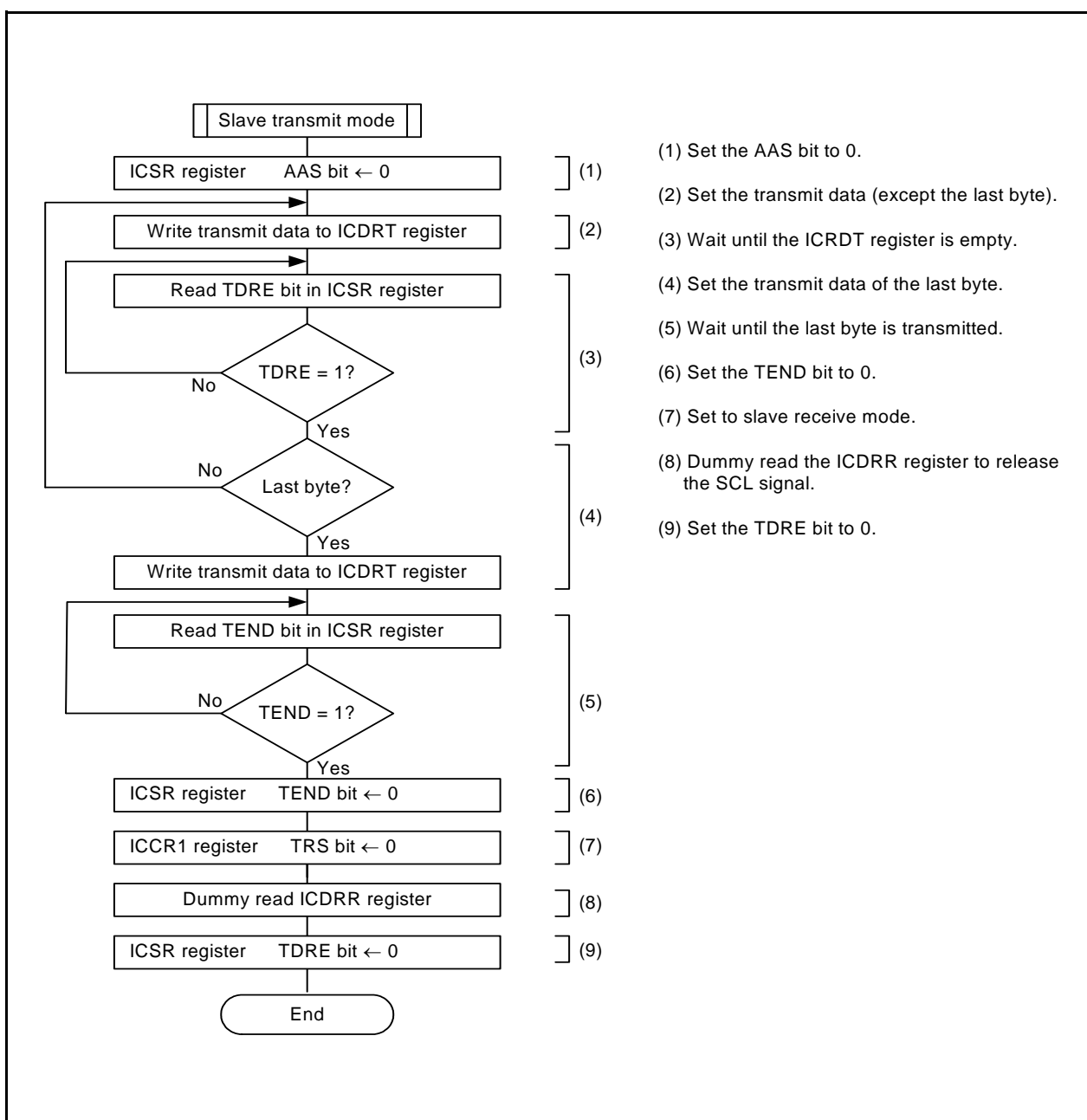
Figure 26.18 Register Setting Example in Slave Transmit Mode (I 2 C bus Interface Mode)
