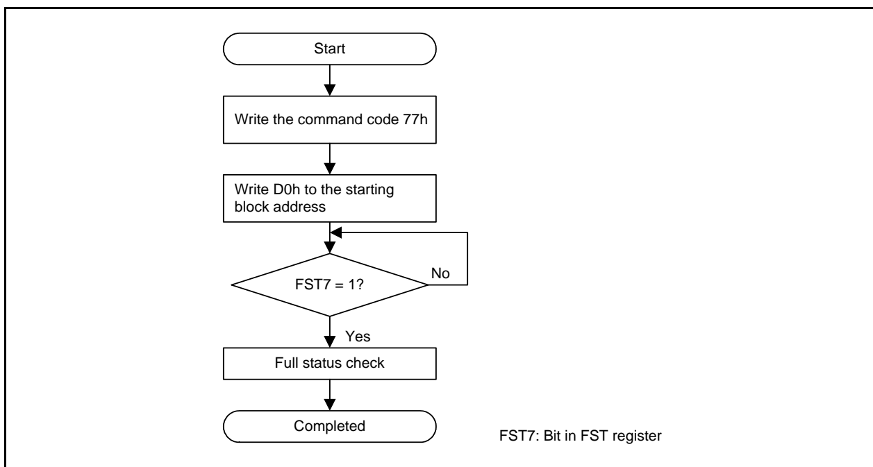
Figure 32.12 Lock Bit Program Flowchart
