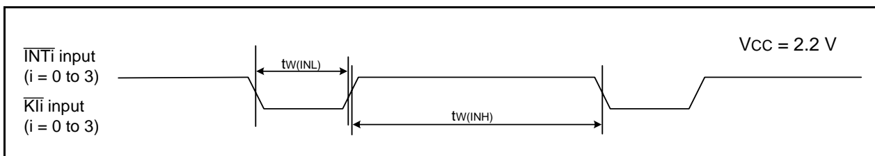
Figure 34.19 Input Timing for External Interrupt \overline{INTi} and Key Input Interrupt \overline{Kli} when Vcc = 2.2 V
