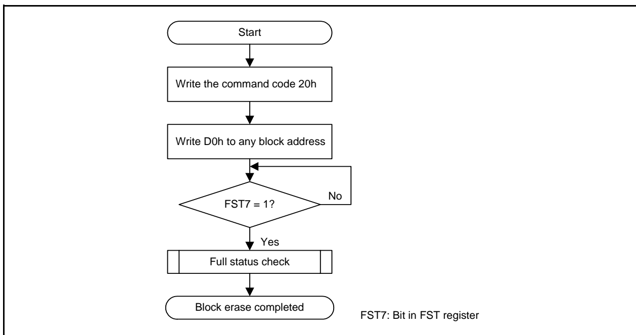
Figure 32.9 Block Erase Flowchart (Flash Ready Status Interrupt Disabled)
