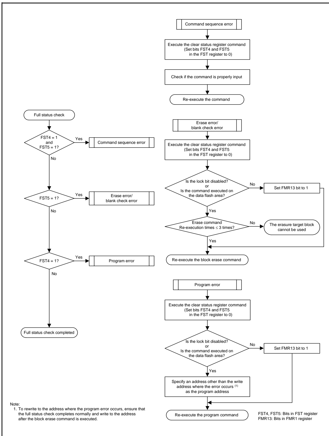
Figure 32.15 Full Status Check and Handling Procedure for Individual Errors
