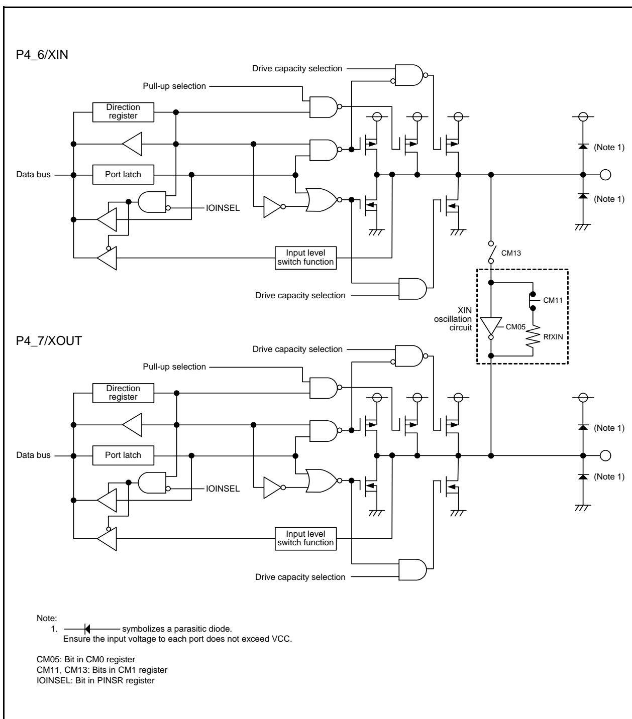
Figure 7.11 Configuration of I/O Ports (11)
