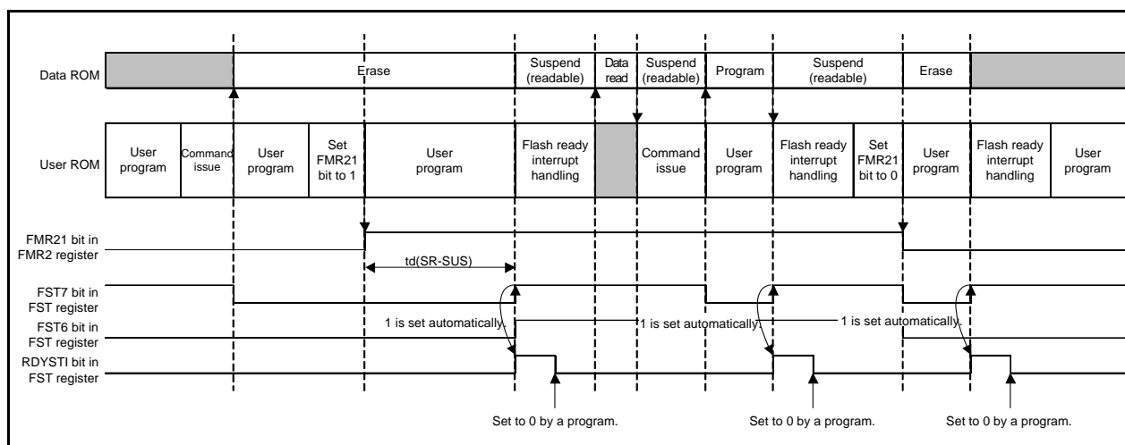
Figure 32.2 Suspend Operation Timing
