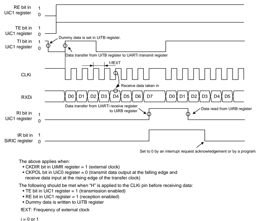
Figure 22.3 Transmit and Receive Timing in Clock Synchronous Serial I/O Mode
