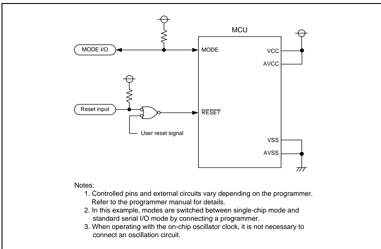
Figure 32.17 Pin Handling in Standard Serial I/O Mode 3
