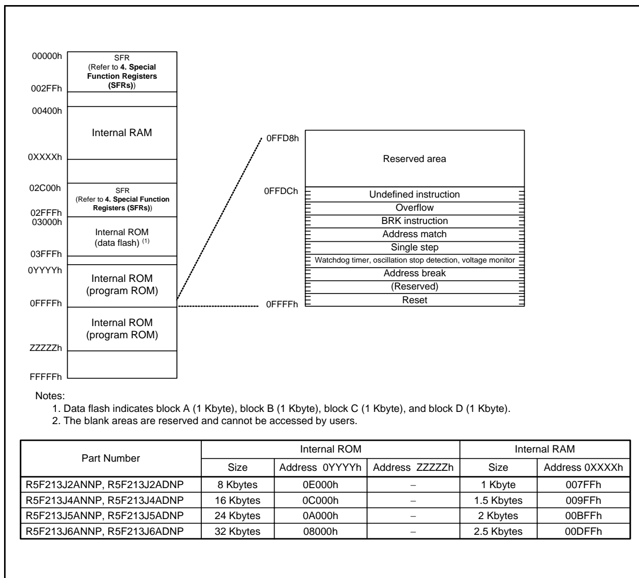
Figure 3.1 Memory Map of R8C/3JA Group
