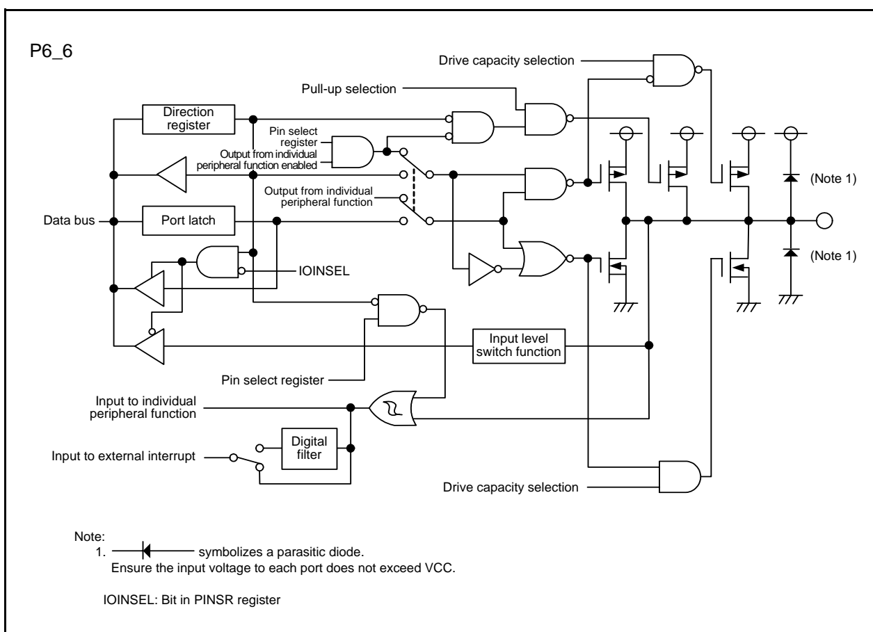
Figure 7.12 Configuration of I/O Ports (12)
