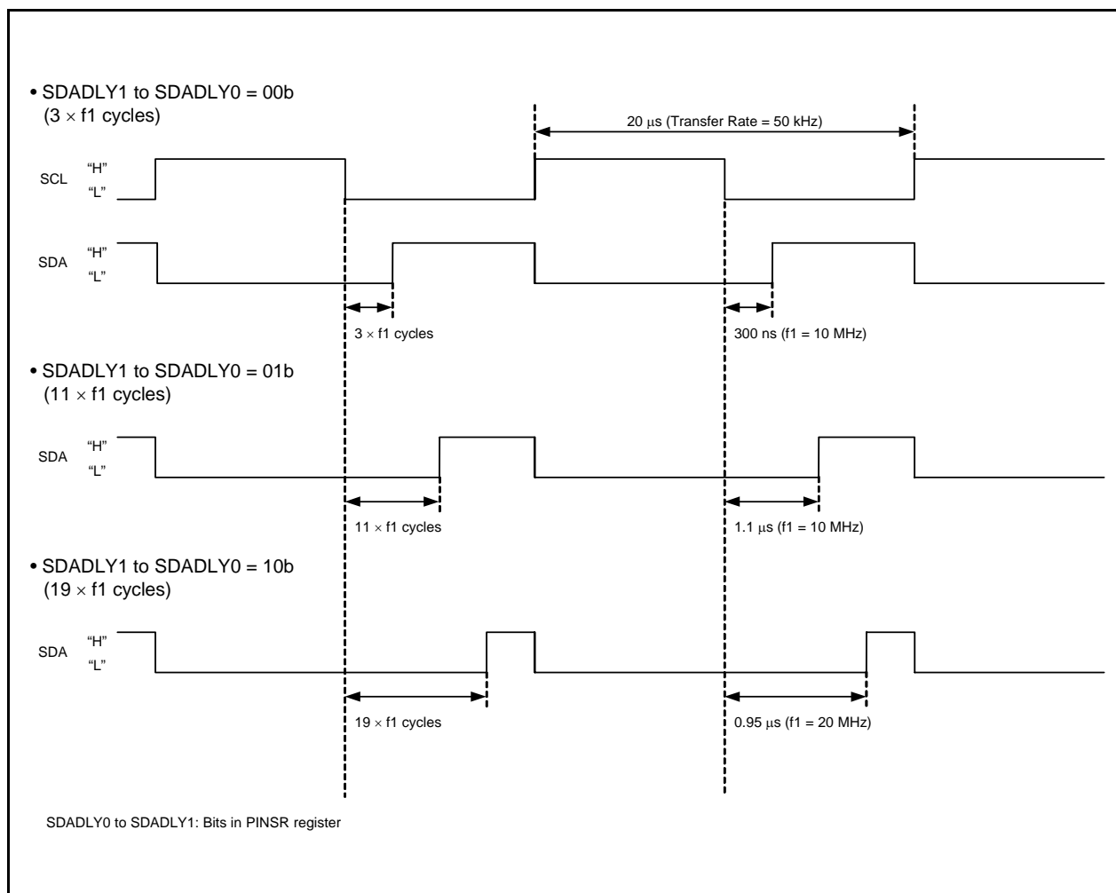
Figure 26.3 Operating Example of Digital Delay for SDA Pin
