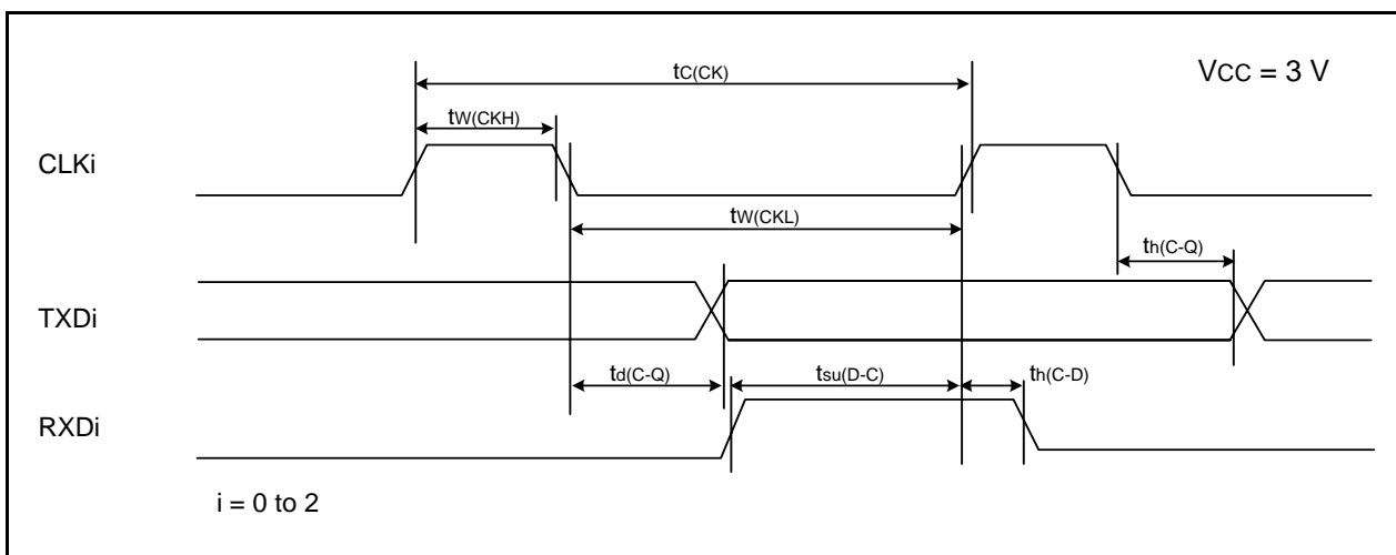
Figure 34.14 Serial Interface Timing Diagram when V_{cc} = 3\text{ V}
