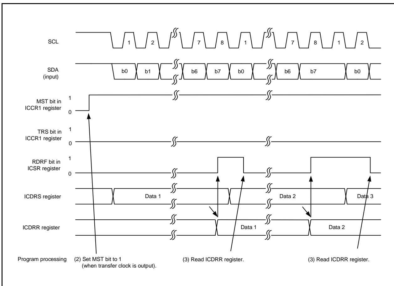
Figure 26.15 Operating Timing in Receive Mode (Clock Synchronous Serial Mode)
