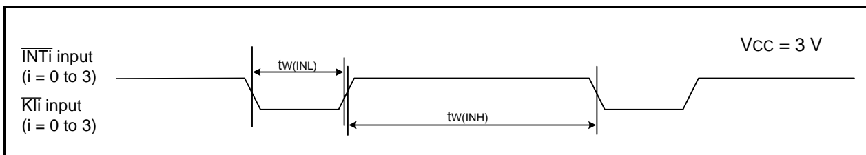
Figure 34.15 Input Timing for External Interrupt \overline{INTi} and Key Input Interrupt \overline{Kli} when V_{cc} = 3\text{ V}
