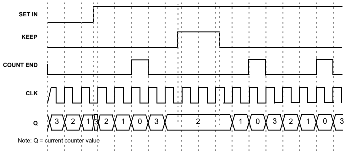
Figure 50: CNT/FSM Timing Diagram (Set Rising Edge Mode, Oscillator is Forced On, UP = 0) for Counter Data = 3
