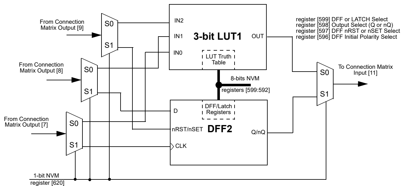
Figure 30: 3-bit LUT1 or DFF2
