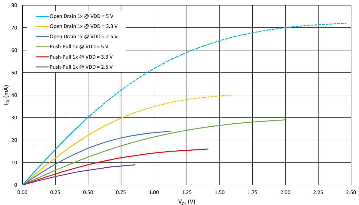
Figure 19: Typical Low Level Output Current vs. Low Level Output Voltage, 1x Drive at T = 25^\circ\text{C} , Full Range
