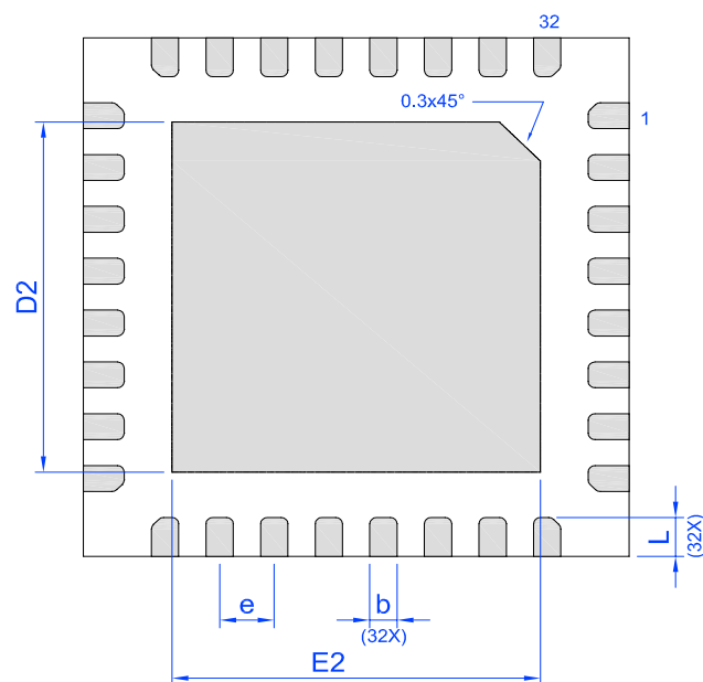
BTM View
