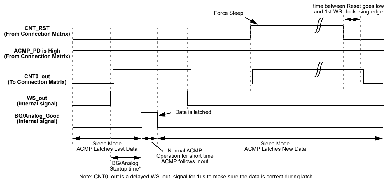
Figure 59: Wake/Sleep Timing Diagram, Short Wake Mode, Counter Set is Used
