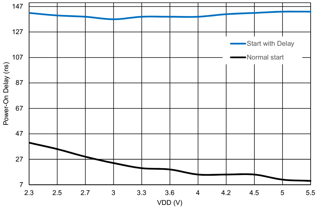
Figure 88: Oscillator2 Maximum Power-On Delay vs. V_{DD} at T = 25^{\circ}\text{C} , \text{OSC2} = 25\text{ MHz}
