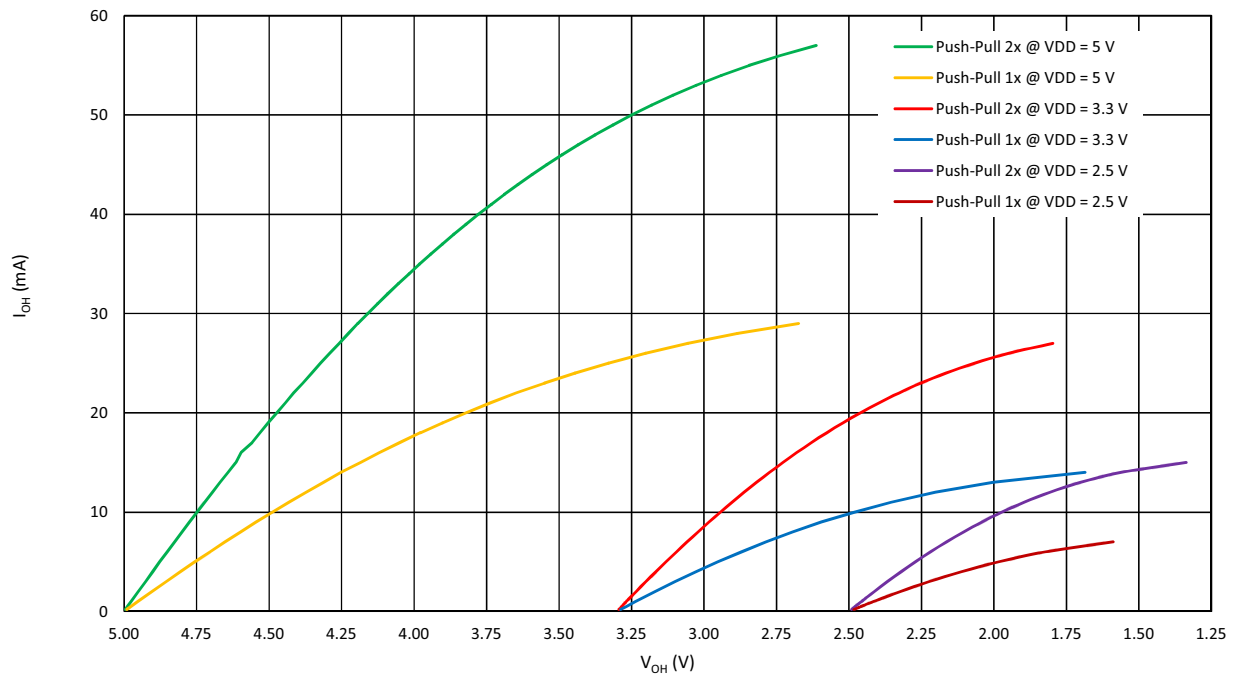
Figure 18: Typical High Level Output Current vs. High Level Output Voltage at T = 25^\circ\text{C}
