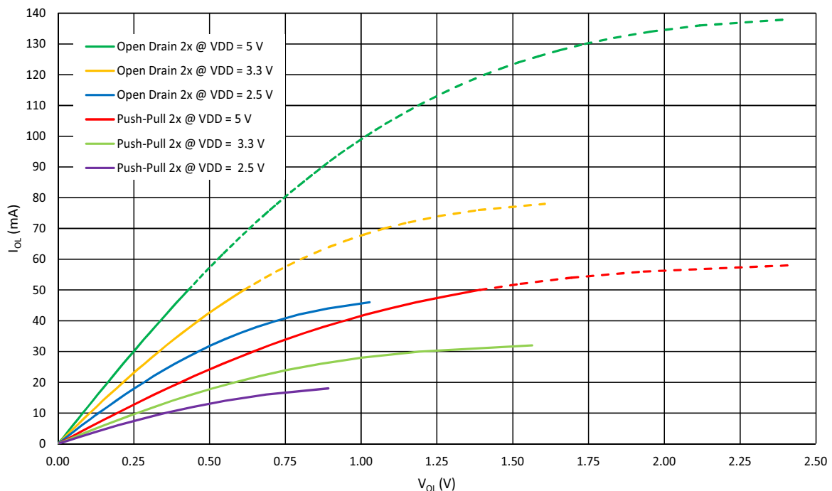
Figure 21: Typical Low Level Output Current vs. Low Level Output Voltage, 2x Drive at T = 25 °C, Full Range
