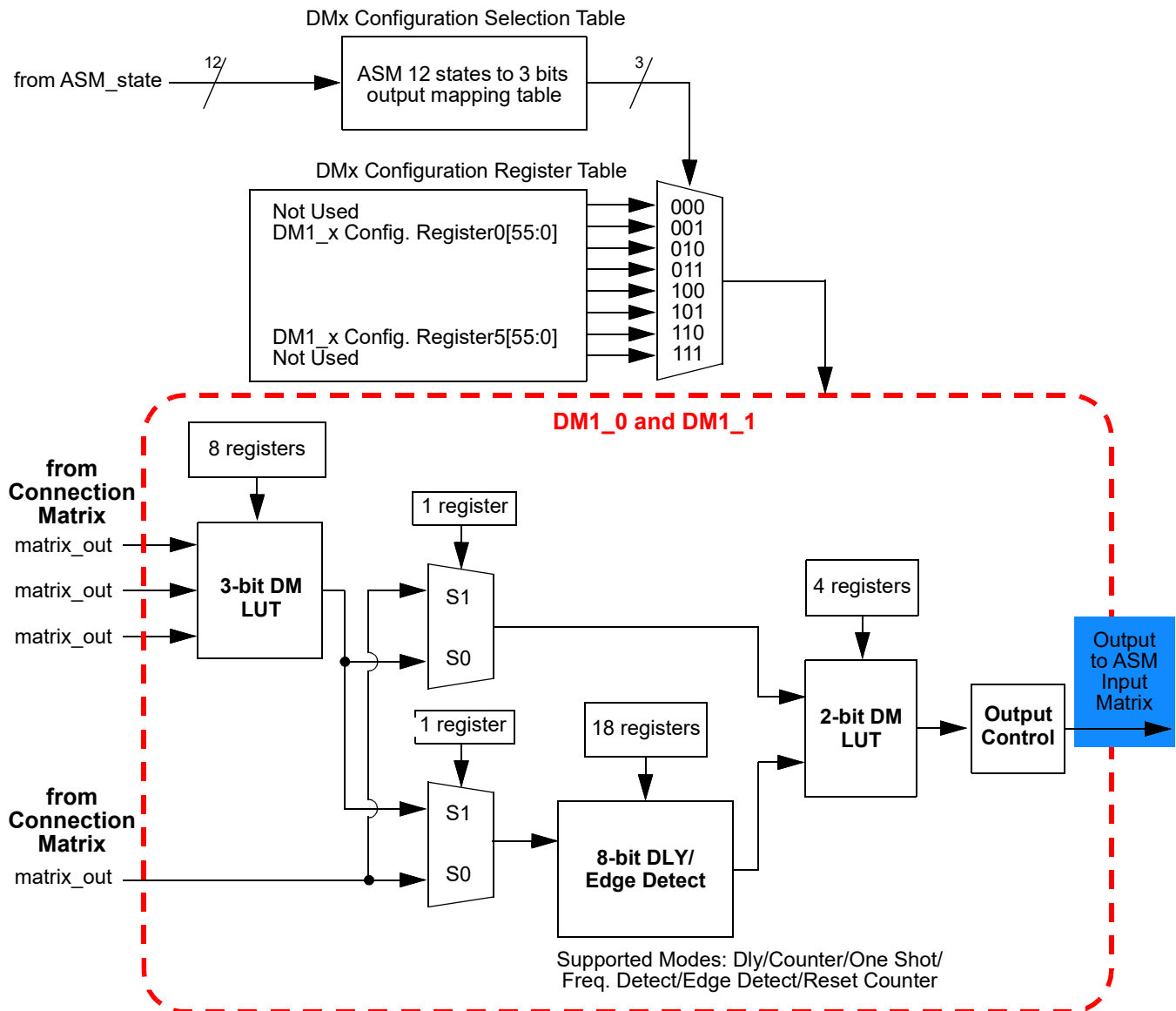
Figure 124: DM1_0/DM1_1 Outputs
