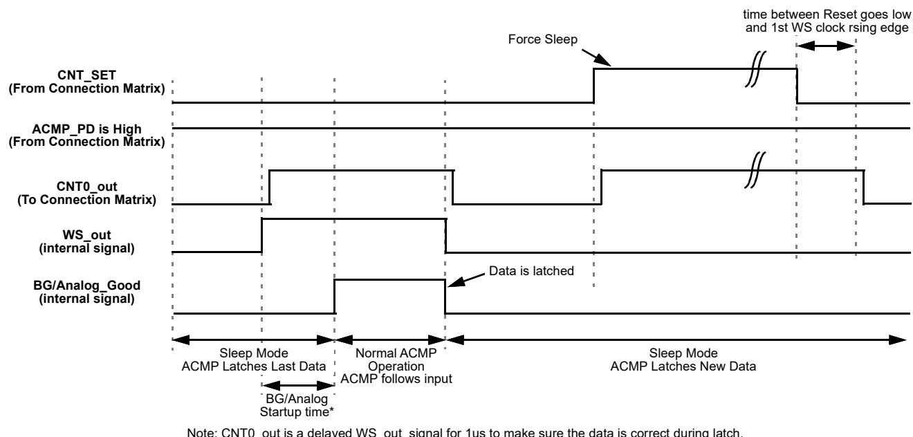
Figure 58: Wake/Sleep Timing Diagram, Normal Wake Mode, Counter Set is Used
