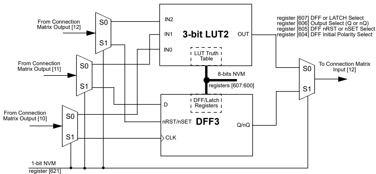
Figure 31: 3-bit LUT2 or DFF3
