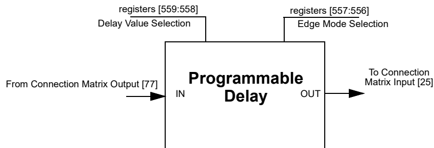
Figure 71: Programmable Delay
