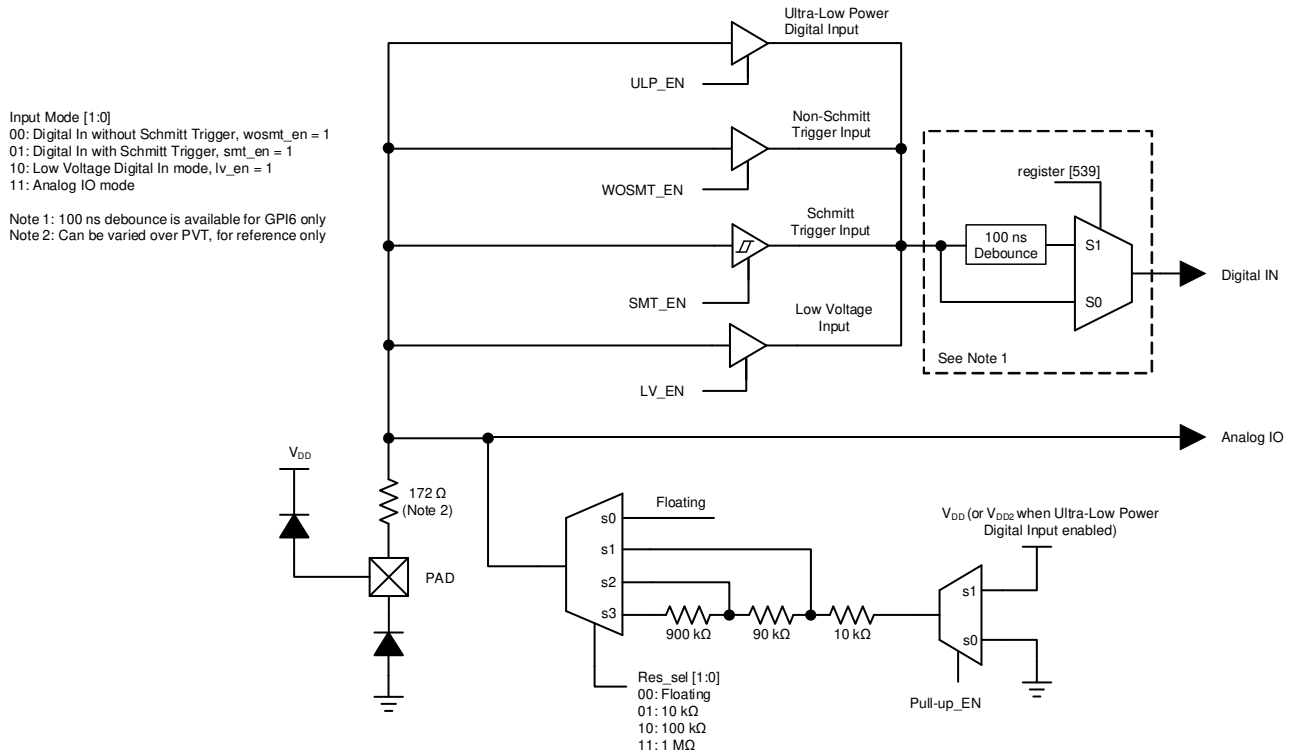
Figure 6: SLG46881 GPI IO Structure Diagram
