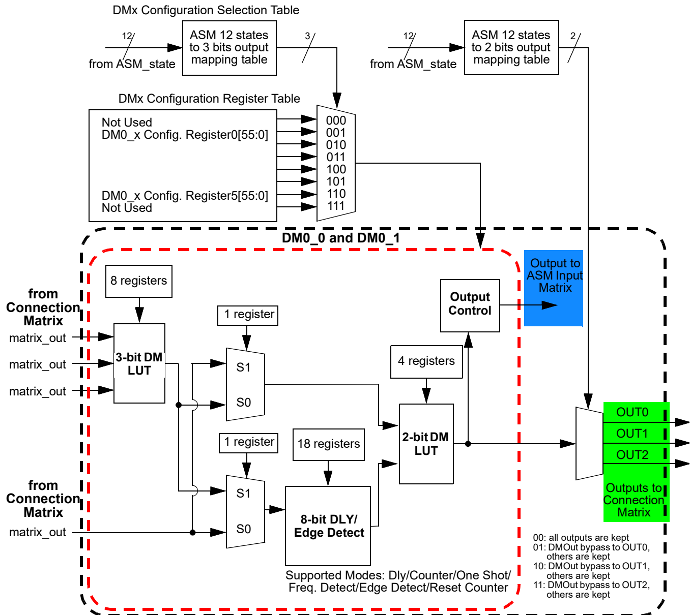
Figure 123: DM0_0/DM0_1 Outputs
