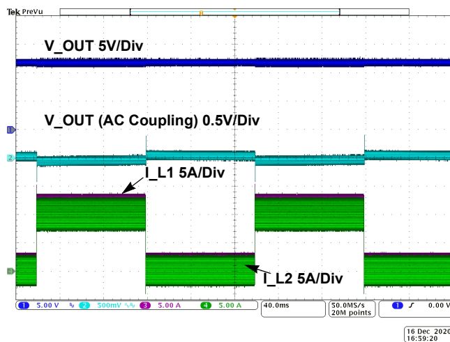
Figure 24. Dual-Phase Waveforms, V_{IN} = 48V , I_{OUT} = 0A-20A Dynamic, CCM Mode
