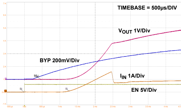
FIGURE 29. Soft-Start with BYP\ CAP = 1.9\mu F and EN to V_{OUT} Delay with VCCX\ CAP = 0.1\mu F , V_{IN} = 6.5V , V_{OUT} = 5V , R_L = 5\Omega , C_{OUT} = 220\mu F , ROCP = 300\Omega
