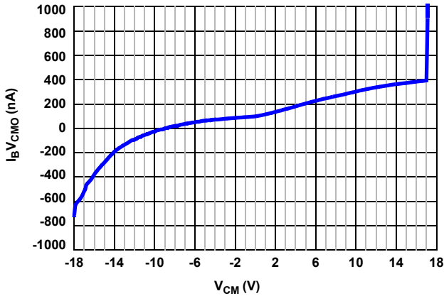
FIGURE 24. I_{BV_{CM0}} vs INPUT COMMON-MODE VOLTAGE
