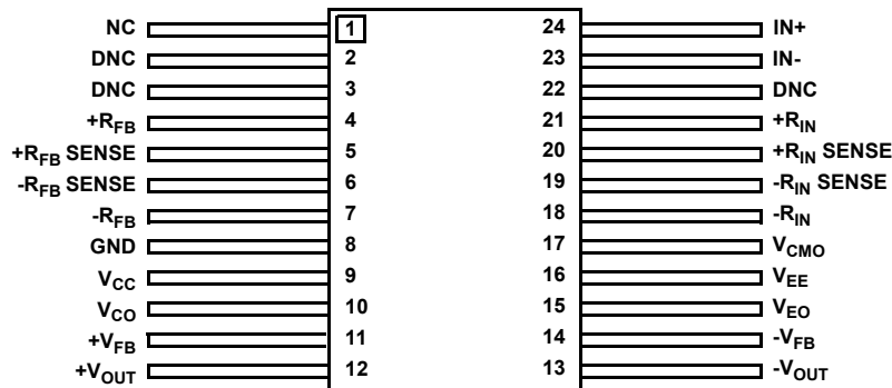
ISL70617SEH (24 LD FLATPACK) TOP VIEW
