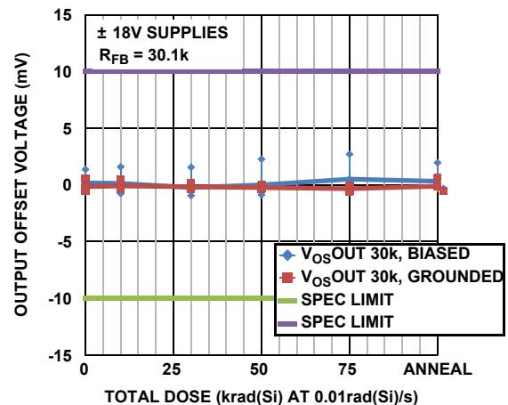
FIGURE 14. V_{OSOUT} (GAIN = 1) vs TOTAL DOSE
