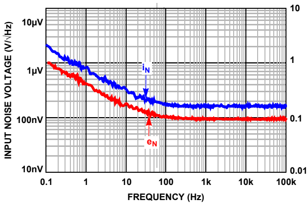
FIGURE 40. INPUT VOLTAGE AND CURRENT NOISE
