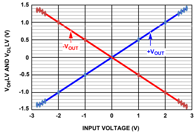
FIGURE 25. V_{OHLV} AND V_{O0LV}
