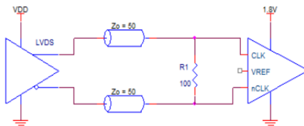
Figure 3. Differential Input Driven by an LVDS Driver – DC Coupling
