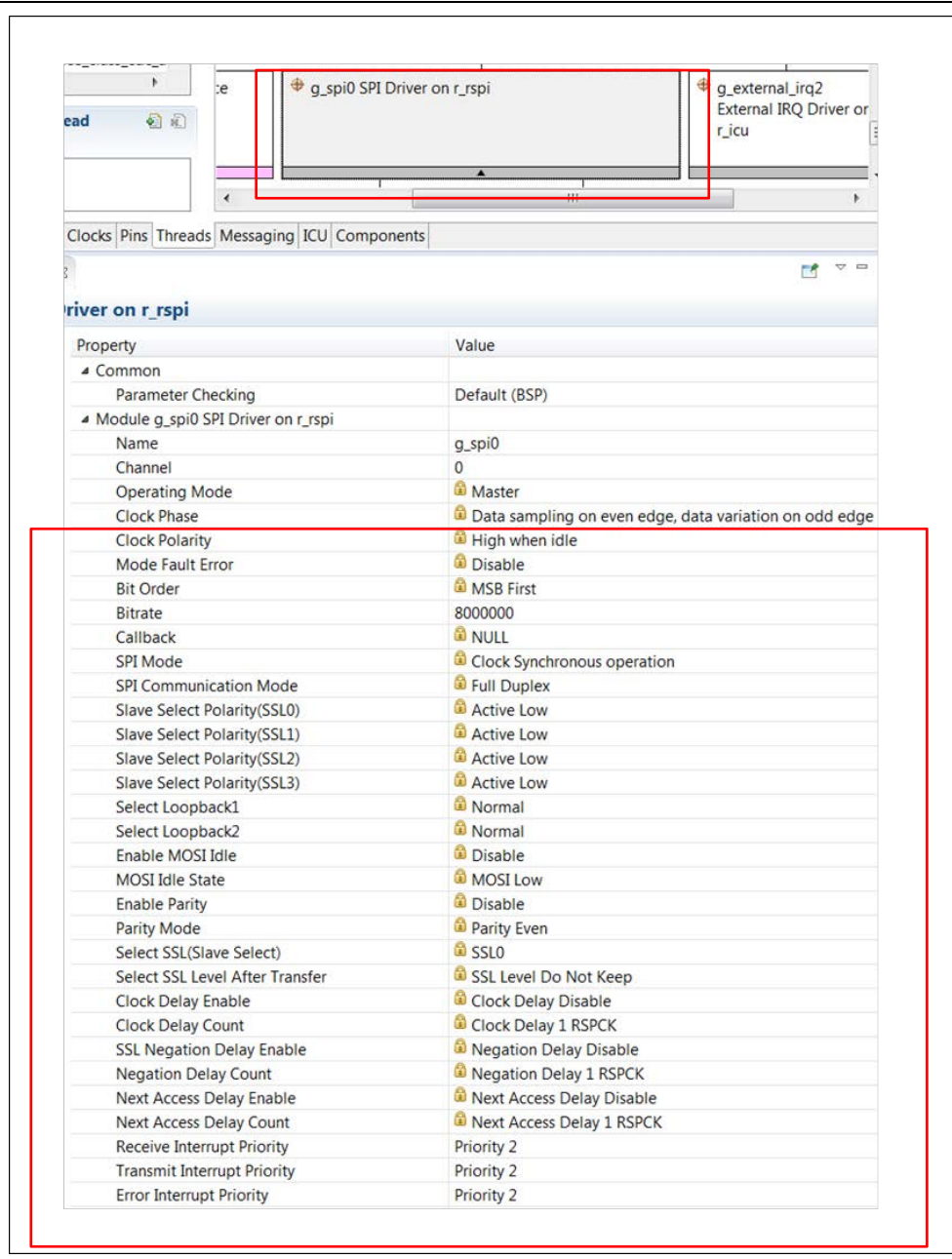
Figure 48. R_SPI configuration
