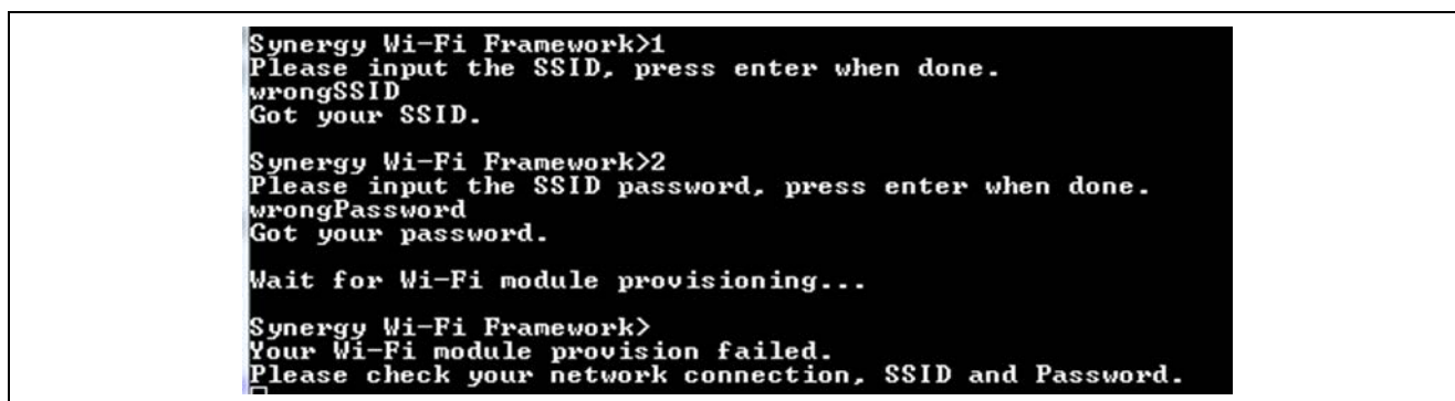
Figure 60. Provision failed
