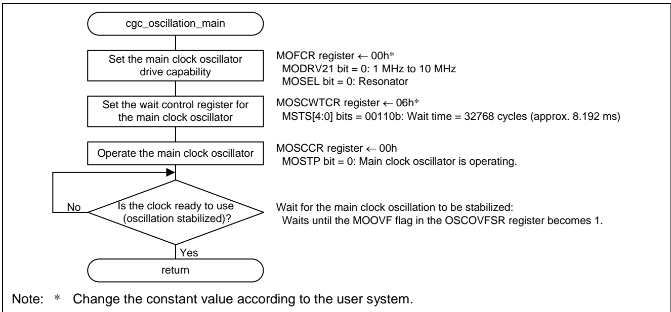
Figure 4.7 Main Clock Oscillation Setting
