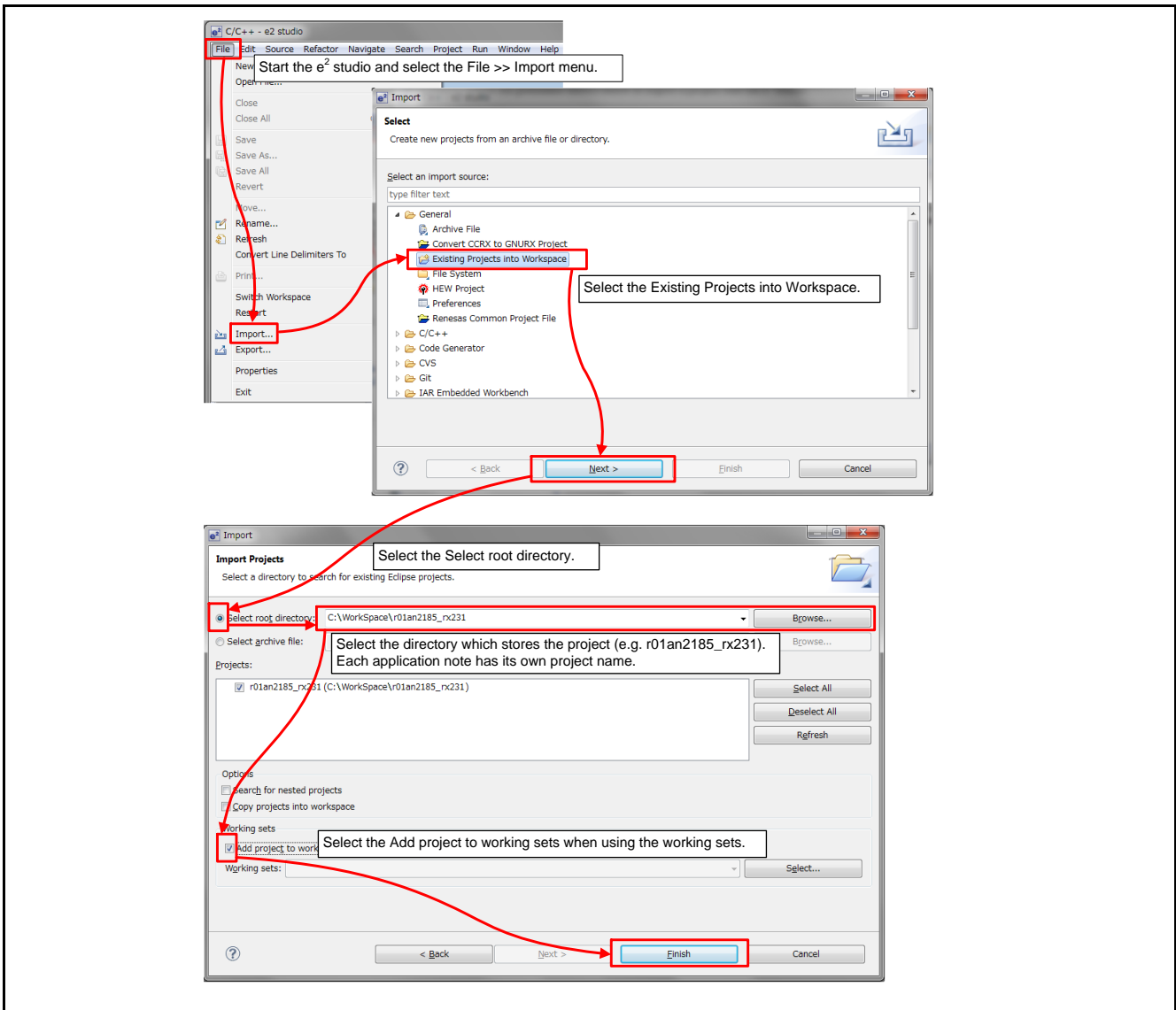
Figure 5.1 Importing a Project in the e 2 studio
