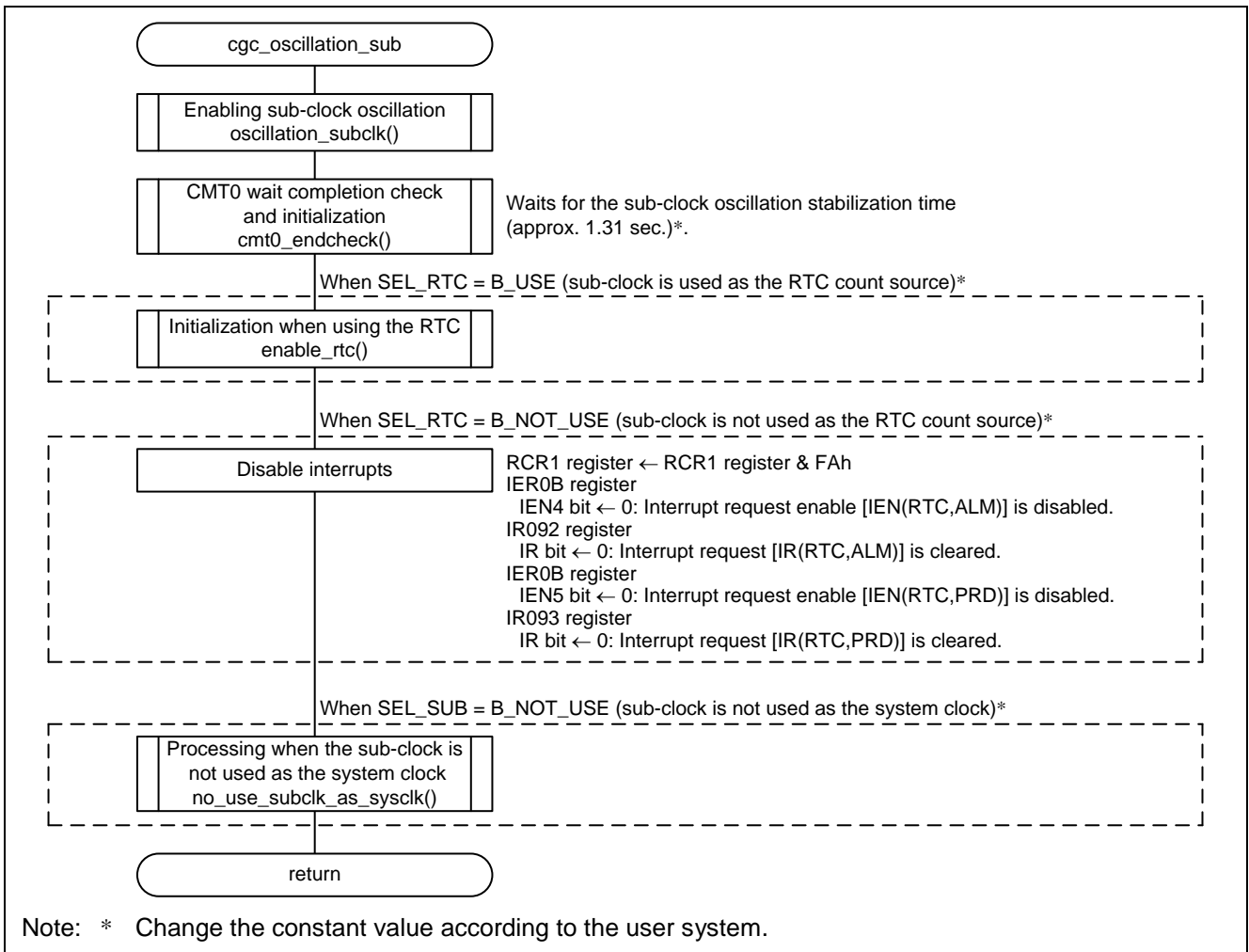
Figure 4.10 Sub-Clock Oscillation Setting
