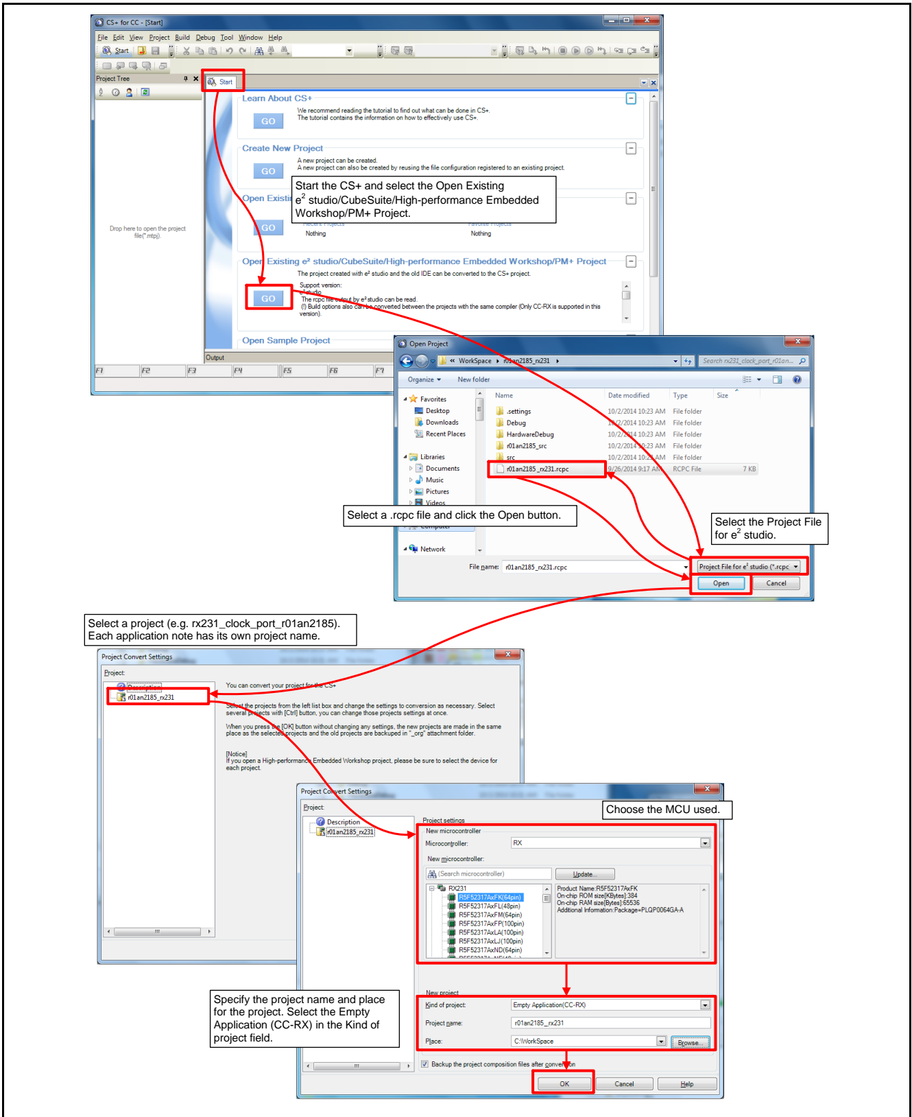
Figure 5.2 Importing a Project in CS+
