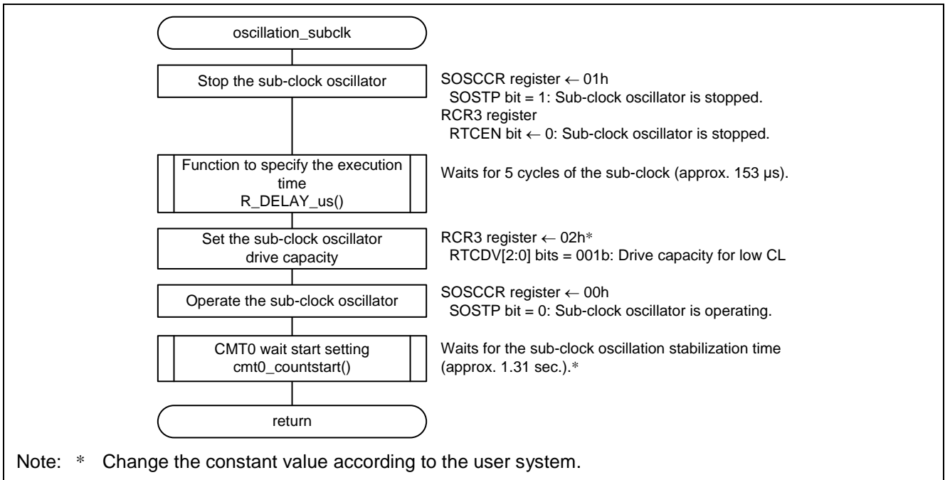
Figure 4.11 Enabling Sub-Clock Oscillation
