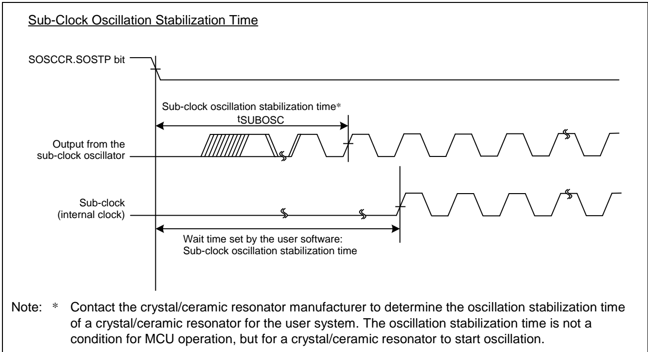
Figure 4.1 Sub-Clock Oscillation Stabilization Time
