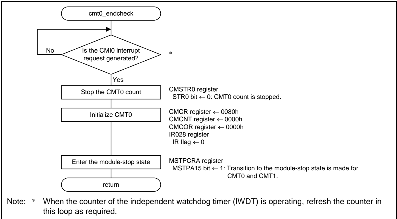
Figure 4.16 CMT0 Wait Completion Check and Initialization
