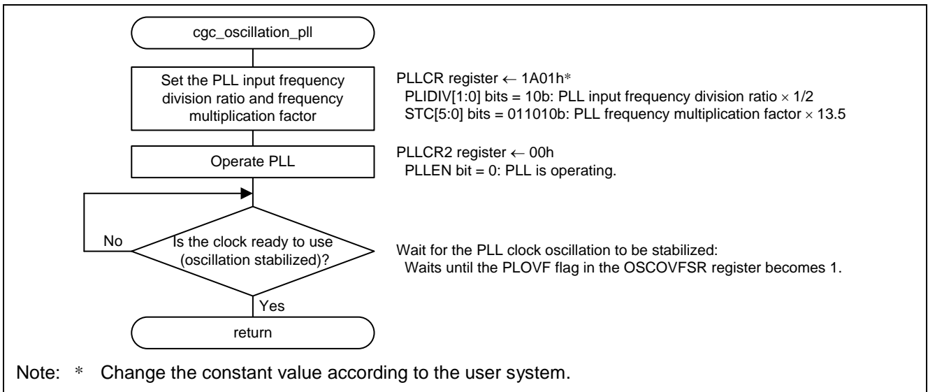
Figure 4.9 PLL Clock Oscillation Setting
