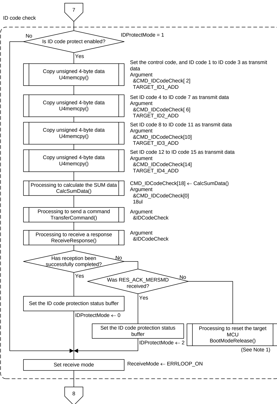
Figure 5.24 Main Processing and Communication Protocol Control
