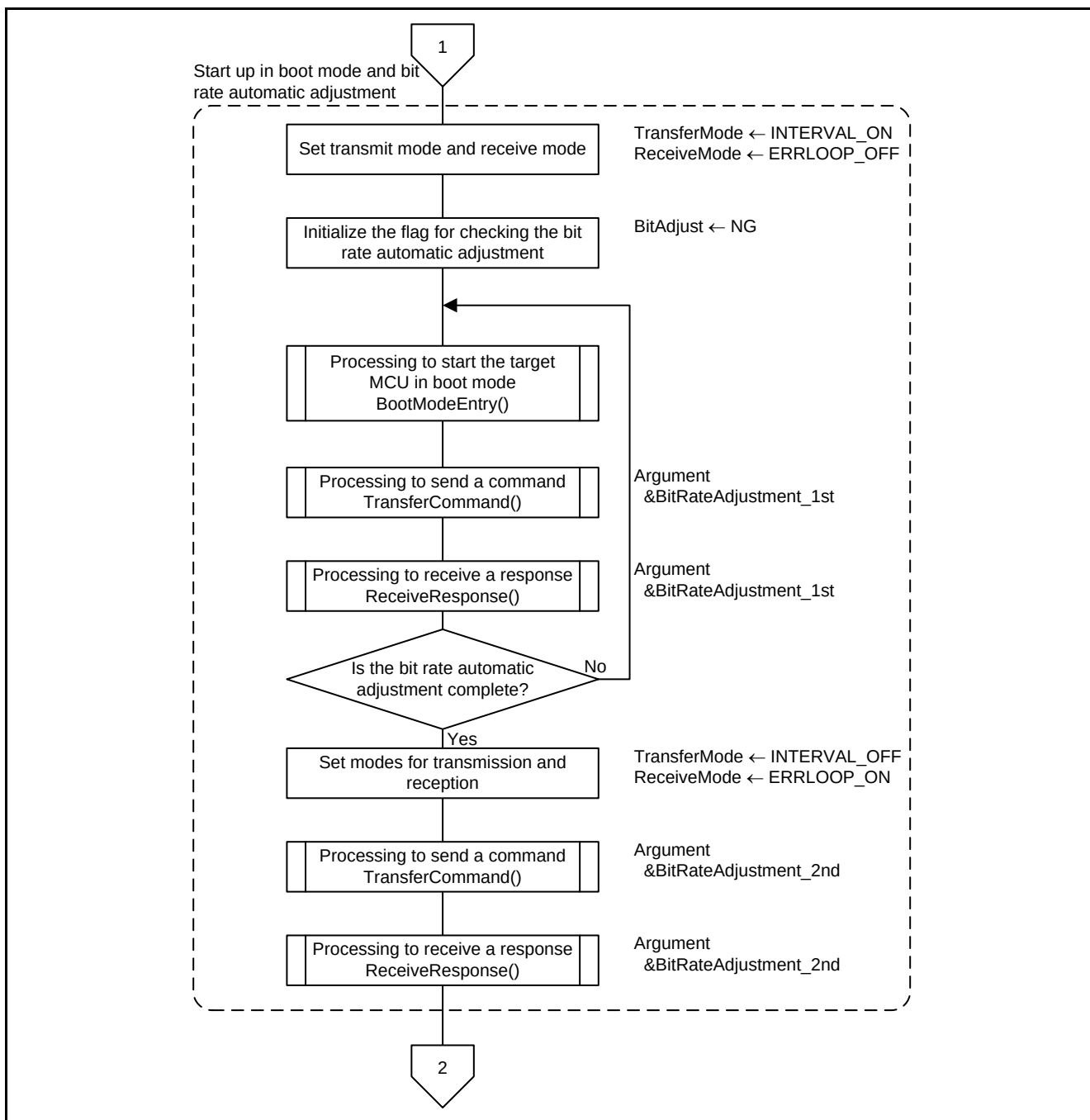
Figure 5.18 Main Processing and Communication Protocol Control
