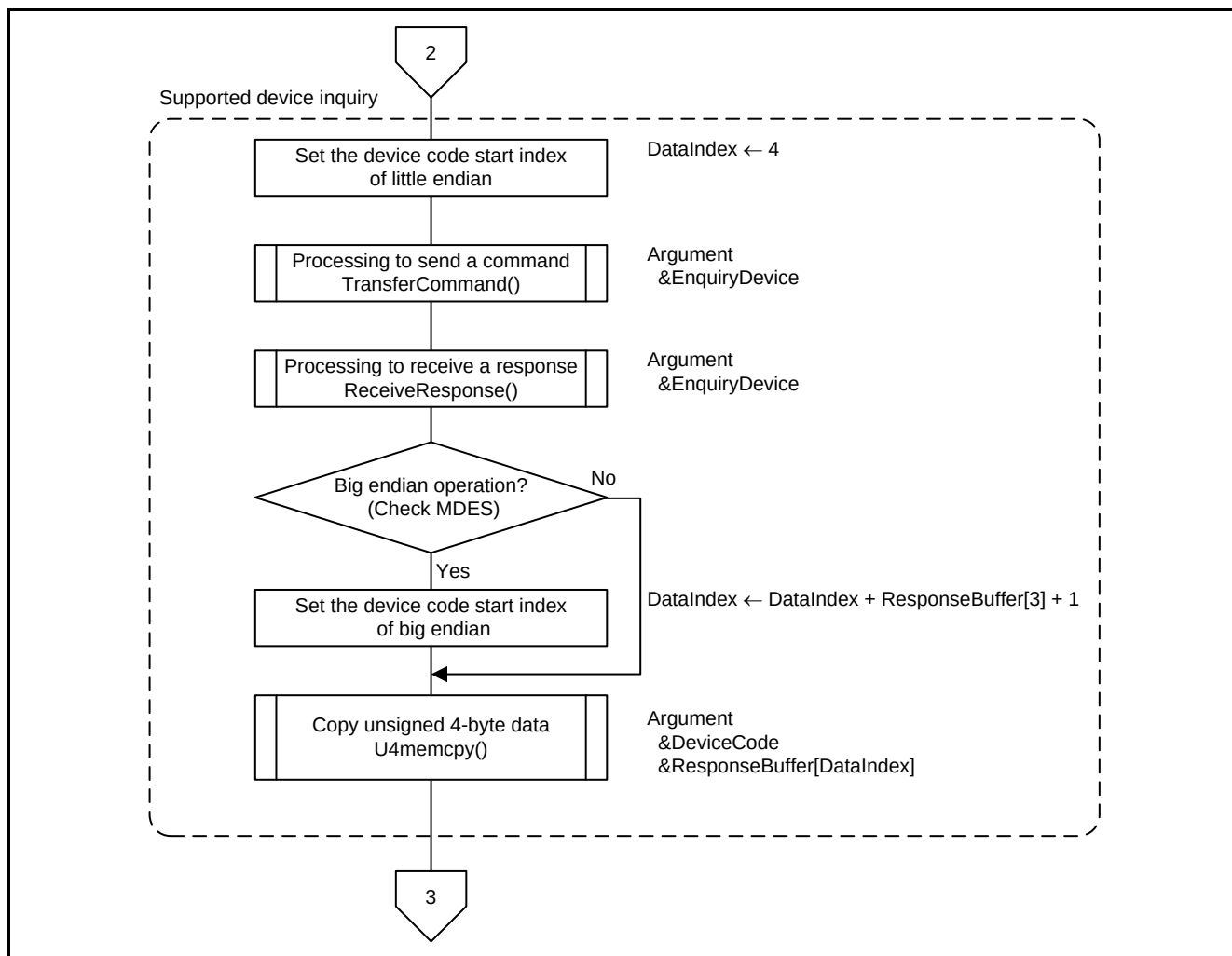
Figure 5.19 Main Processing and Communication Protocol Control
