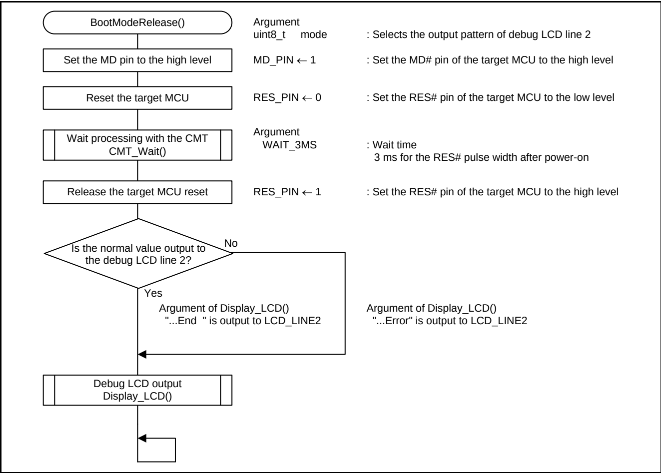
Figure 5.40 Processing to Reset the Target MCU
