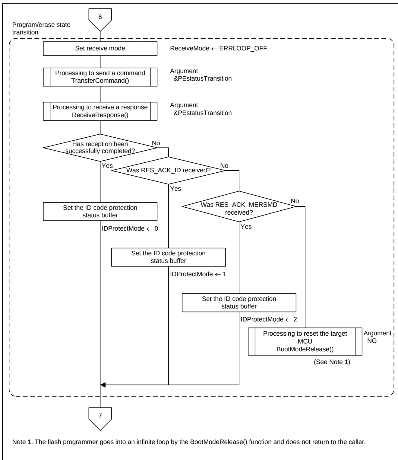
Figure 5.23 Main Processing and Communication Protocol Control
