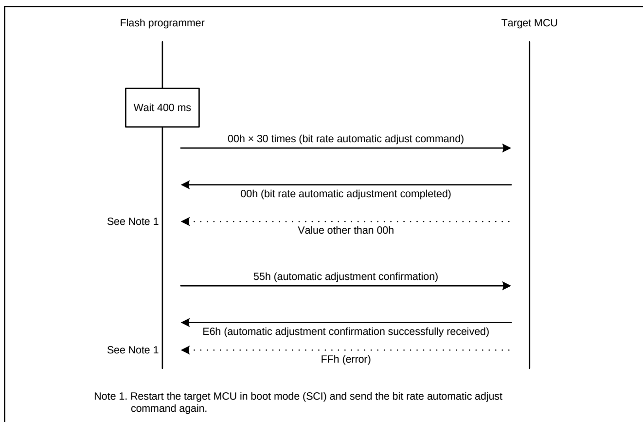
Figure 5.4 Bit Rate Automatic Adjustment Procedure
