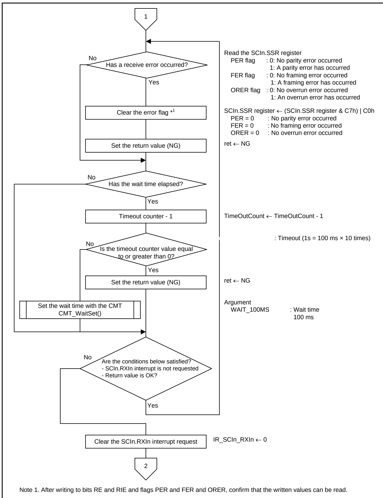
Figure 5.43 Processing to Receive a Command
