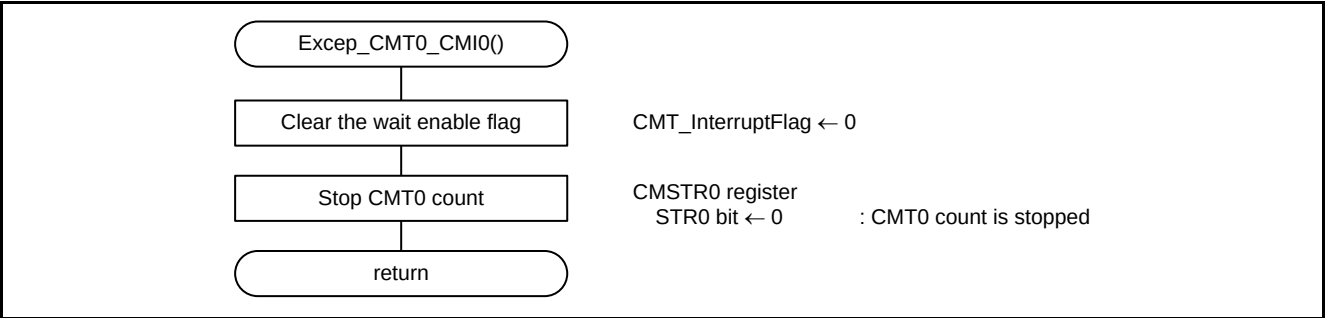
Figure 5.35 Interrupt Handling for CMI0 in CMT0
